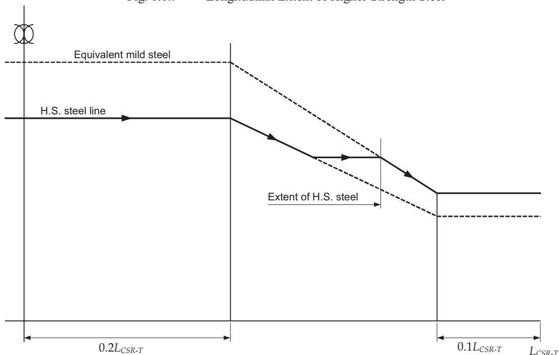
Fig. 8.1.9 Longitudinal Extent of Higher Strength Steel
