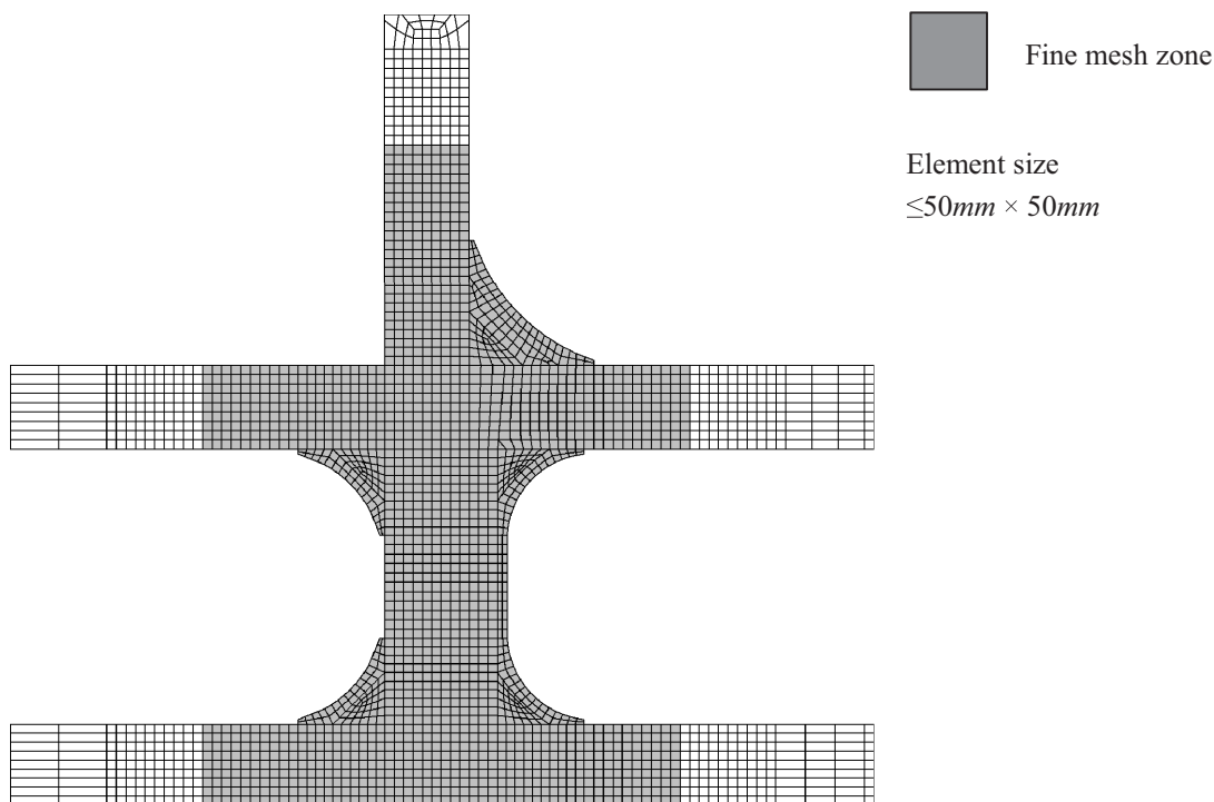
Fig. B.3.13 (Continued)
