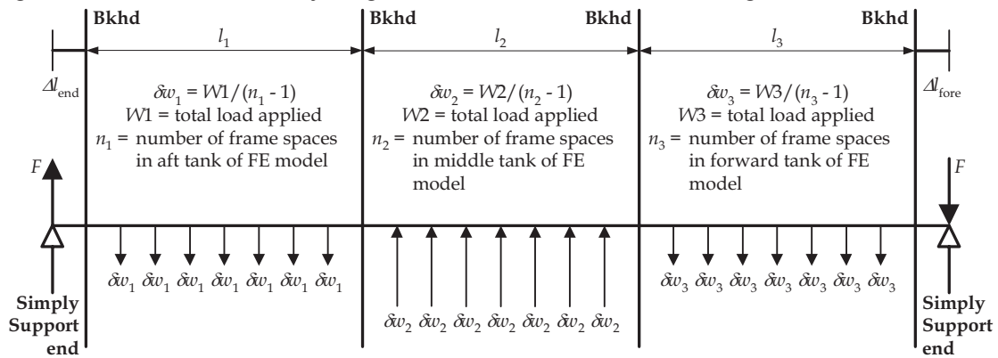
Fig. B.2.11 Distribution of Adjusting Vertical Force at Frames and Resulting Shear Force Distributions
