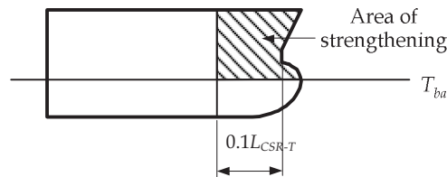
Fig. 8.6.6 Extent of Strengthening Against Bow Impact
