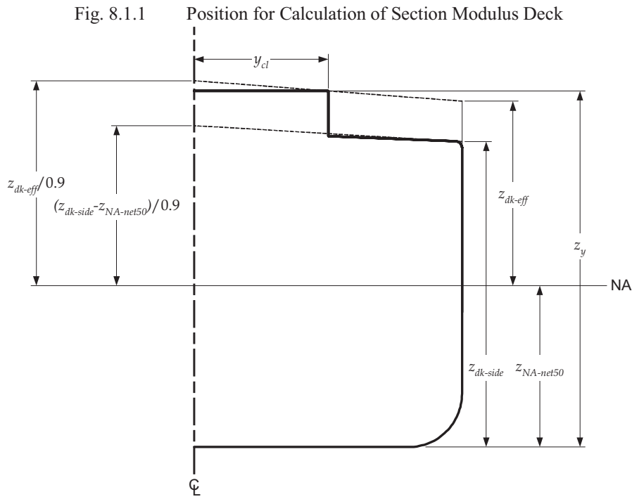
(a) Trunk deck or continuous hatch coaming
