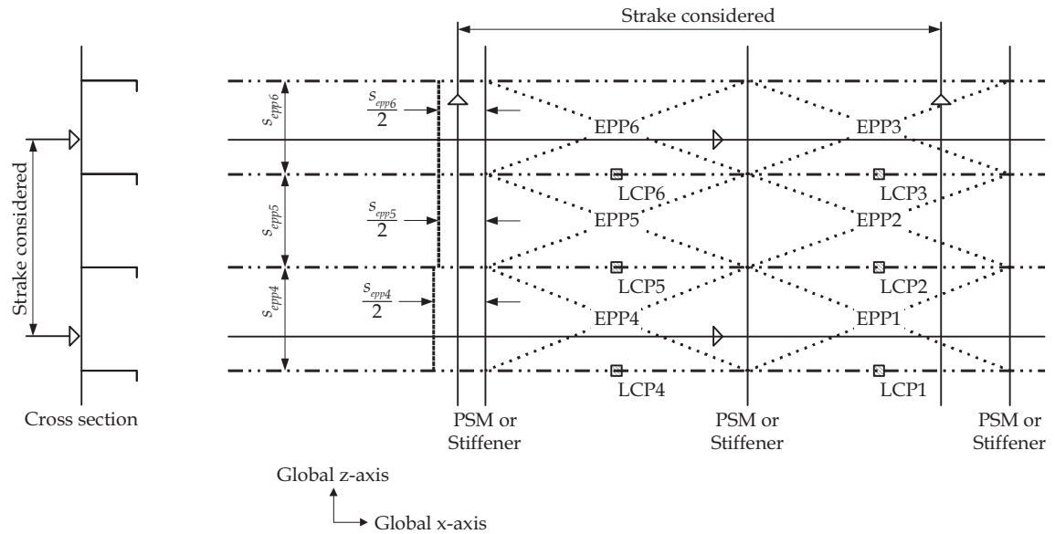
(b) Transverse Framing
