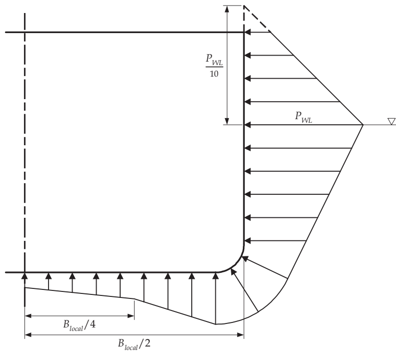
Fig. 7.3.6 Transverse Distribution of Minimum Dynamic Wave Pressure for Scantling Requirements and Strength Assessment
