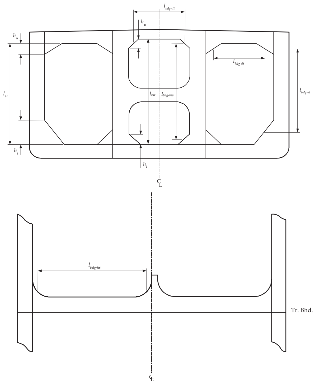
Fig. 8.2.7 (Continued) Definition of Spans of Deck, Side Transverses, Vertical Web Frames on Longitudinal Bulkheads and Horizontal Stringers on Transverse Bulkheads
