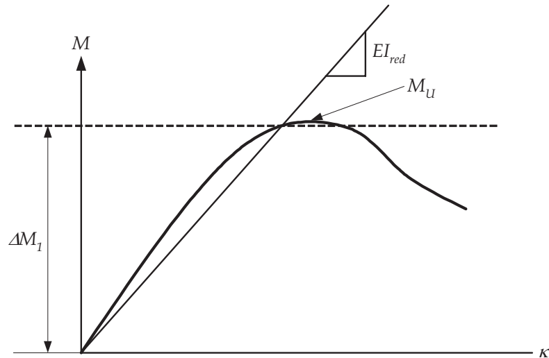
Fig. A.2.1 Moment – Curvature of Hull Girder Single Step Procedure
