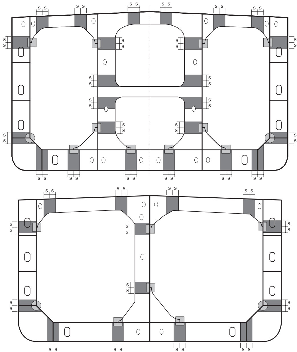
Fig. B.3.1 (Continued) Areas Requiring Consideration for Fine Mesh Analysis on a Typical Transverse Web Frame, Wash Bulkhead and Web Frame adjacent to Transverse Bulkhead
