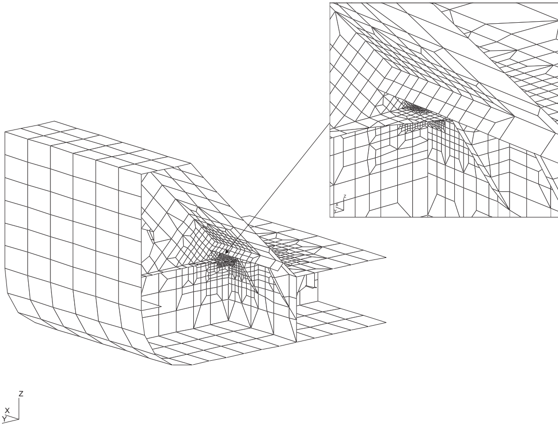
Fig. B.4.4 Typical Local Finite Element Model of Hopper Knuckle Connection t_{net50} \times t_{net50} Mesh on Hopper Plate, Web Frame, Girder and Bracket in way
