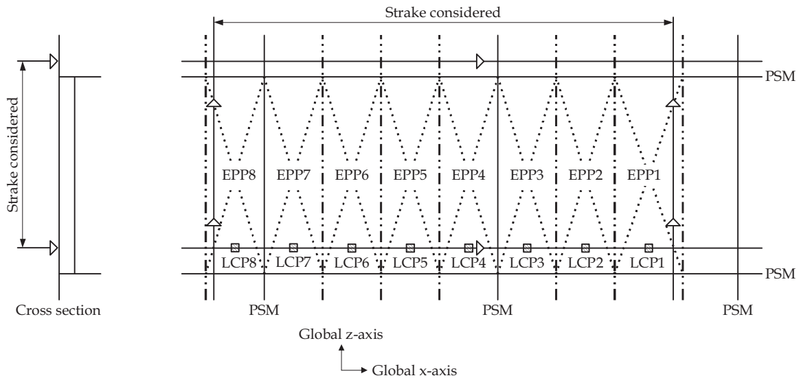
(b) Transverse Framing
