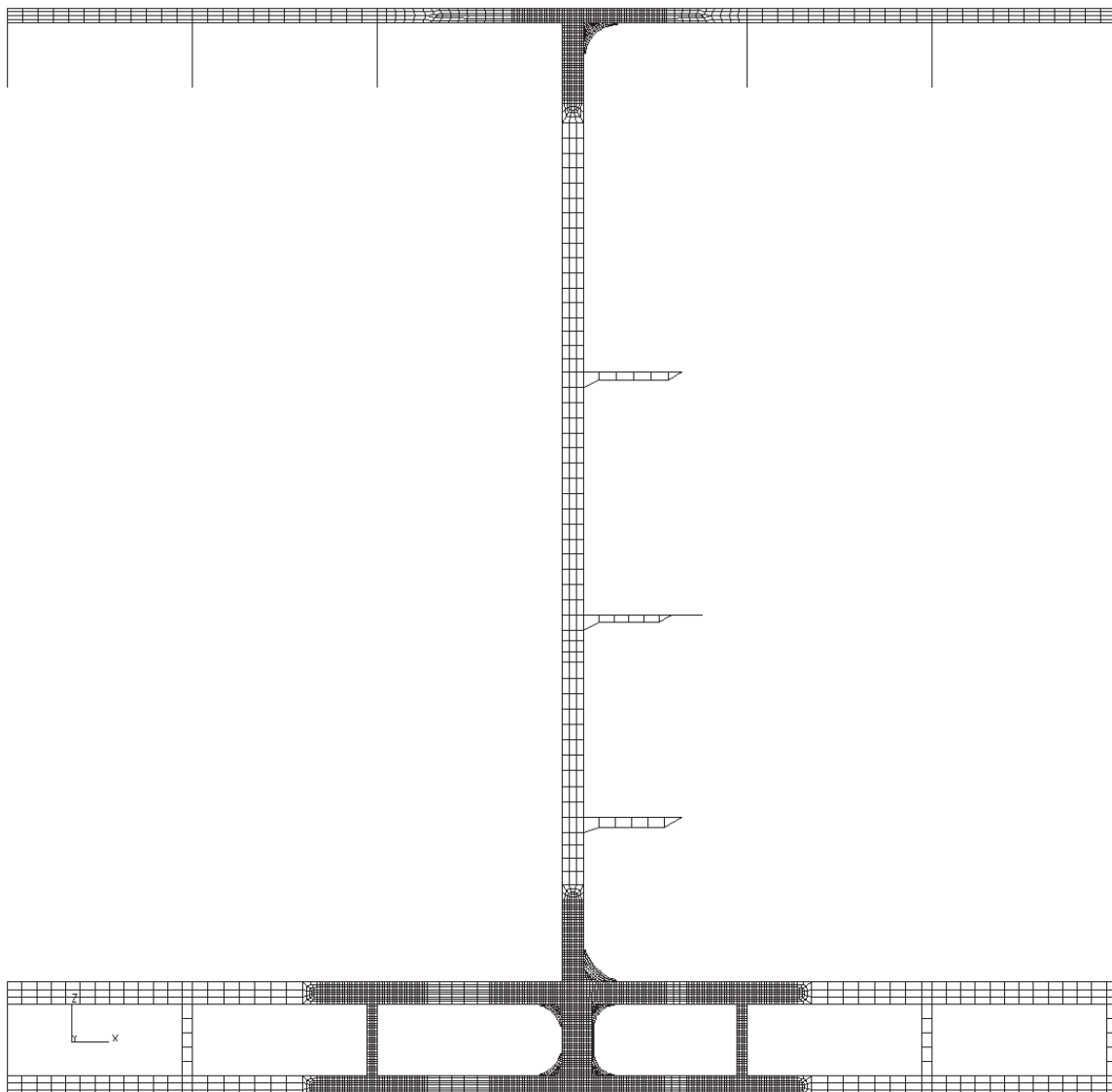
Fig. B.3.13 Sub-Model for Fine Mesh Analysis of End Connections and Web Stiffeners of Deck and Double Bottom Longitudinals
