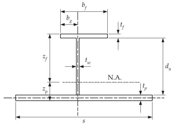
Fig. C.1.7 Stiffener Geometry
