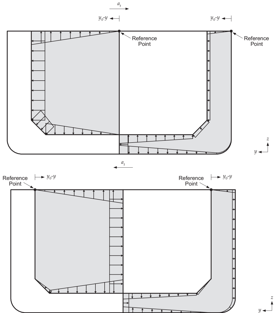
Fig. 7.6.5 Dynamic Tank Pressure in Cargo Tank (Left) and Ballast Tank (Right) due to Negative and Positive Transverse Tank Acceleration
