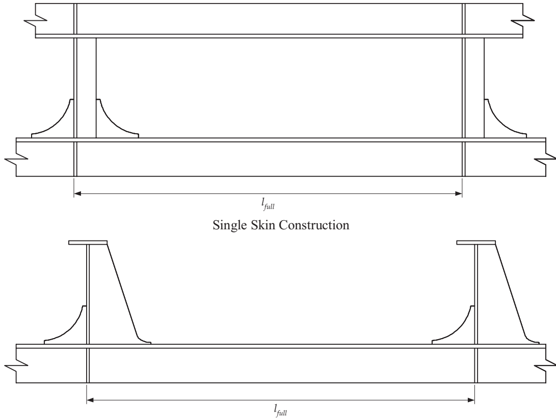
Fig. 3.5.4 Definition of Overall Span of Stiffeners, l_{full} Double Skin Construction
