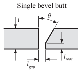
Fig. 6.5.1 Typical Butt Welds
