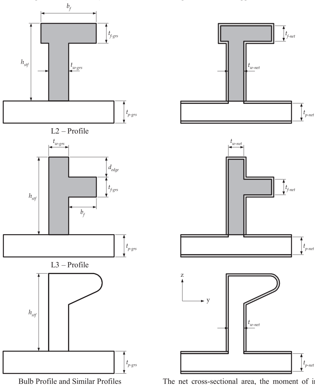
Fig. 4.2.12 (Continued) Net Sectional Properties of Local Support Members
