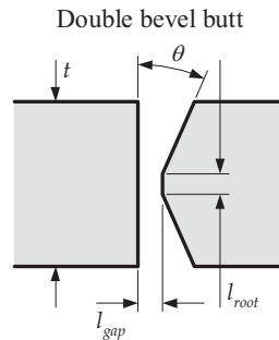
Double vee butt, uniform bevels
