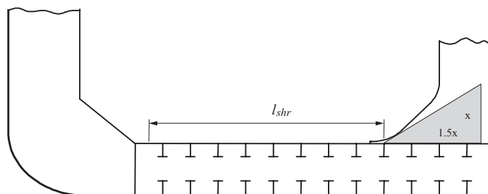
Typical arrangement with hopper and end bracket
