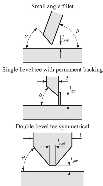
Fig. 6.5.3 Other Typical Tee and Cross Joint Welds
