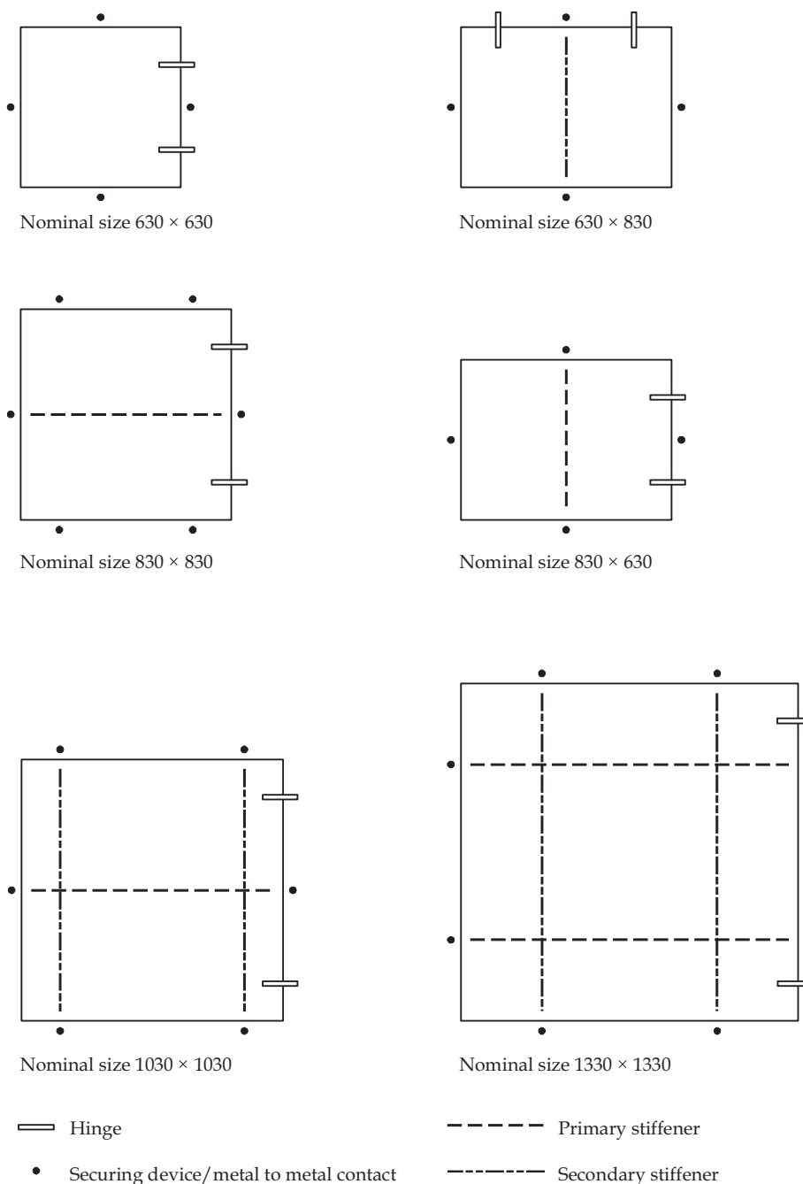
Fig. 11.1.1 Arrangement of Stiffeners
