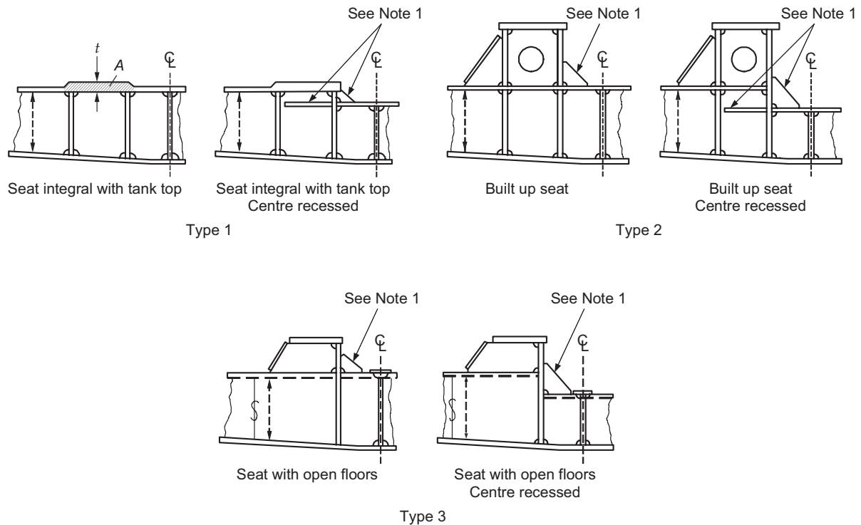
Fig. 8.4.1 Machinery Foundations
