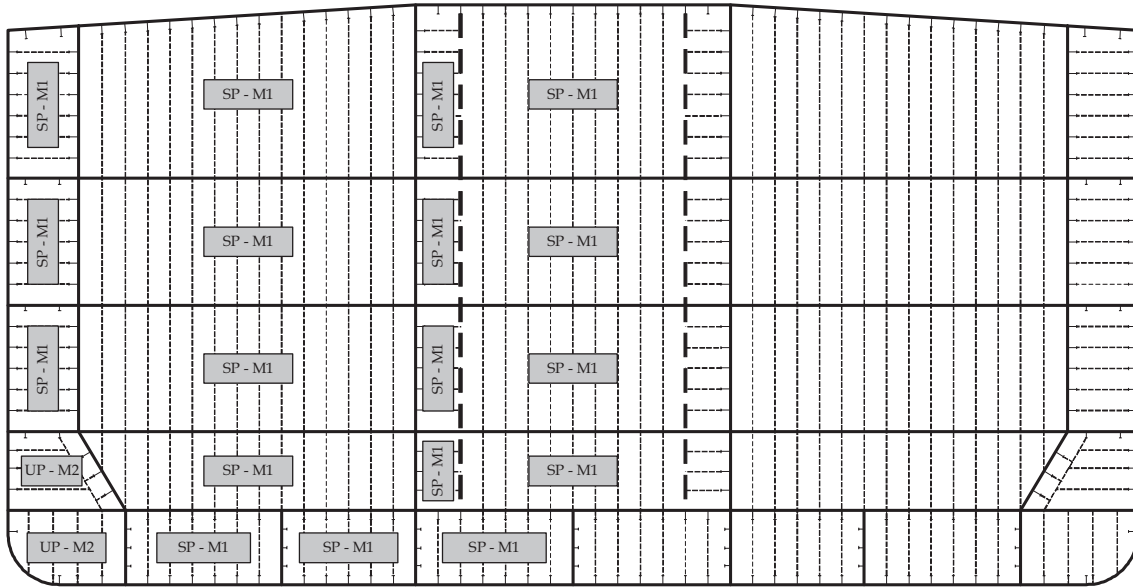
Fig. D.5.3 Transverse Bulkhead
