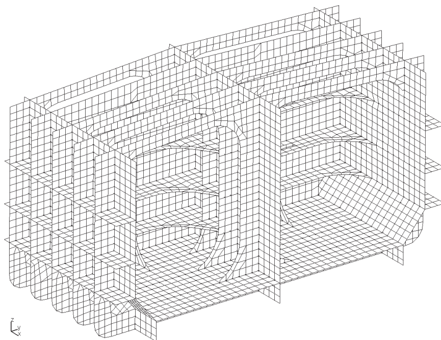
Aframax Oil Tanker
