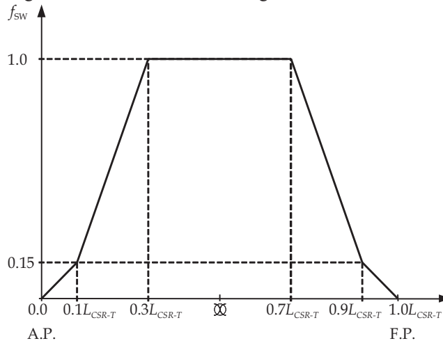
Fig. 7.2.1 Still Water Bending Moment Distribution
