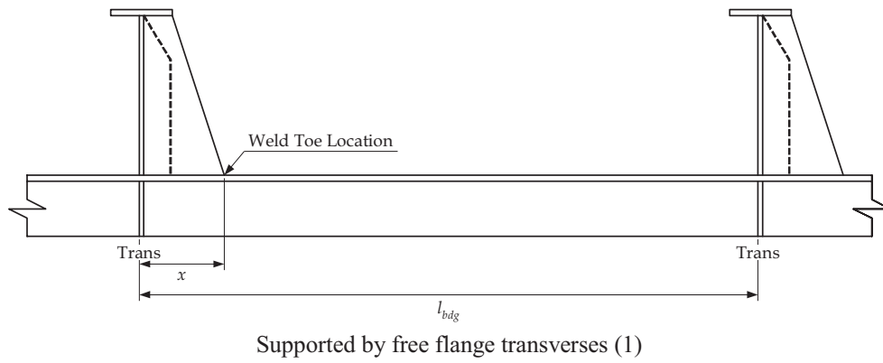
Fig. C.1.5 Definition of Effective Span Lengths
