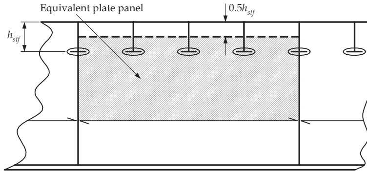
Fig. D.5.6 Capacity Model for Web Plate
