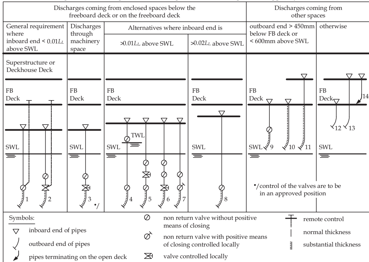
Fig. 11.1.3 Diagrammatic Arrangement of Discharge and Scupper Systems
