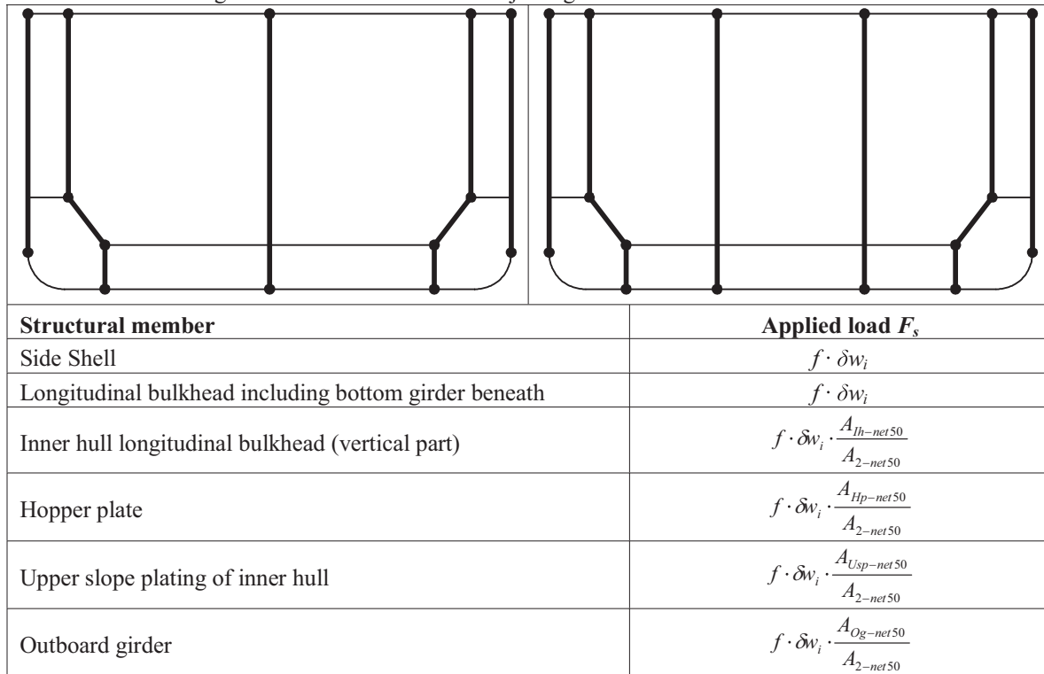
Fig. B.2.12 Distribution of Adjusting Load on a Transverse Section
