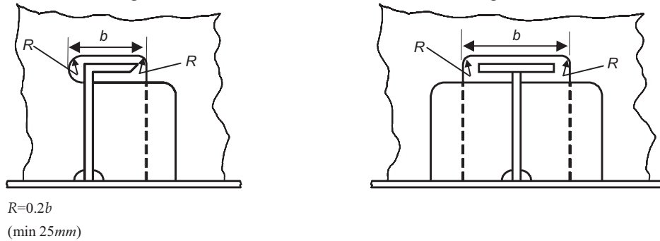
Fig. 4.3.4 Collars for Cut-outs in Areas of High Stress
