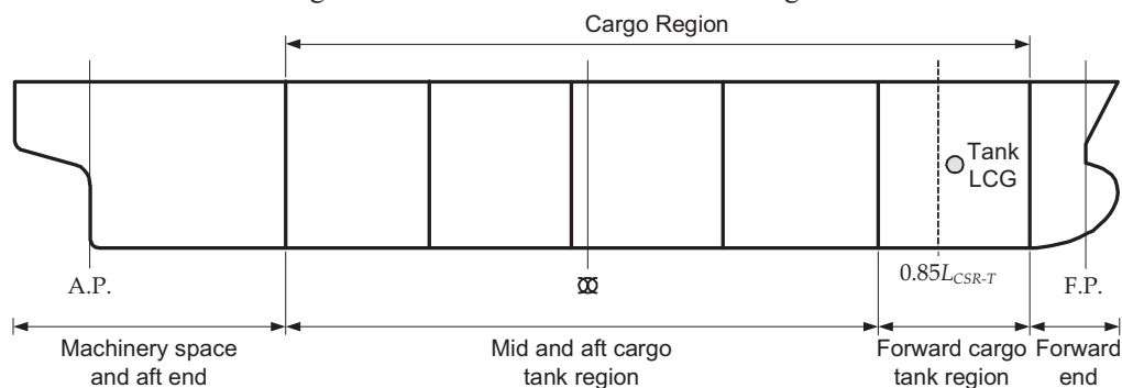
Fig. 7.6.7 Illustration of Structural Regions
