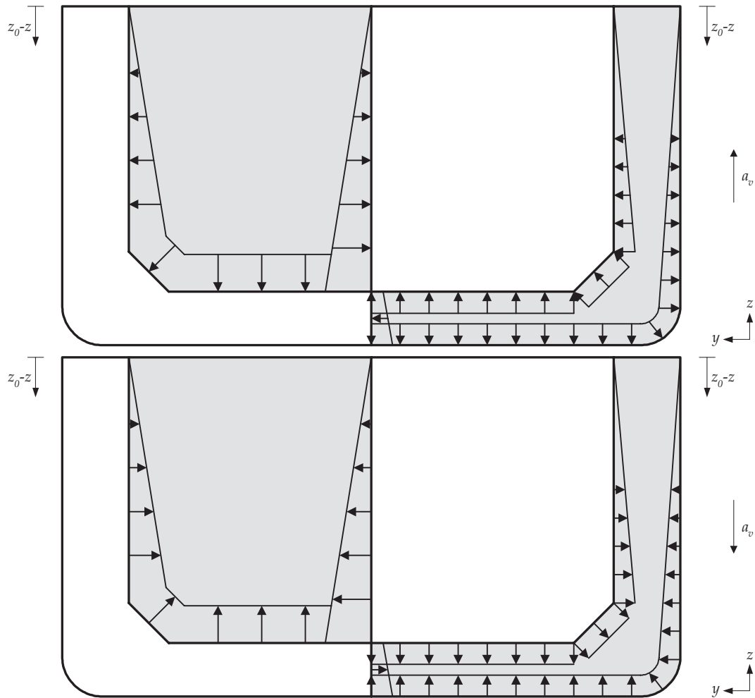
Fig. 7.6.4 Dynamic Tank Pressure in Cargo Tank (Left) and Ballast Tank (Right) due to Positive and Negative Vertical Tank Acceleration
