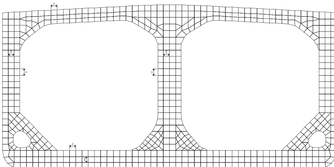
Fig. B.2.2 Typical Finite Element Mesh on Web Frame
