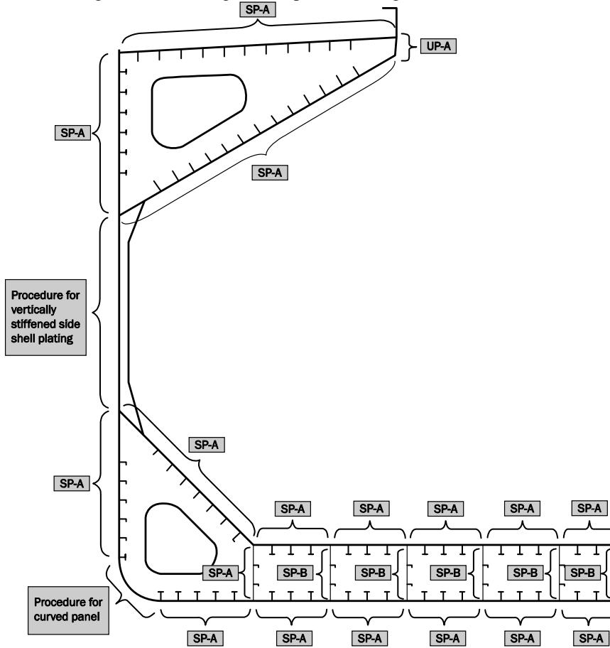
Fig. 5 Longitudinal plates for single hull bulk carrier
