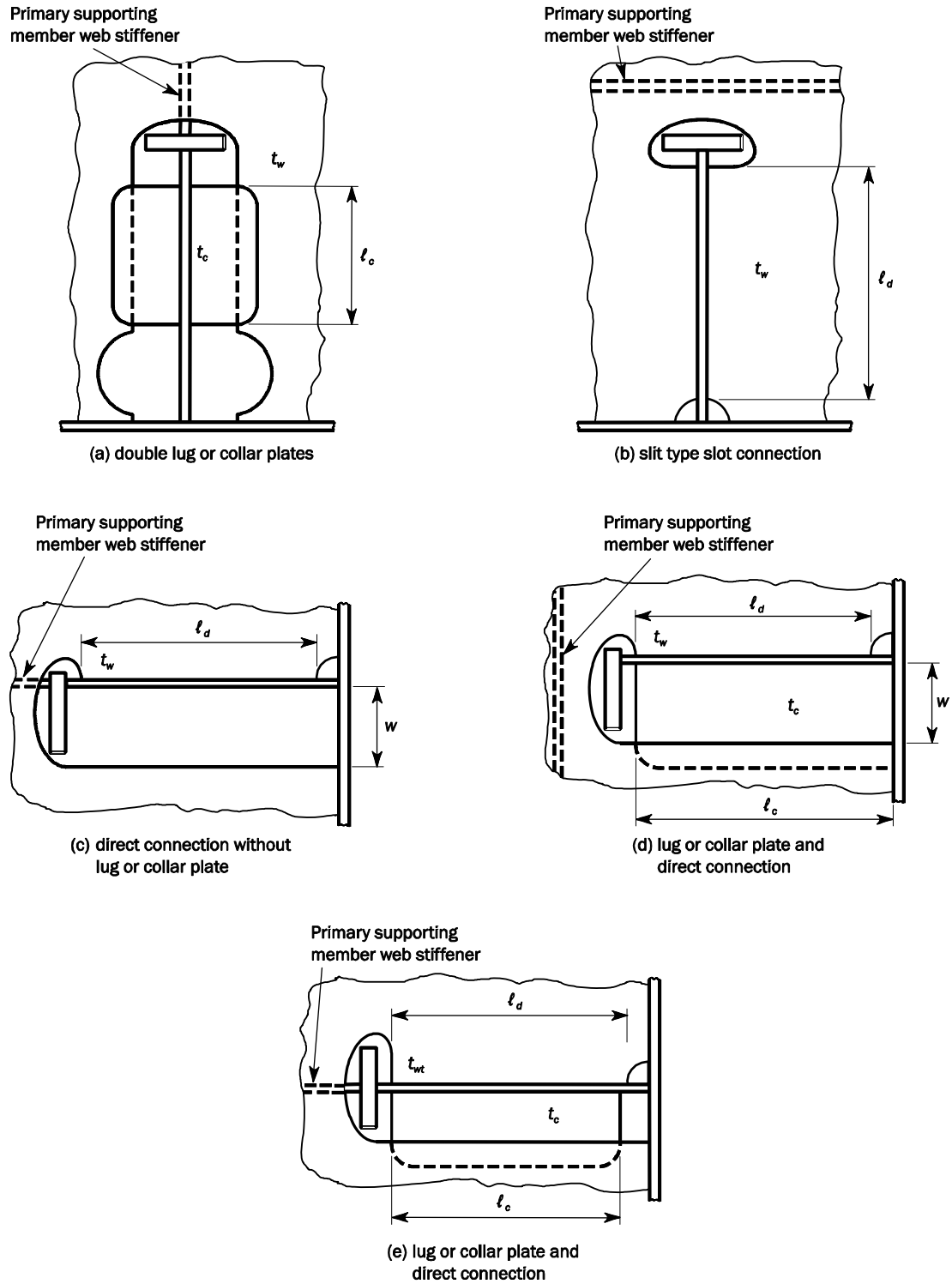
Fig. 8 Symmetric and asymmetric cut-outs
