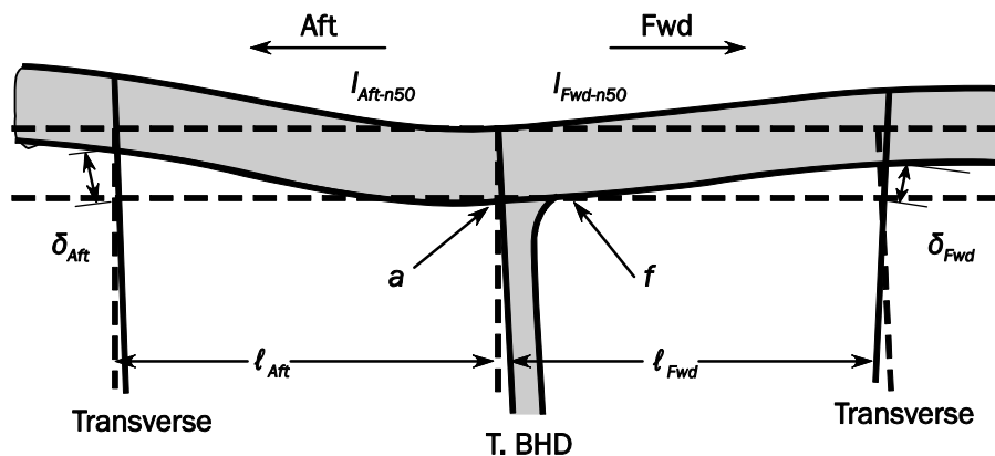
Fig. 4 Definition of the relative displacement (example of the side longitudinal)
