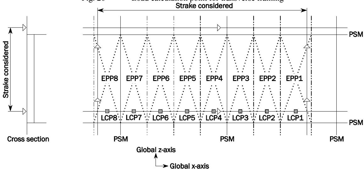
Fig. 20 Load calculation point for transverse framing
