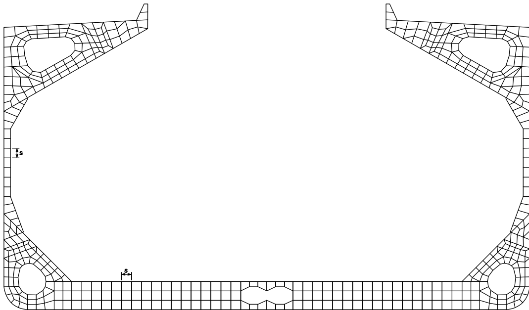
Fig. 8 Typical finite element mesh on transverse bulkhead
