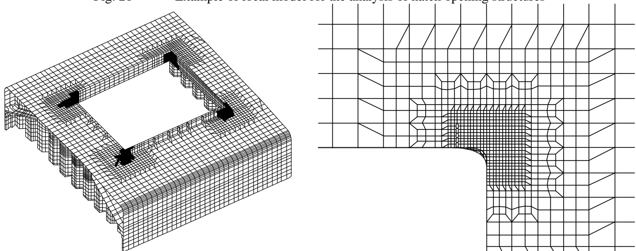
Fig. 21 Example of local model for the analysis of hatch opening structures
