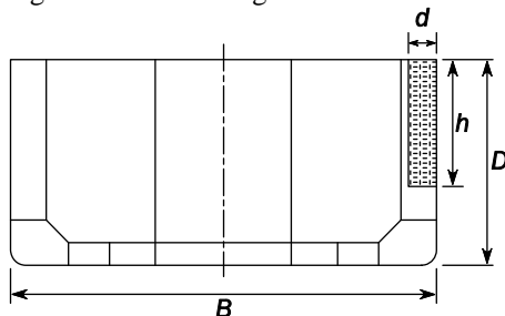
Fig. 1 Damage extent for collision
