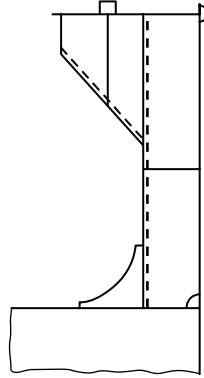
Fig. 3 Coaming stay (example 2)
