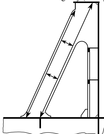
Fig. 4 Coaming stay (example 3)
