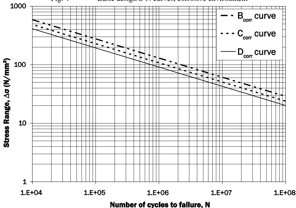
Fig. 4 Basic design S-N curves, corrosive environment
