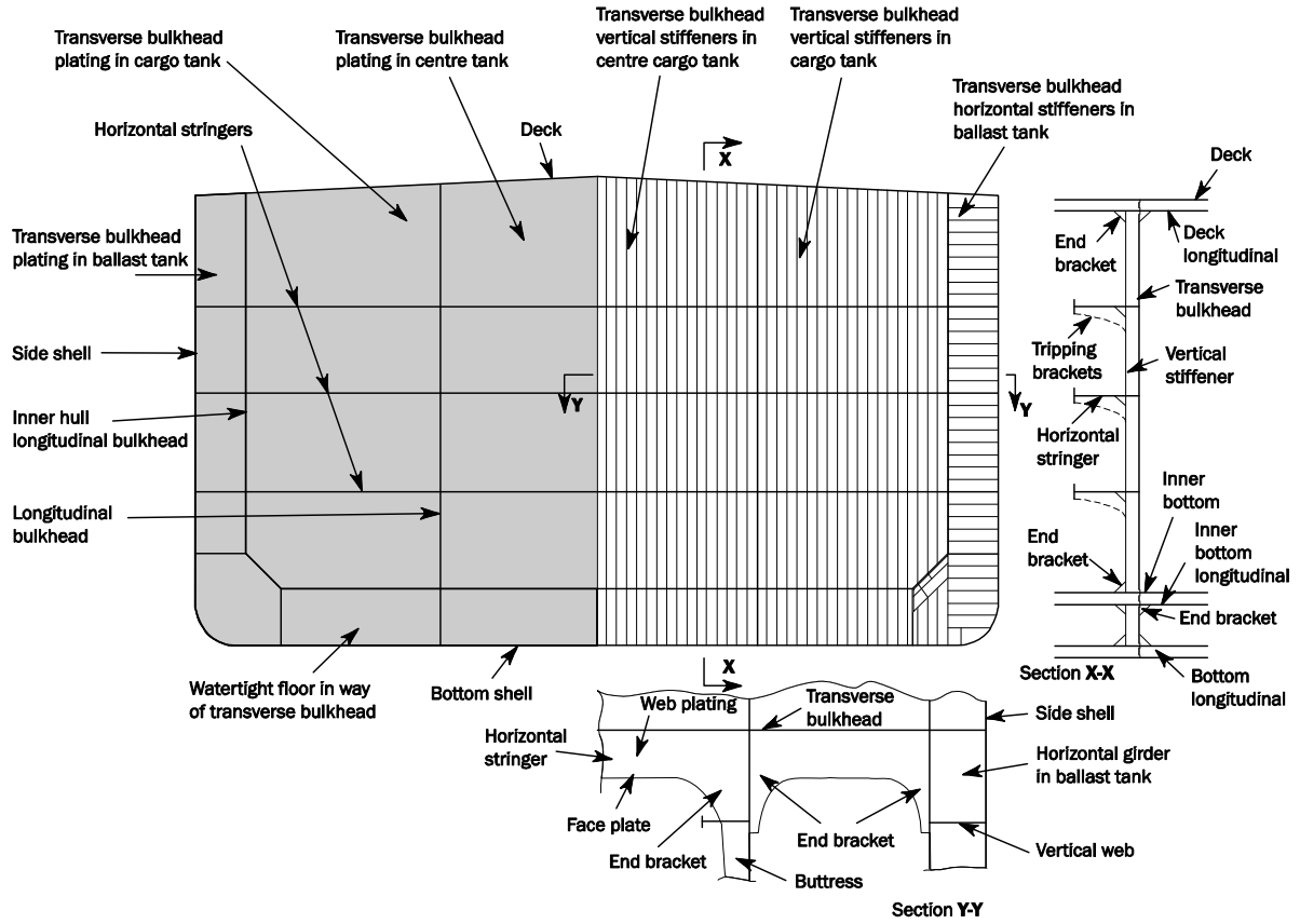
Fig. 5 Transverse bulkhead of double hull tanker
