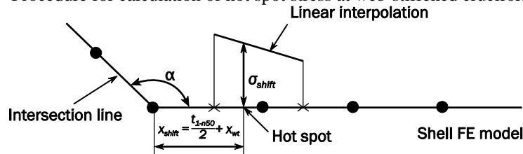
Fig. 19 Procedure for calculation of hot spot stress at web-stiffened cruciform connections
