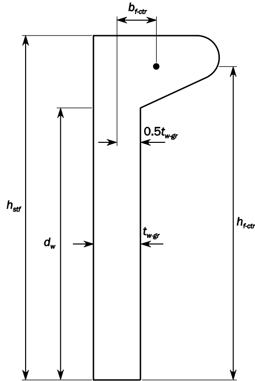
Fig. 15 Characteristic data for bulb profiles
