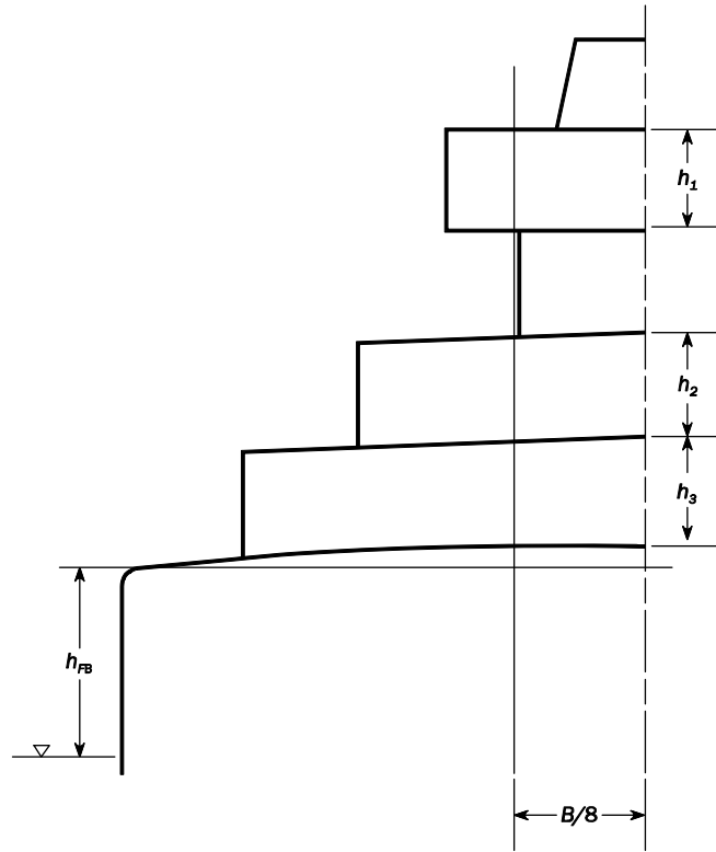
Fig. 1 Effective heights of deckhouses
