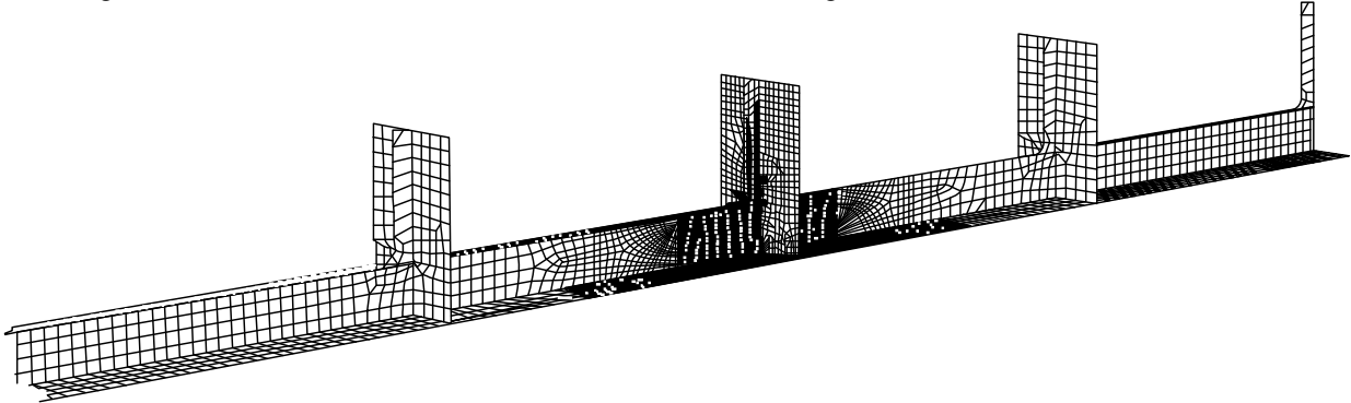
Fig. 10 Fine mesh finite element model for derivation of geometrical stress concentration factor
