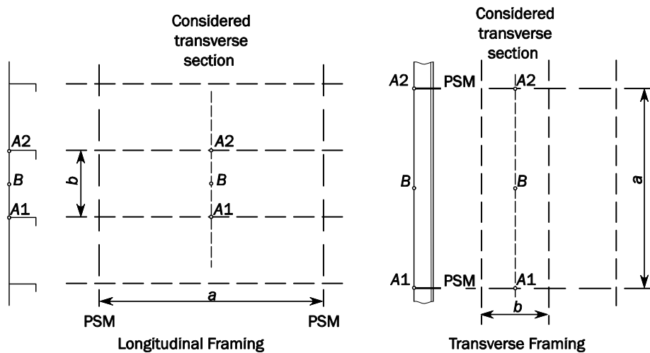
Fig. 23 LCP for plate buckling – hull girder stresses
