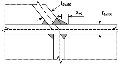
Fig. 18 Geometrical parameters of web-stiffened cruciform connections
