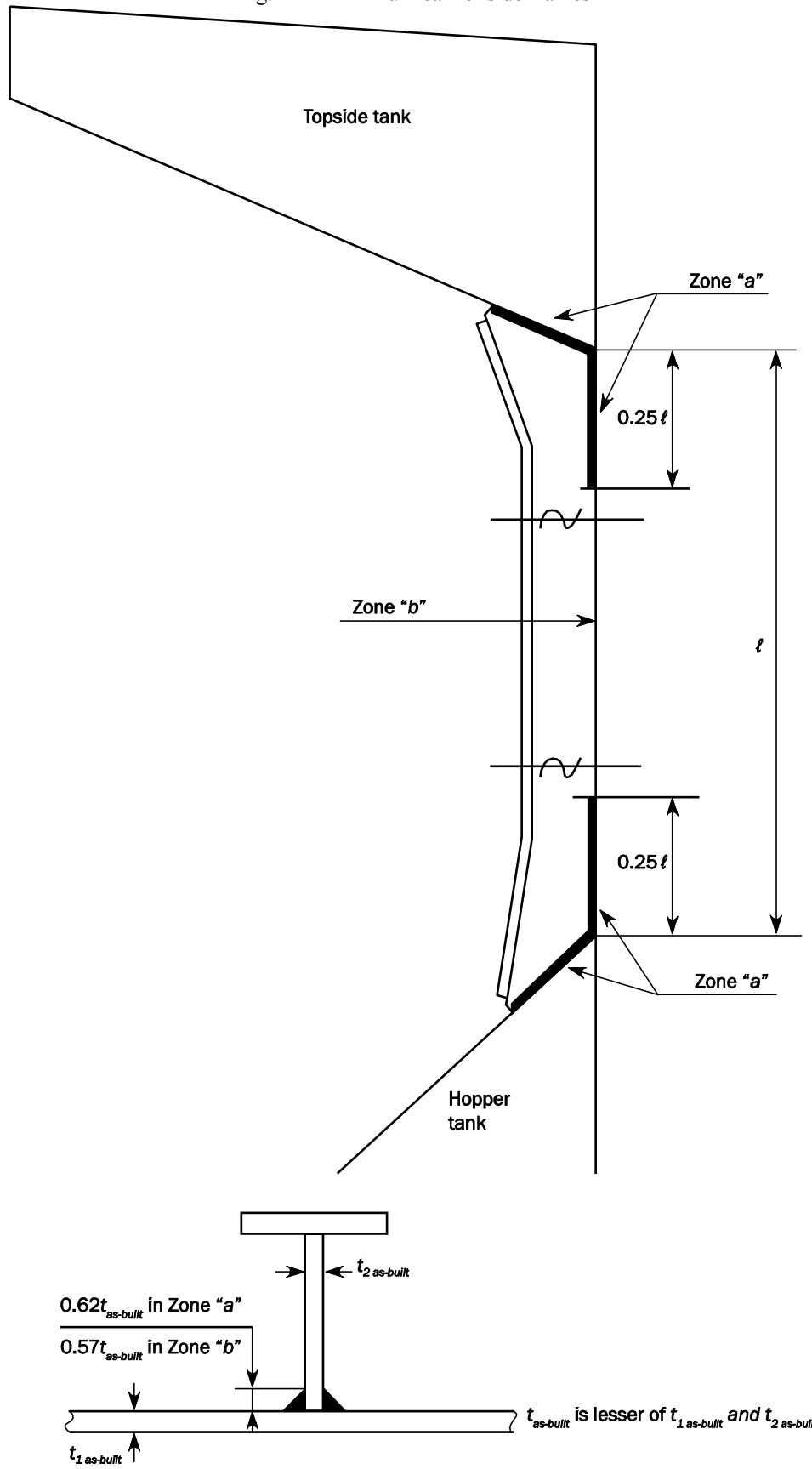
Fig. 11 Bulk carrier side frames
