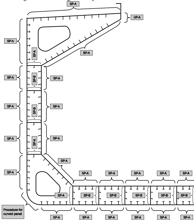
Fig. 7 Longitudinal plates for double hull bulk carrier
