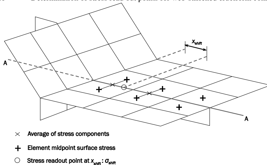
Fig. 20 Determination of stress read out points for web-stiffened cruciform connections
