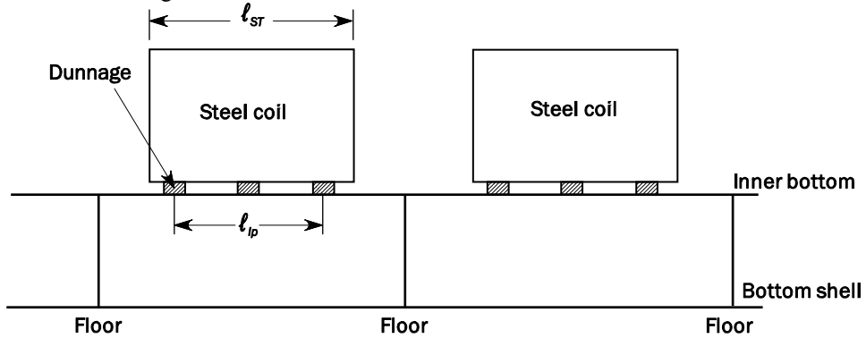
Fig. 10 Steel coils loaded between inner bottom floors
