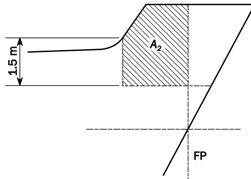
Fig. 2 Profile areas of screens and bulwarks
