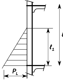
Fig. 25 Definition of pressure for vertical stiffeners
