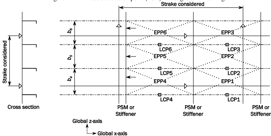
Fig. 19 Load calculation point (LCP) for longitudinal framing
