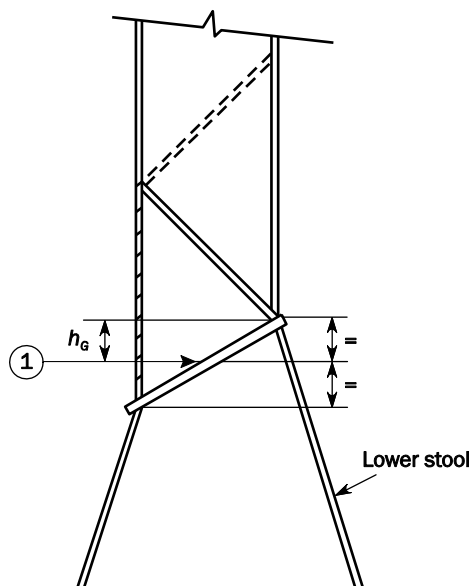
Fig. 6 Asymmetrical gusset / shedder plates
