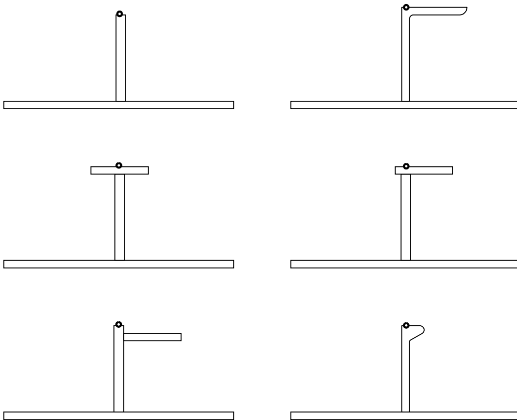
Fig. 24 Reference point for calculation of section modulus and hull girder stress for local scantling assessment
