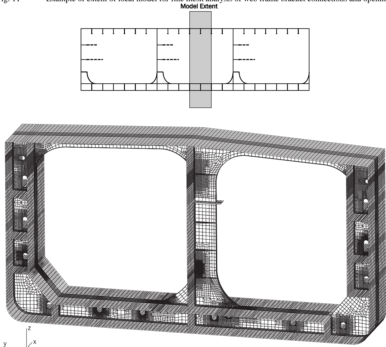
Fig. 11 Example of extent of local model for fine mesh analysis of web frame bracket connections and openings
