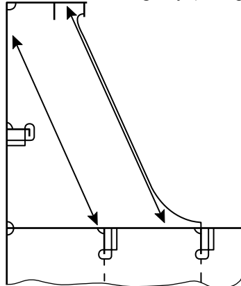
Fig. 2 Coaming stay (example 1)
