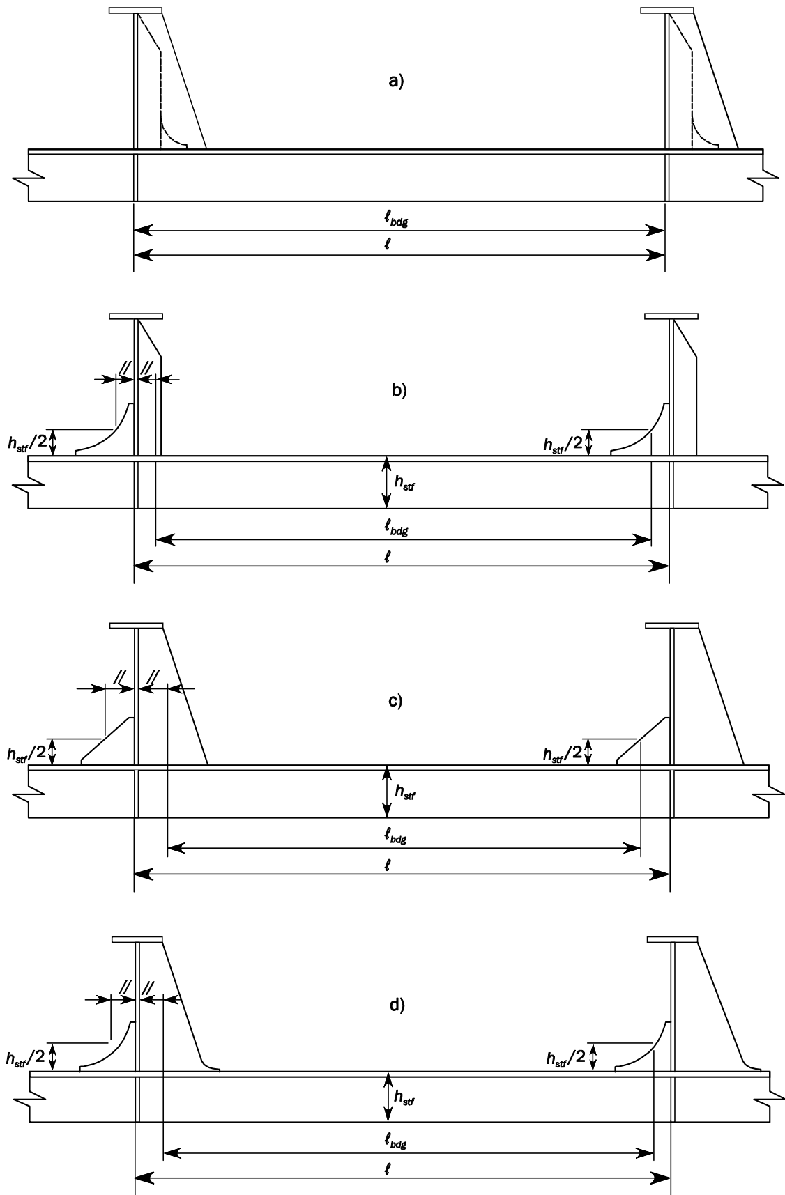
Fig. 1 Effective bending span of stiffeners supported by web stiffeners (single skin construction)
