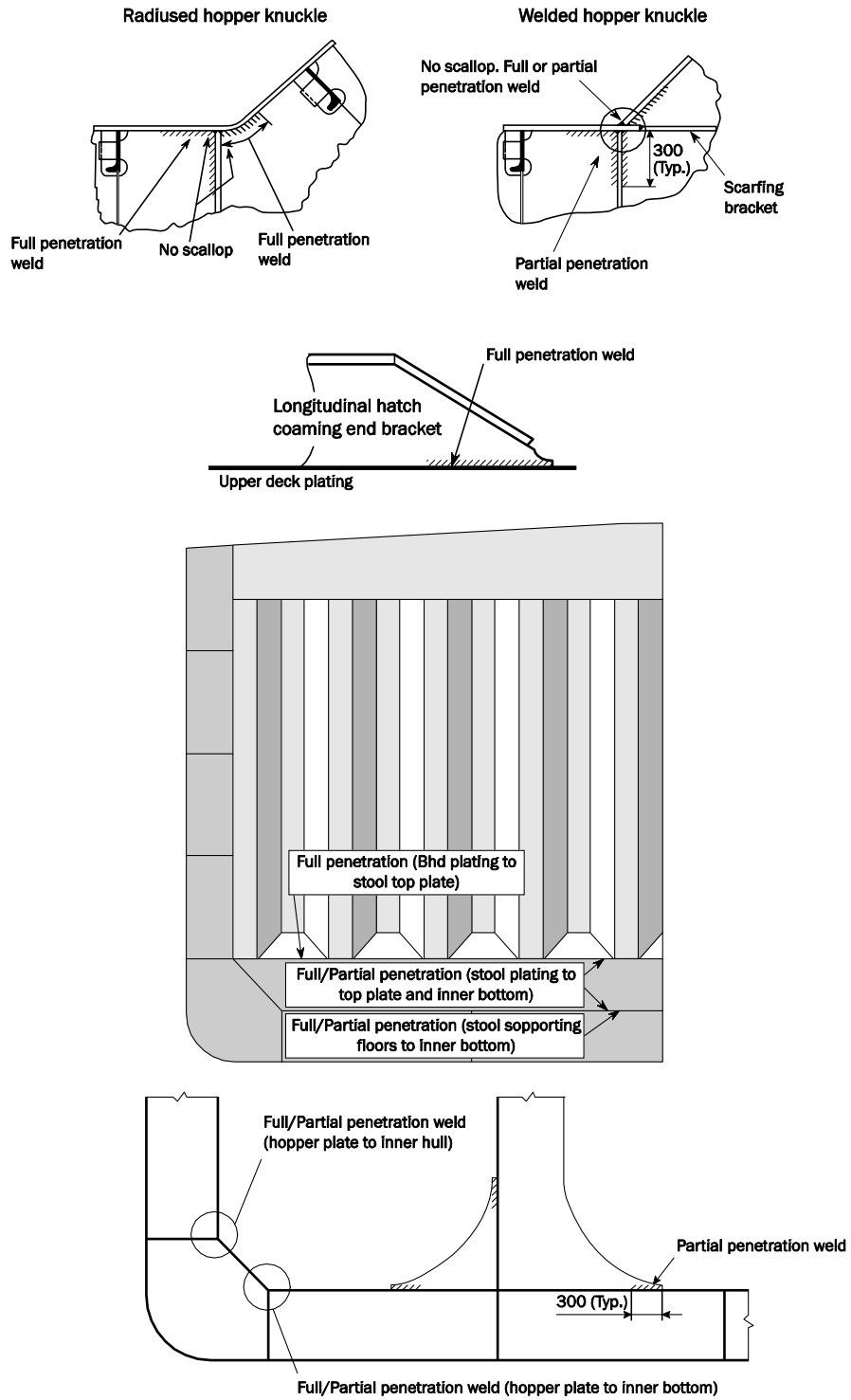
Fig. 3 High stress areas welding
