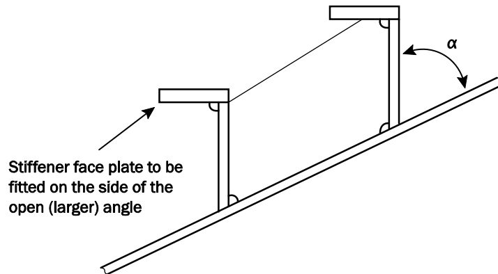
Fig. 2 Stiffener on attached plating with an angle less than 50deg
