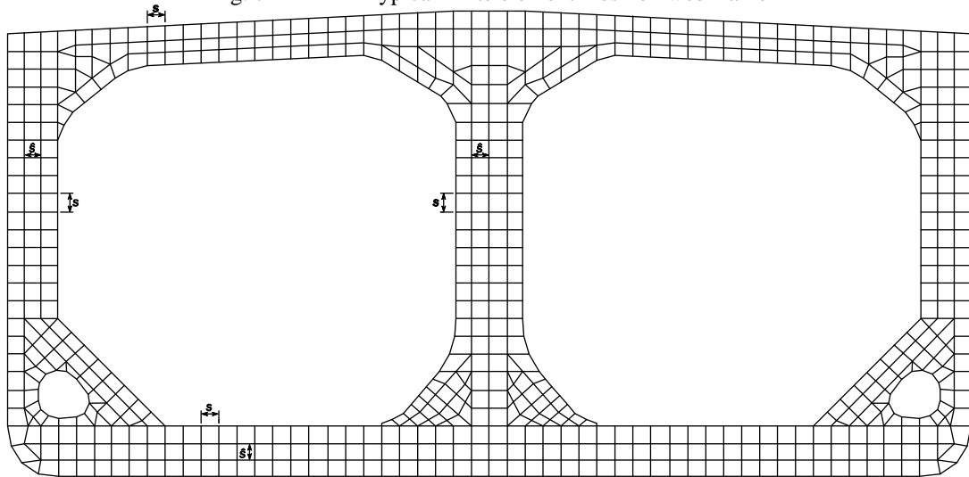
Fig. 7 Typical finite element mesh on web frame
