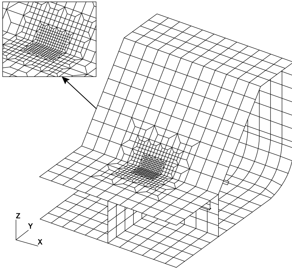
Fig. 3 Local very fine mesh model ( t_{n50} \times t_{n50} ) of hopper knuckle connection between inner bottom and hopper plate
