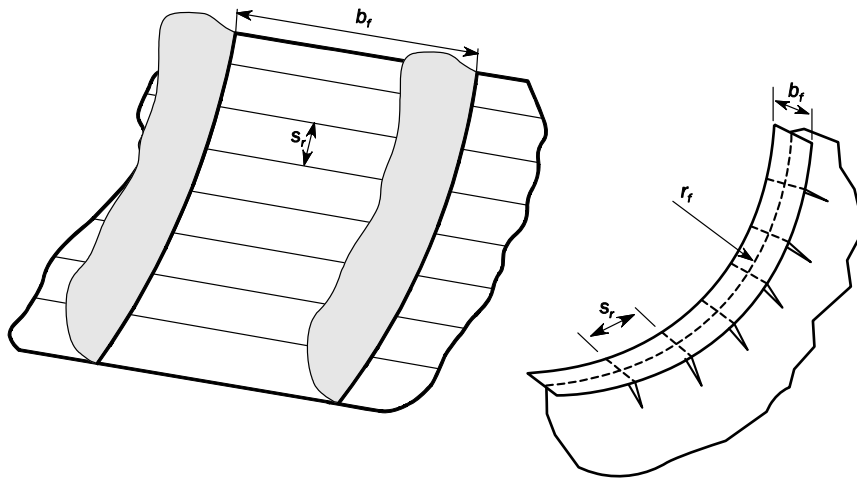
Fig. 12 Curved shell panel and face plate
