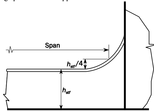
Fig. 3 Effective bending span for local support members with continuous face plate along bracket edge
