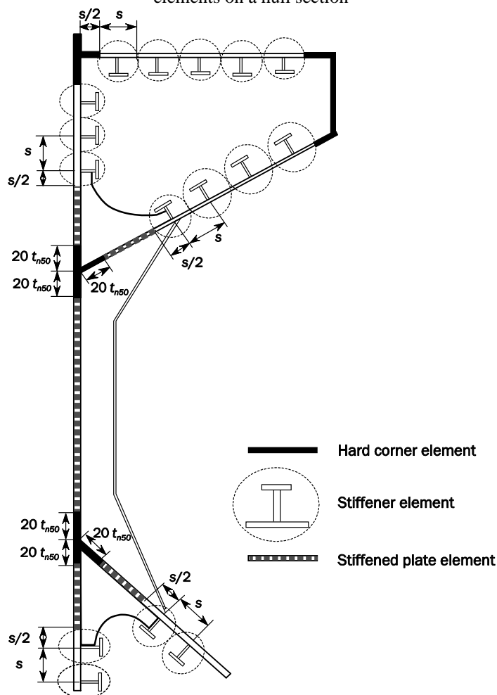
Fig.3 Examples of the configuration of stiffened plate elements, stiffener elements and hard corner elements on a hull section
