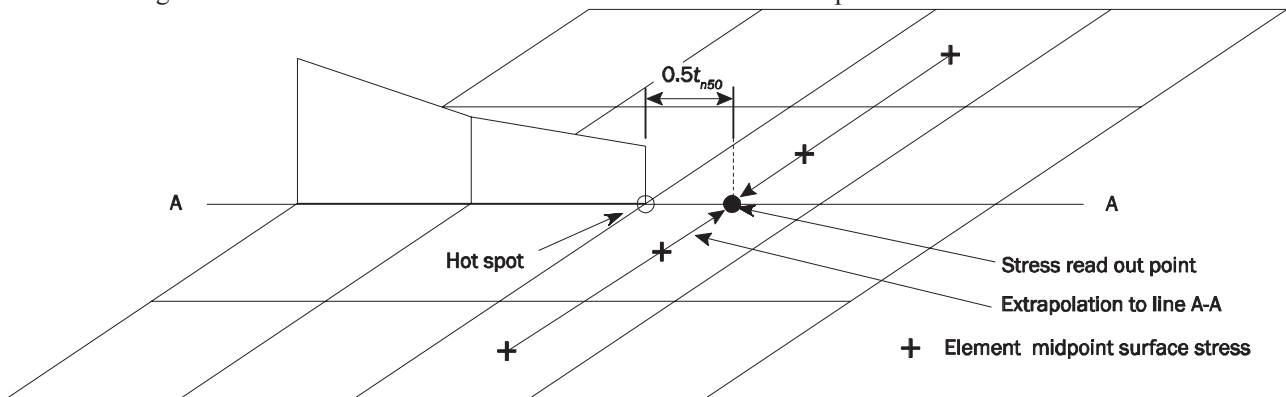
Fig. 15 Determination of Stress Read out Points and Hot Spot Stress for 4-node Element
