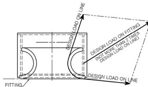
Fig. 4 Design Load on Fitting
