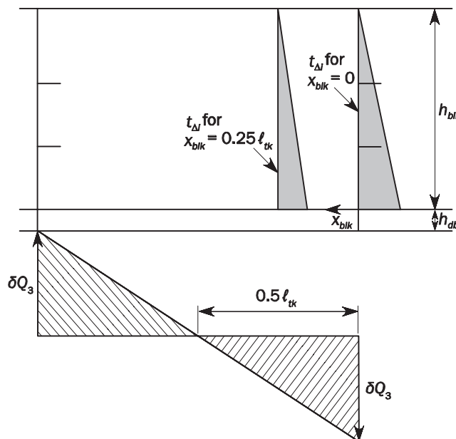
Fig. 5 Shear Force Correction for Longitudinal Bulkheads
