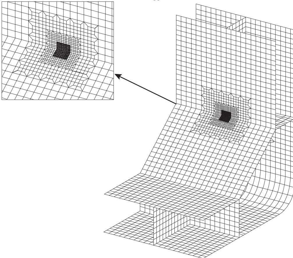
Fig. 5 Local Very Fine Mesh Model ( t_{n50} \times t_{n50} ) of Upper Hopper Knuckle Connection between Inner Side Shell and Hopper Plate
