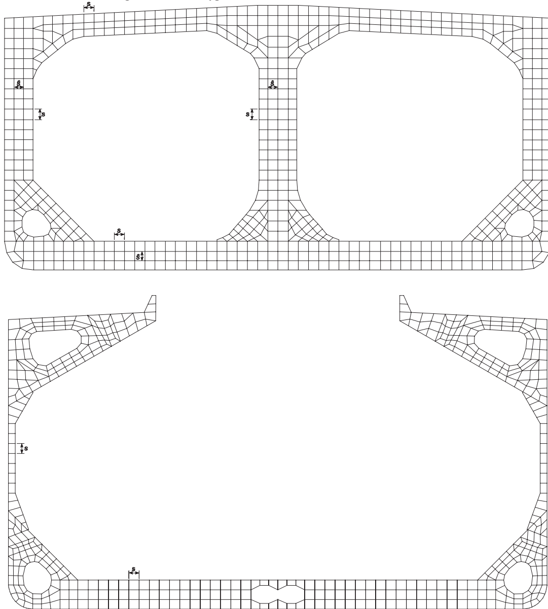
Fig. 7 Typical Finite Element Mesh on Web Frame
