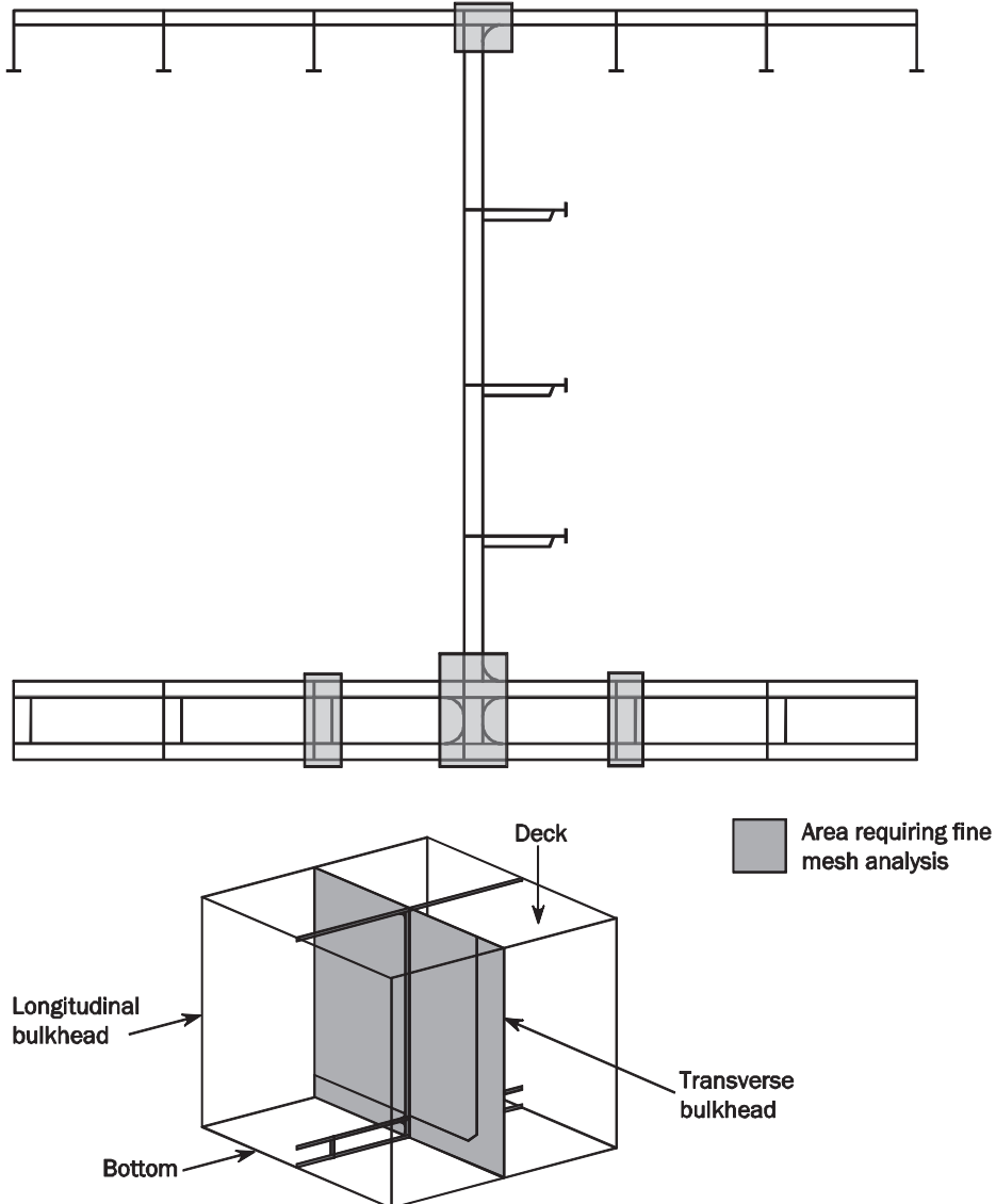
Fig. 3 Examples of Mandatory Areas at Connections between Double Bottom and Deck Longitudinals and Adjoining Structure of Transverse Bulkhead
