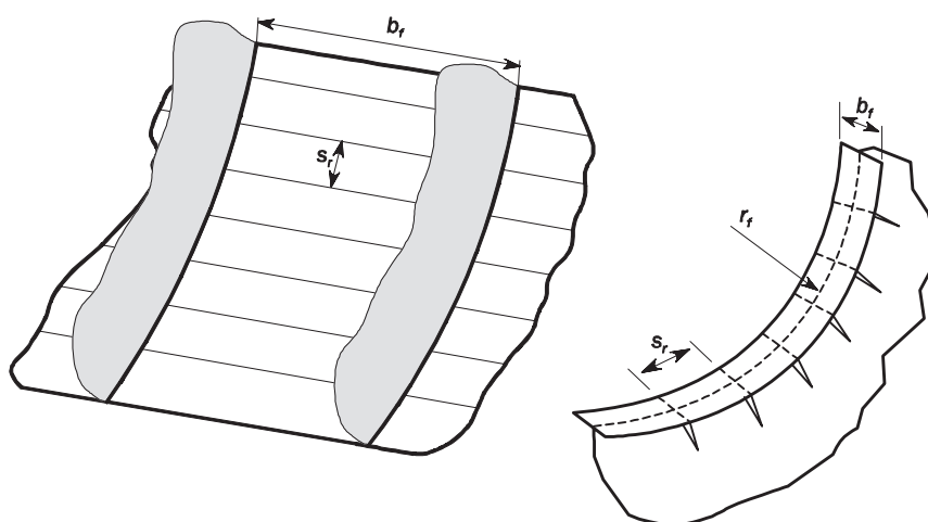
Fig. 12 Curved Shell Panel and Face Plate
