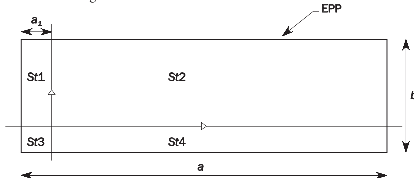
Fig. 17 Strake Considered in a Given EPP
