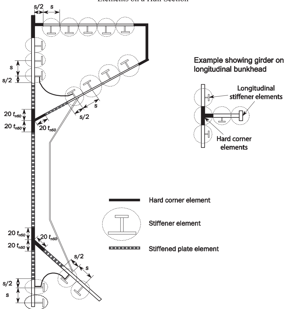
Fig.3 Examples of the Configuration of Stiffened Plate Elements, Stiffener Elements and Hard Corner Elements on a Hull Section
