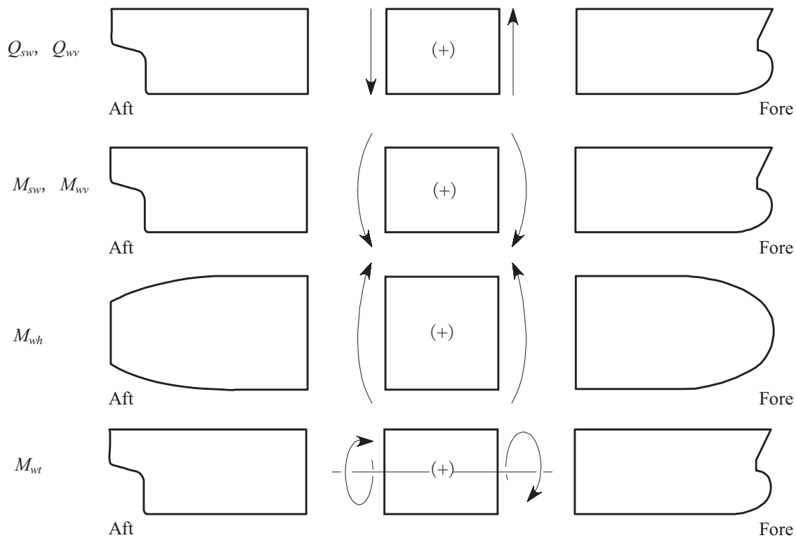
Fig. 2 Sign Conventions for Shear Forces Q_{sw} , Q_{wv} and Bending Moments M_{sw} , M_{wv} , M_{wh} and M_{wt}
