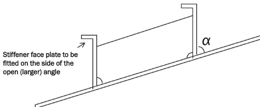
Fig. 2 Stiffener on Attached Plating with an Angle less than 50 deg
