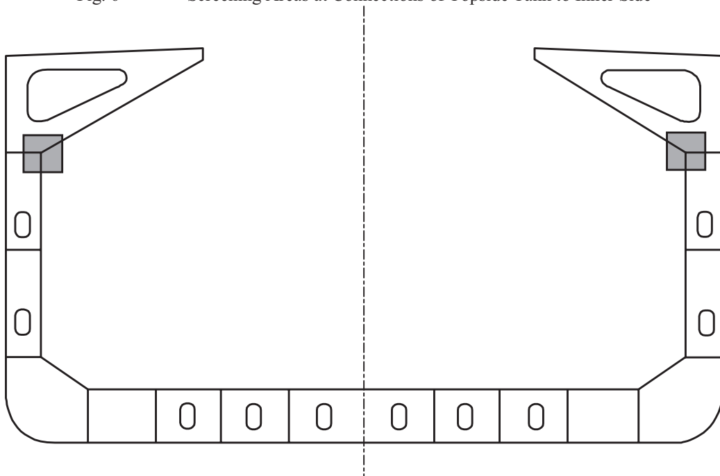
Fig. 6 Screening Areas at Connections of Topside Tank to Inner Side
