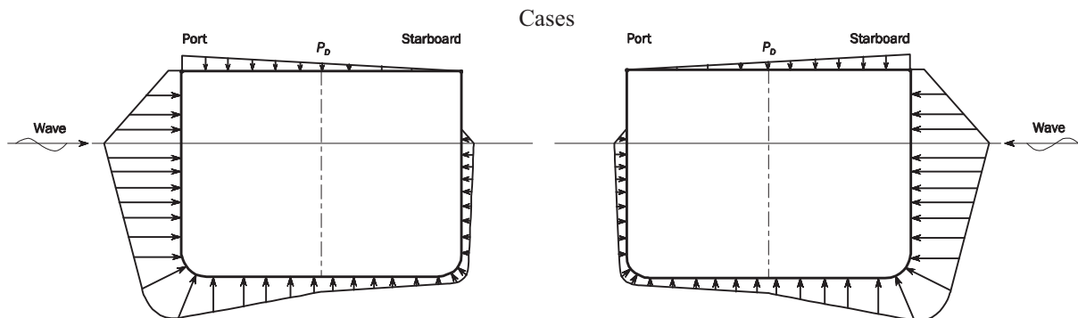
Fig. 10 Transverse Distribution of Dynamic Pressure Amidships for OSA-1P (Left) and OSA-1S (Right) Load Cases
