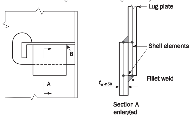
Fig. 2 Modelling of Eccentric Lug Plate by Shell Elements
