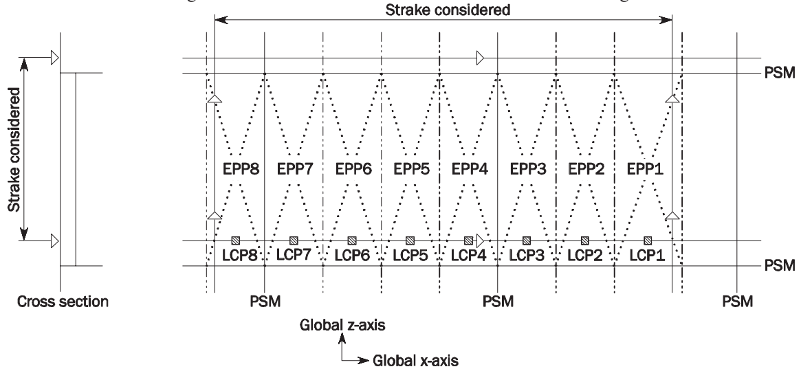
Fig. 19 Load Calculation Point for Transverse Framing
