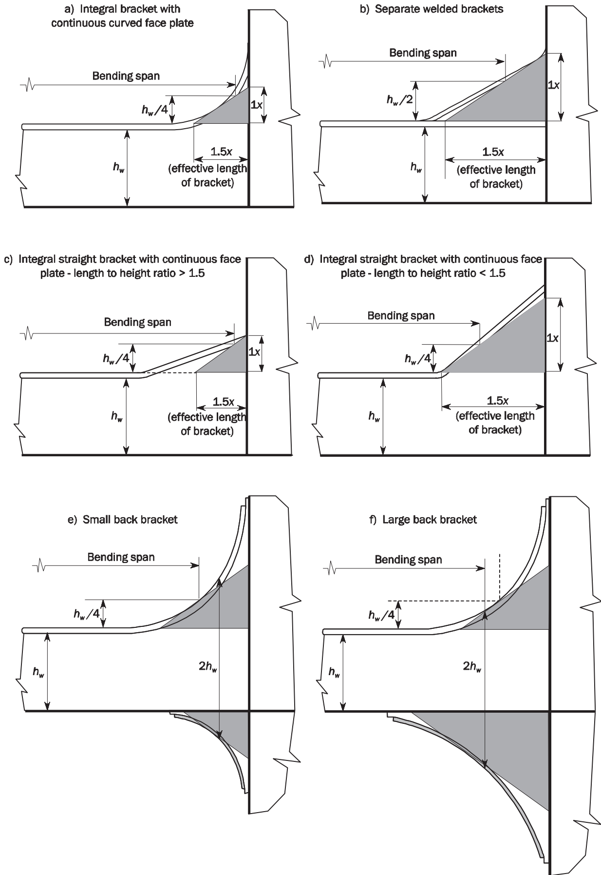
Fig.9 Effective Bending Span of Primary Supporting Member
