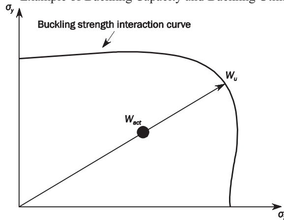
Fig. 1 Example of Buckling Capacity and Buckling Utilisation Factor
