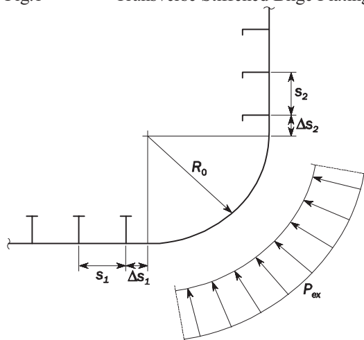
Fig.1 Transverse Stiffened Bilge Plating
