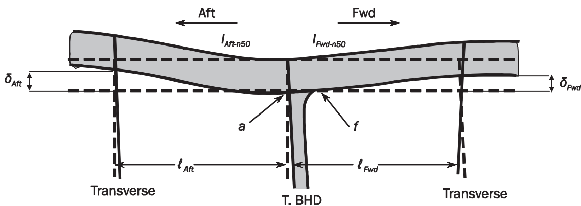
Fig. 4 Definition of the Relative Displacement (Example of the Side Longitudinal)
