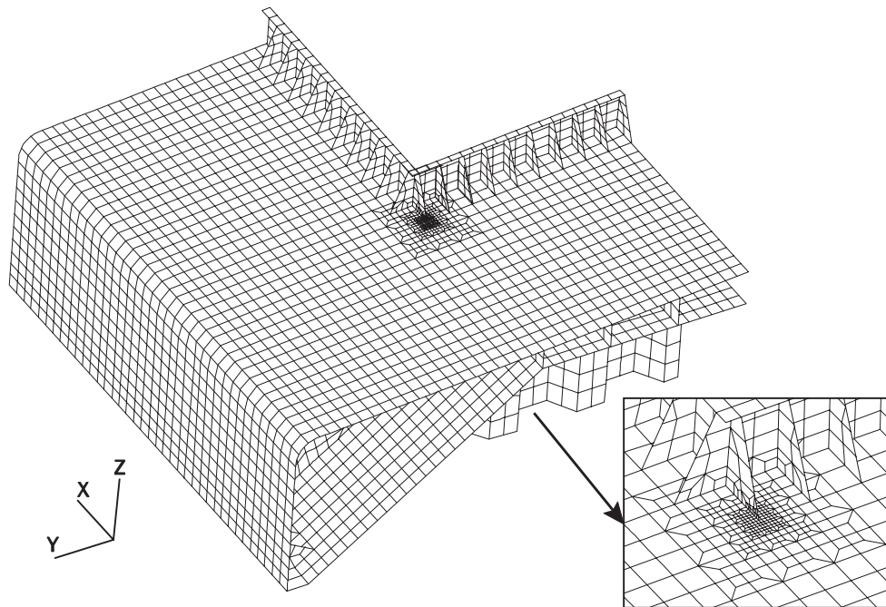
Fig. 12 Local FE Model of Longitudinal Hatch Coaming End Bracket to the Deck Plating with Very Fine Mesh Zone, t_{n50} \times t_{n50} Mesh
