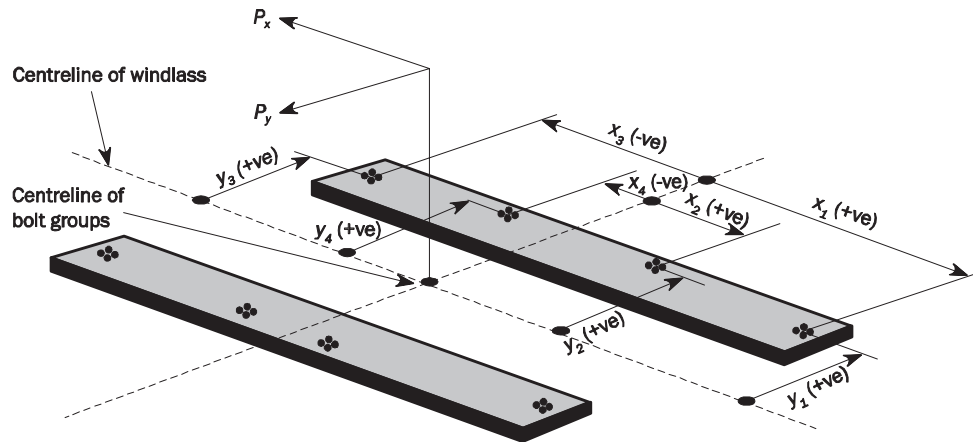
Fig. 2 Bolting Arrangements and Sign Conventions
