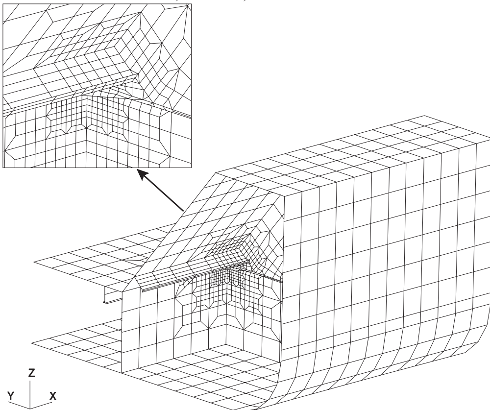
Fig. 4 Local Very Fine Mesh Model ( t_{n50} \times t_{n50} ) of Hopper Knuckle Connection between Inner Bottom, Hopper Plate, Web Frame, Girder and Bracket
