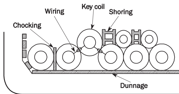
Fig. 8 Inner Bottom Loaded by Steel Coils
