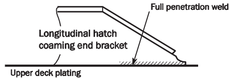
Fig. 3 High Stress Areas Welding (examples)
