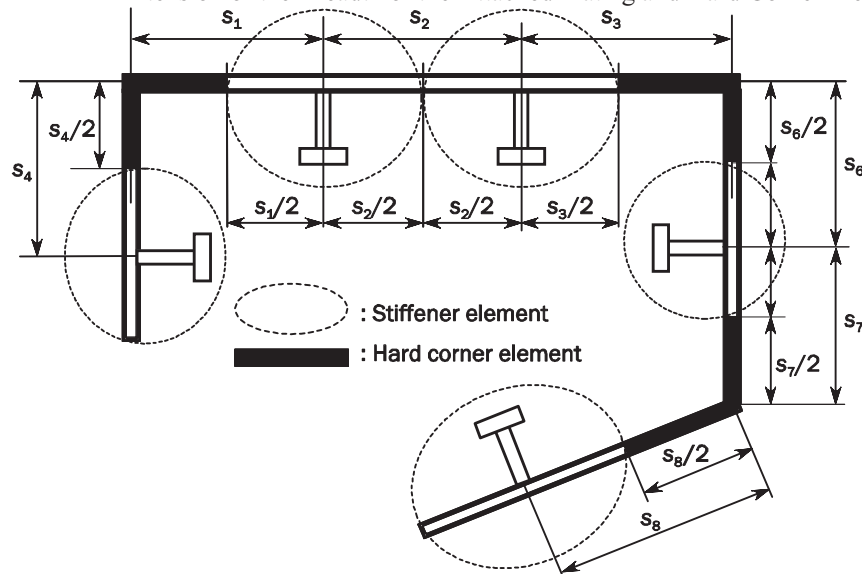
Fig. 4 Extension of the Breadth of the Attached Plating and Hard Corner Element
