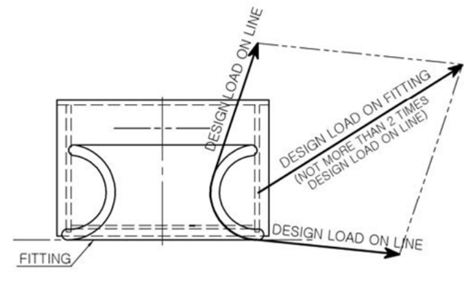
Fig. 4 Design Load on Fitting
