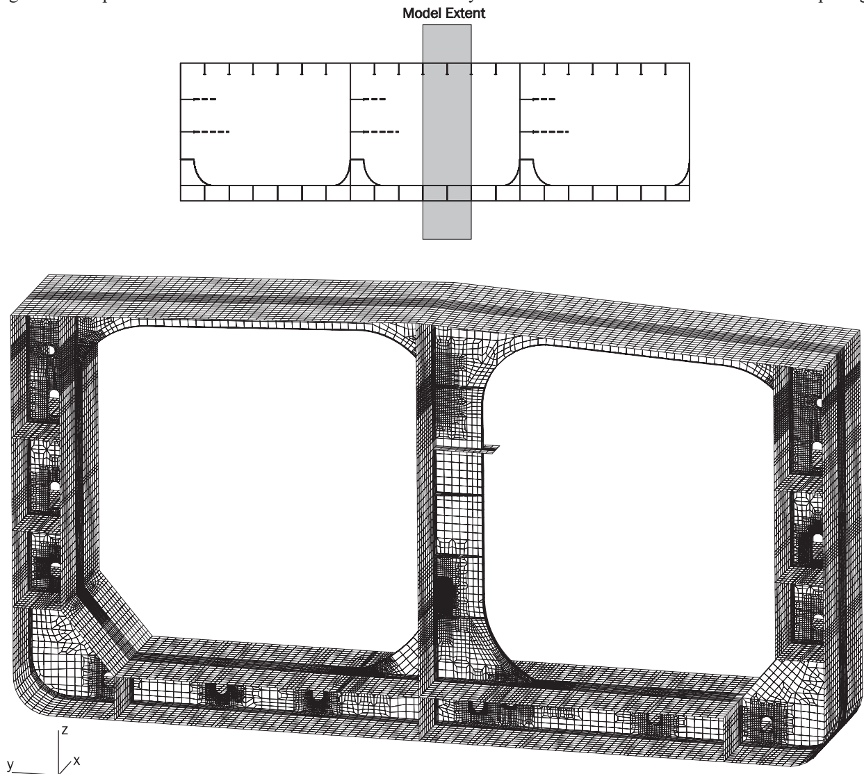
Fig. 1 Example of Extent of Local Model for Fine Mesh Analysis of Web Frame Bracket Connections and Openings
