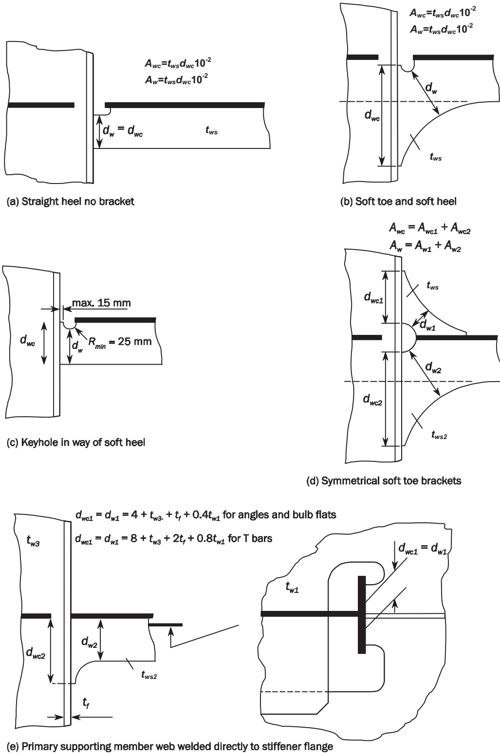
Fig. 9 Primary Supporting Member Web Stiffener Details
