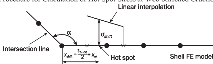
Fig. 20 Determination of Stress Read out Points for Web-stiffened Cruciform Connections
