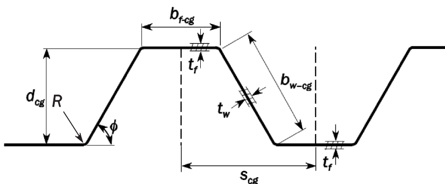
Fig. 21 Dimensions of a Corrugated Bulkhead
