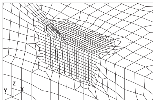
Fig. 10 Fine Mesh Zone around an Opening
