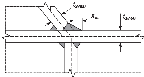
Fig. 18 Geometrical Parameters of Web-stiffened Cruciform Connections
