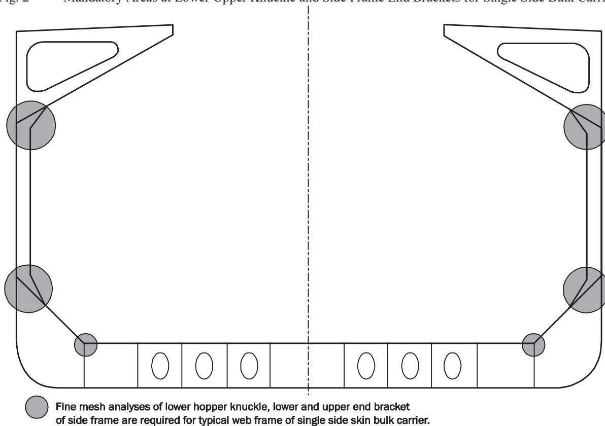
Fig. 2 Mandatory Areas at Lower Upper Knuckle and Side Frame End Brackets for Single Side Bulk Carrier
