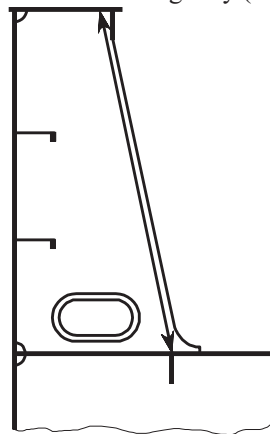
Fig. 6 Coaming Stay (Example 4)
