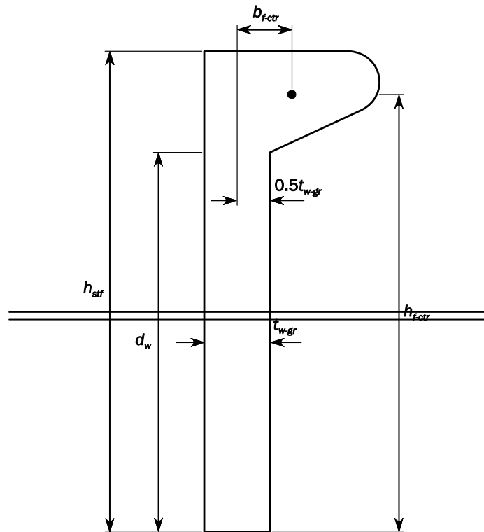
Fig. 15 Characteristic Data for Bulb Profiles
