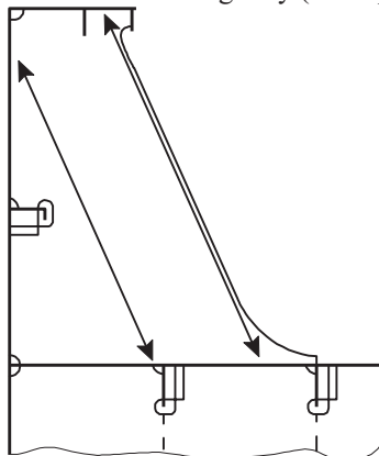
Fig. 3 Coaming Stay (Example 1)
