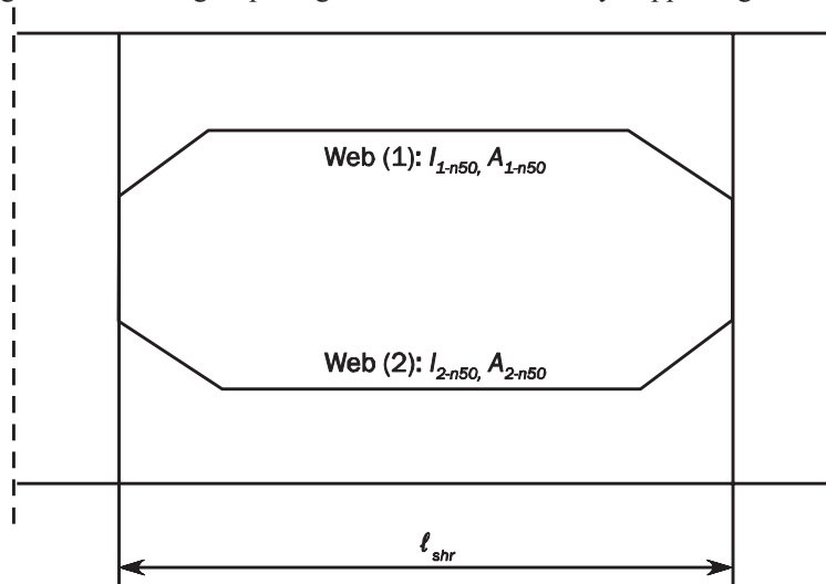
Fig. 14 Large Openings in the Web of Primary Supporting Members
