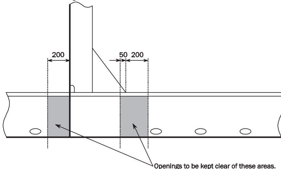
Fig. 12 Location of Air and Drain Holes
