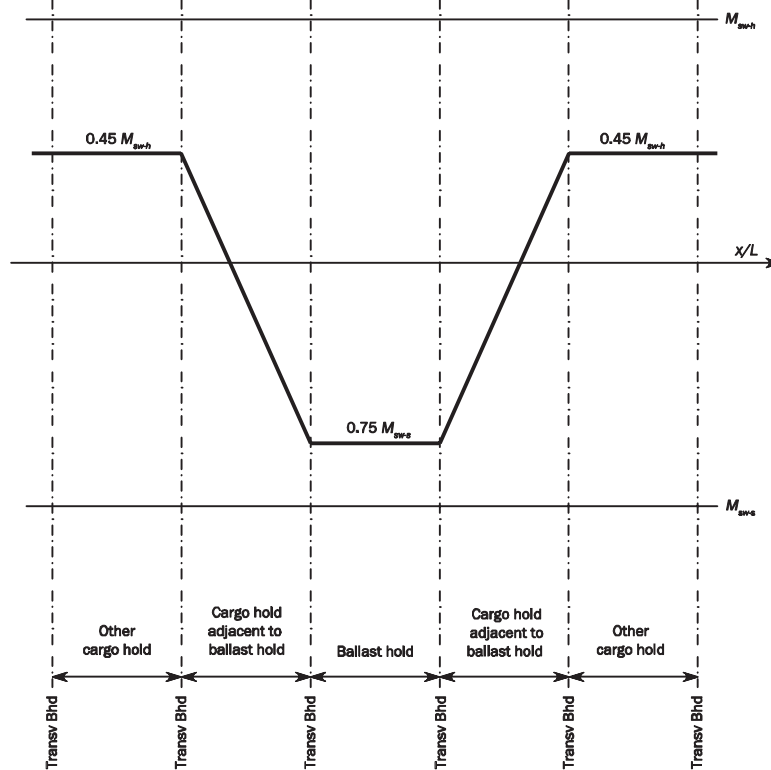
Fig. 1 Distribution of Still Water Bending Moment for Fatigue Assessment in way of Ballast Hold
