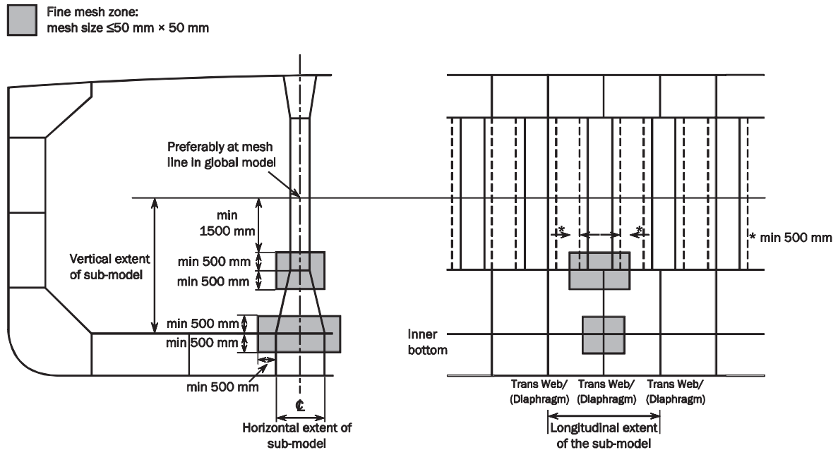
Fig. 18 Extent of Local Model and Fine Mesh Zone for the Analysis of Corrugated Bulkhead Connection to Lower Stool and Inner Bottom
