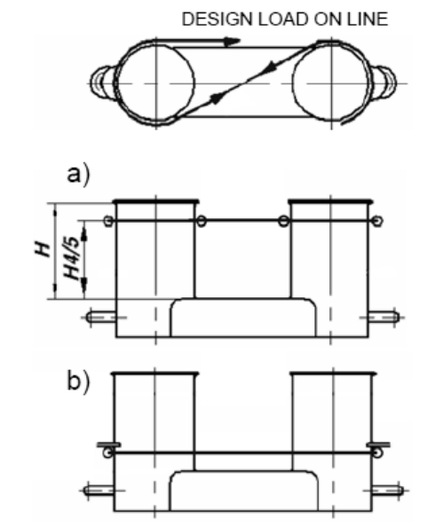
Fig. 6 Attachment point of the mooring line
