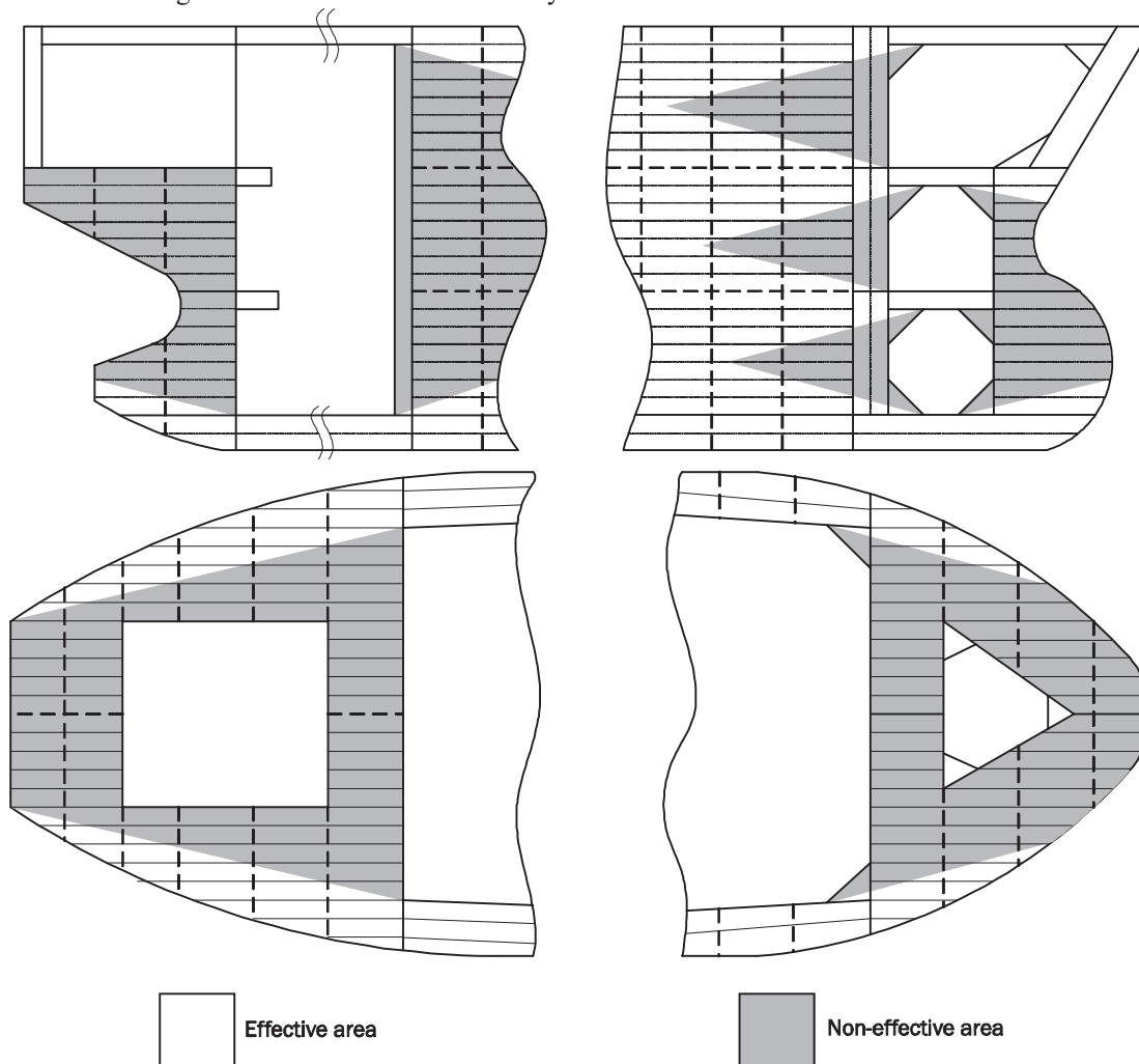
Fig. 2 Effective Area in way of Non-continuous Decks and Bulkheads
