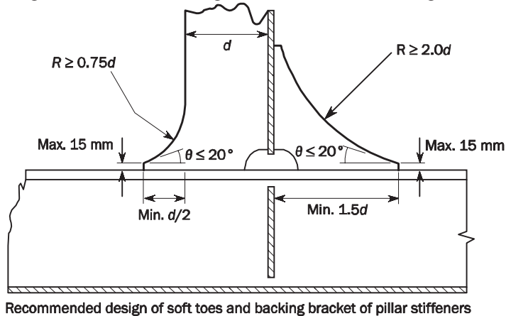
Fig. 9 Detail Design for Soft Toes and Backing Brackets
