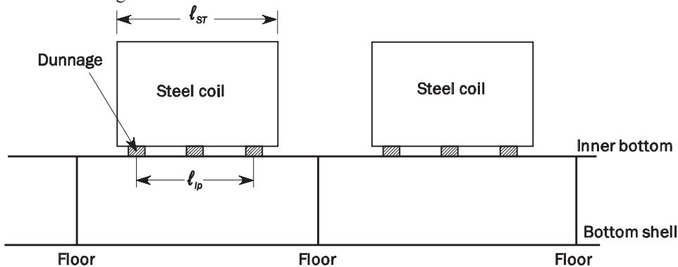
Fig. 10 Steel Coils Loaded between Inner Bottom Floors
