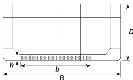
Fig. 2 Damage Extent for Grounding
