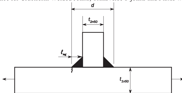
Fig. 2 Toe Distance for Cruciform Welded Joints, Transverse T -joints and Plates with Transverse Attachment
