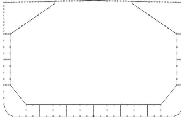
Fig. 18 End Constraint Beams for a Bulk Carrier
