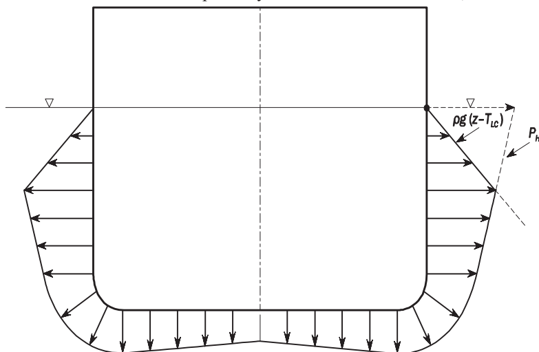
Fig. 2 Transverse Distribution Amidships of Dynamic Pressure for HSM-1, HSA-1 and FSM-1 Load Cases
