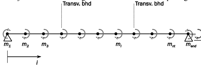
Fig. 19 Adjustments of Bending Moments outside Midship Cargo Hold Region
