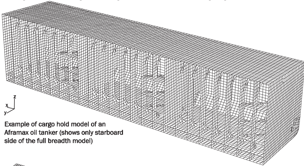
Fig. 3 Example of 3 Cargo Hold Model within Midship Region of Oil Tankers
