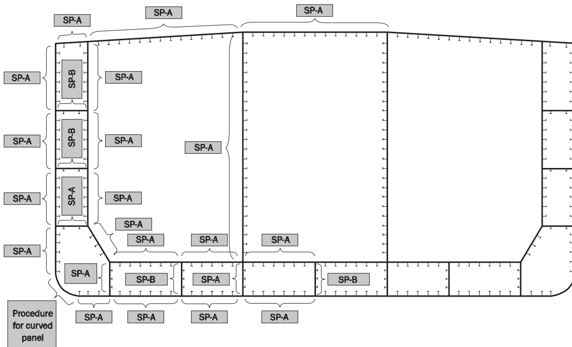
Fig. 1 Longitudinal Plates for Oil Tankers
