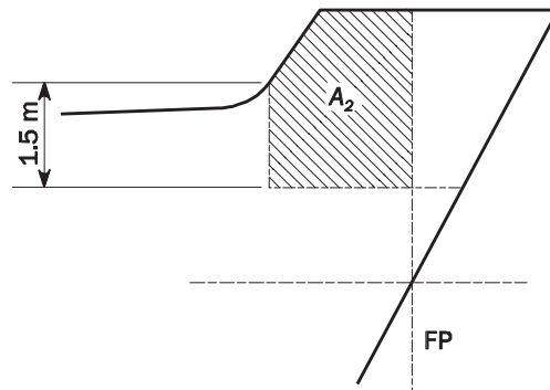
Fig. 2 Profile Areas of Screens and Bulwarks
