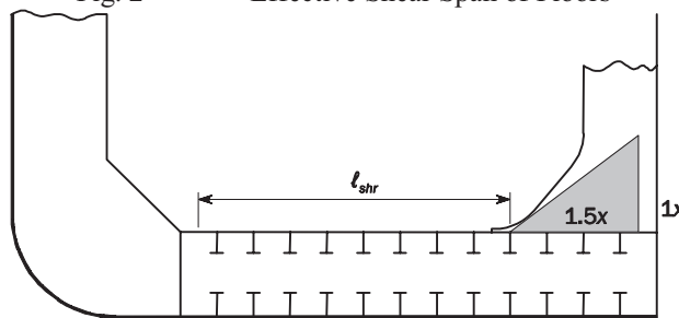
Typical arrangement with hopper and end bracket
