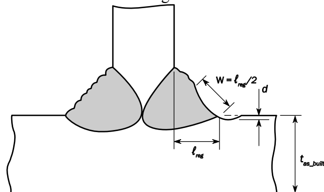
Fig. 6 Extent of Weld Toe Burr Grinding to Remove Inter-bead Toes on Weld Face
