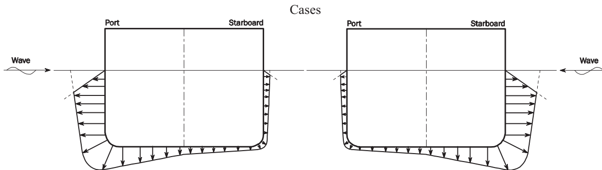
Fig. 11 Transverse Distribution of Dynamic Pressure Amidships for OSA-2P (Left) and OSA-2S (Right) Load Cases
