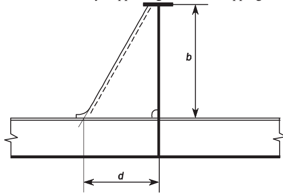
Tripping bracket in way of stiffener
