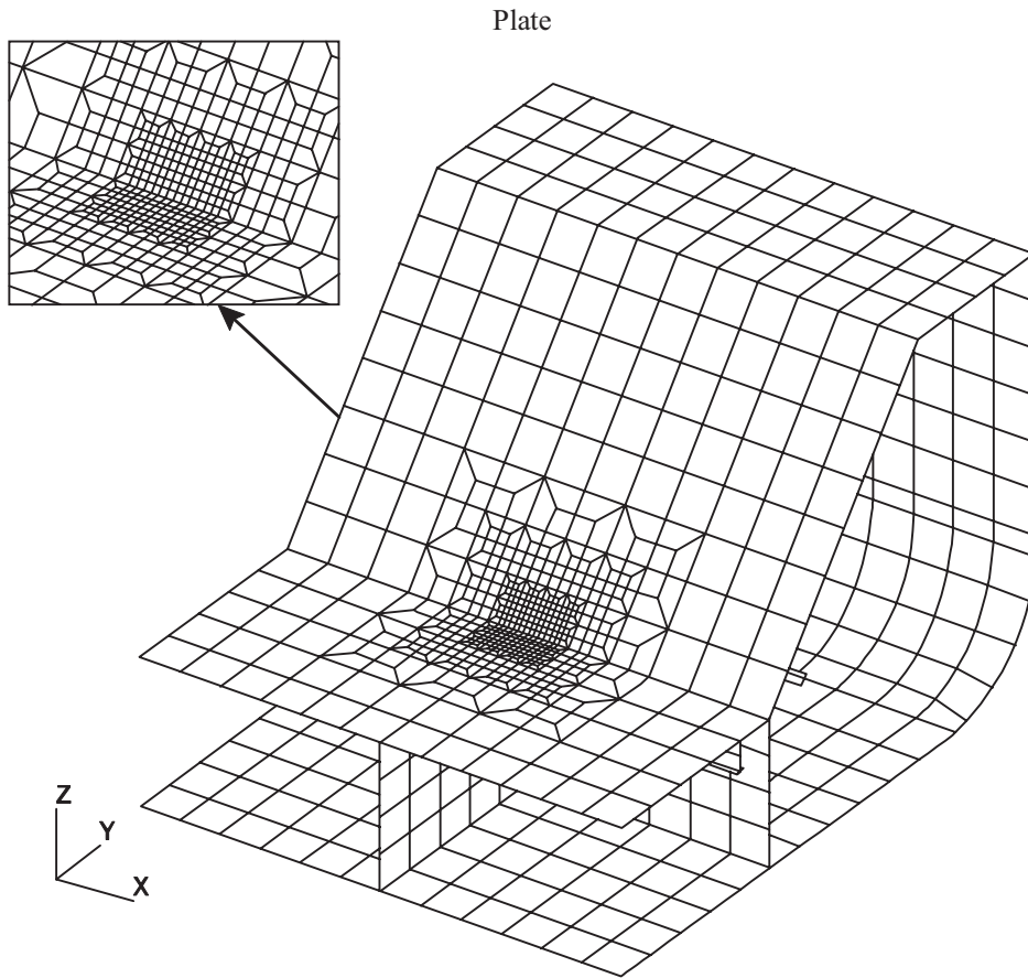
Fig. 3 Local Very Fine Mesh Model ( t_{n50} \times t_{n50} ) of Hopper Knuckle Connection between Inner Bottom and Hopper
