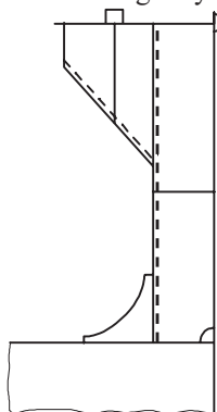
Fig. 4 Coaming Stay (Example 2)
