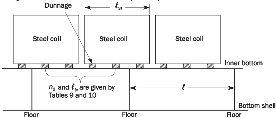
Fig. 9 Steel Coils Loaded Independently of Inner Bottom Floors Locations
