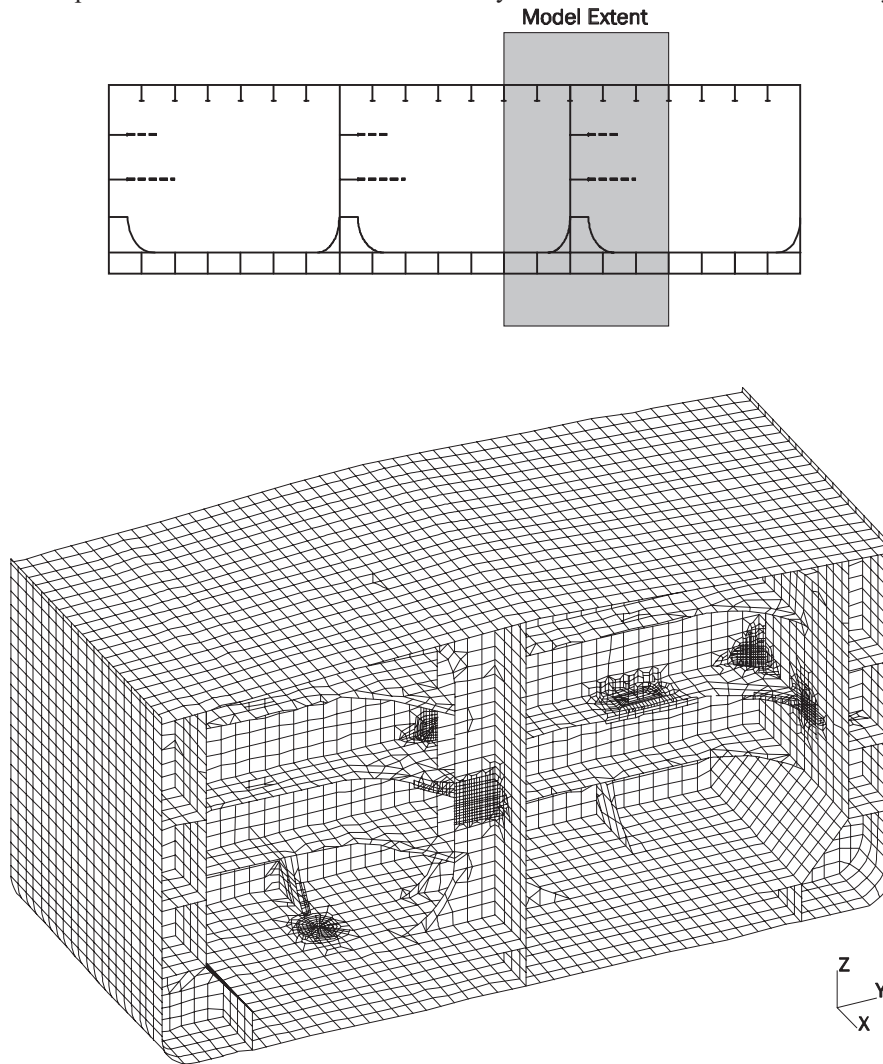
Fig. 13 Example of Local Model for Fine Mesh Analysis of Transverse Bulkhead and Adjacent Structure
