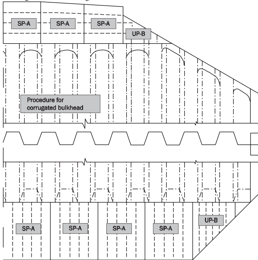
Fig. 9 Corrugated Bulkhead and Cross Deck for Bulk Carriers
