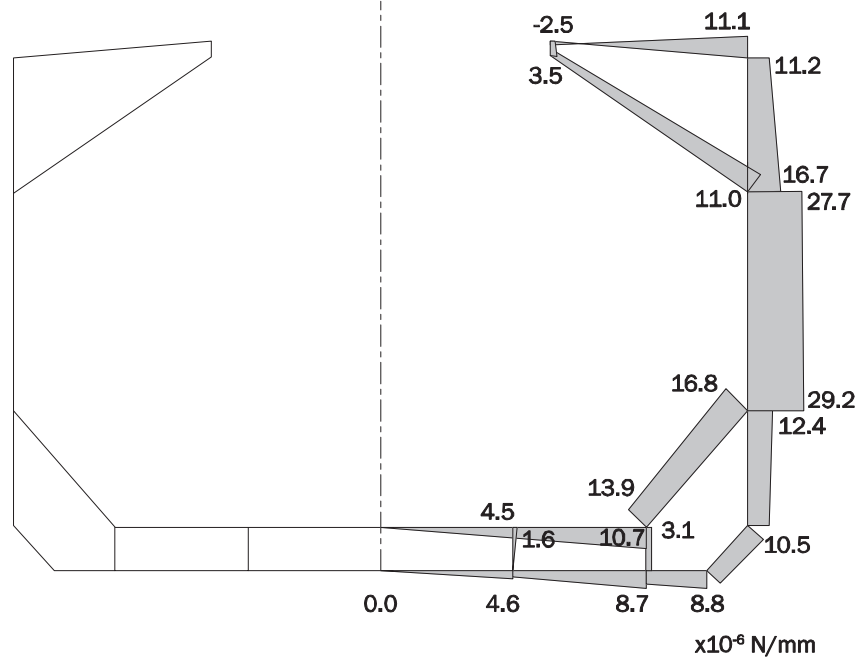
Fig. 7 Calculation Results of Shear Flow q_V , in 10^{-6} N/mm for Vertical Shear Force with 1N
