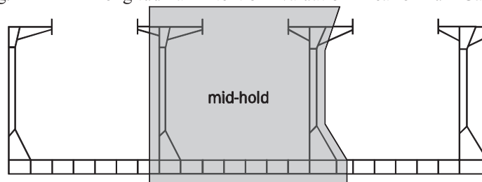
Fig. 22 Longitudinal Extent of Evaluation Area for Bulk Carrier
