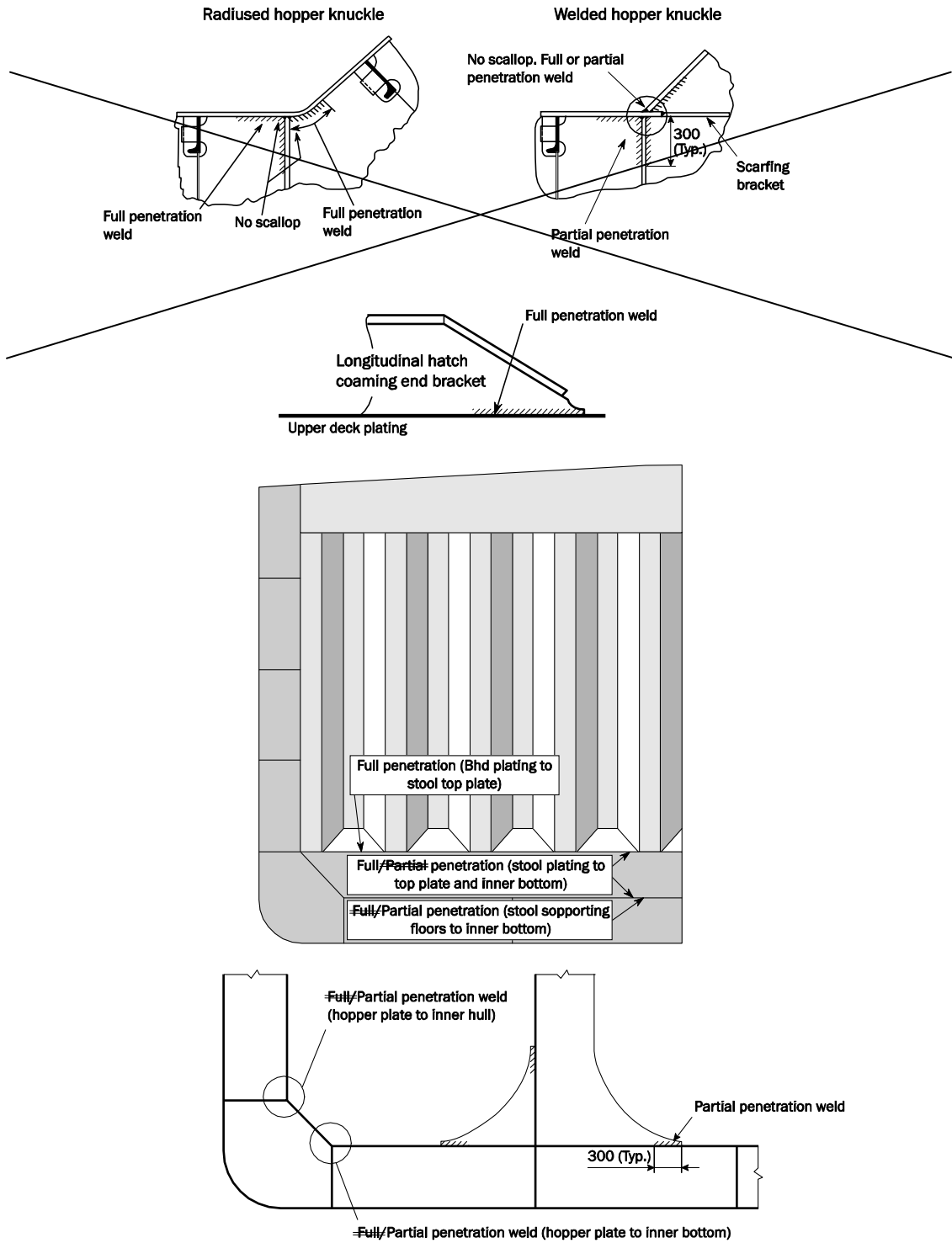
Fig. 3 High Stress Areas Welding (examples)
