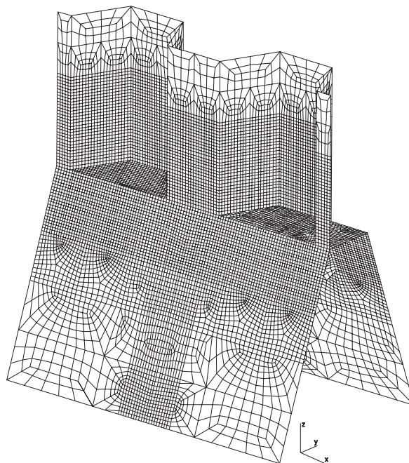
Fig. 19 Example of Partial Local Model for the Analysis of Connection of Corrugated Bulkhead to Lower Stool
