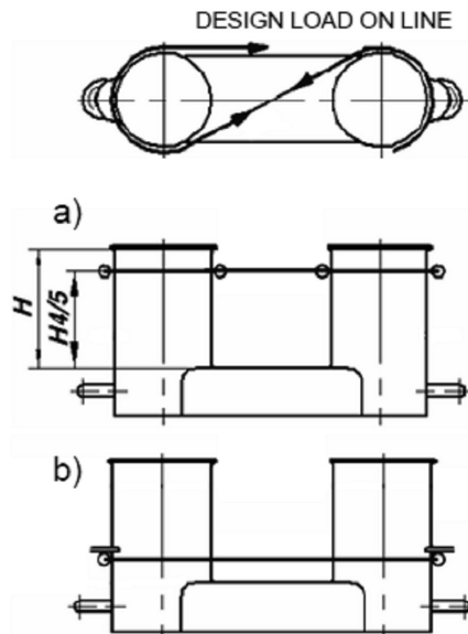
Fig. 6 Attachment point of the mooring line
