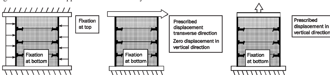
Fig. 3 Load Application and Boundary Conditions – FE Model for Verification of Alternative Design
