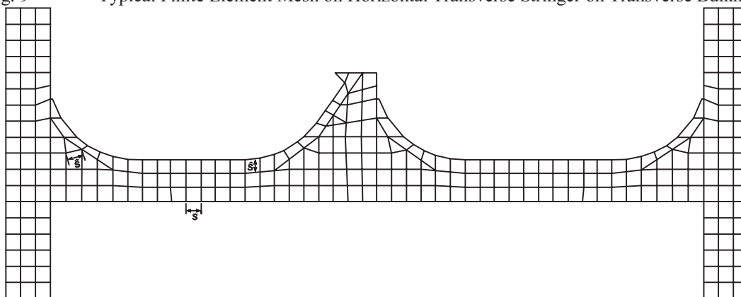
Fig. 9 Typical Finite Element Mesh on Horizontal Transverse Stringer on Transverse Bulkhead
