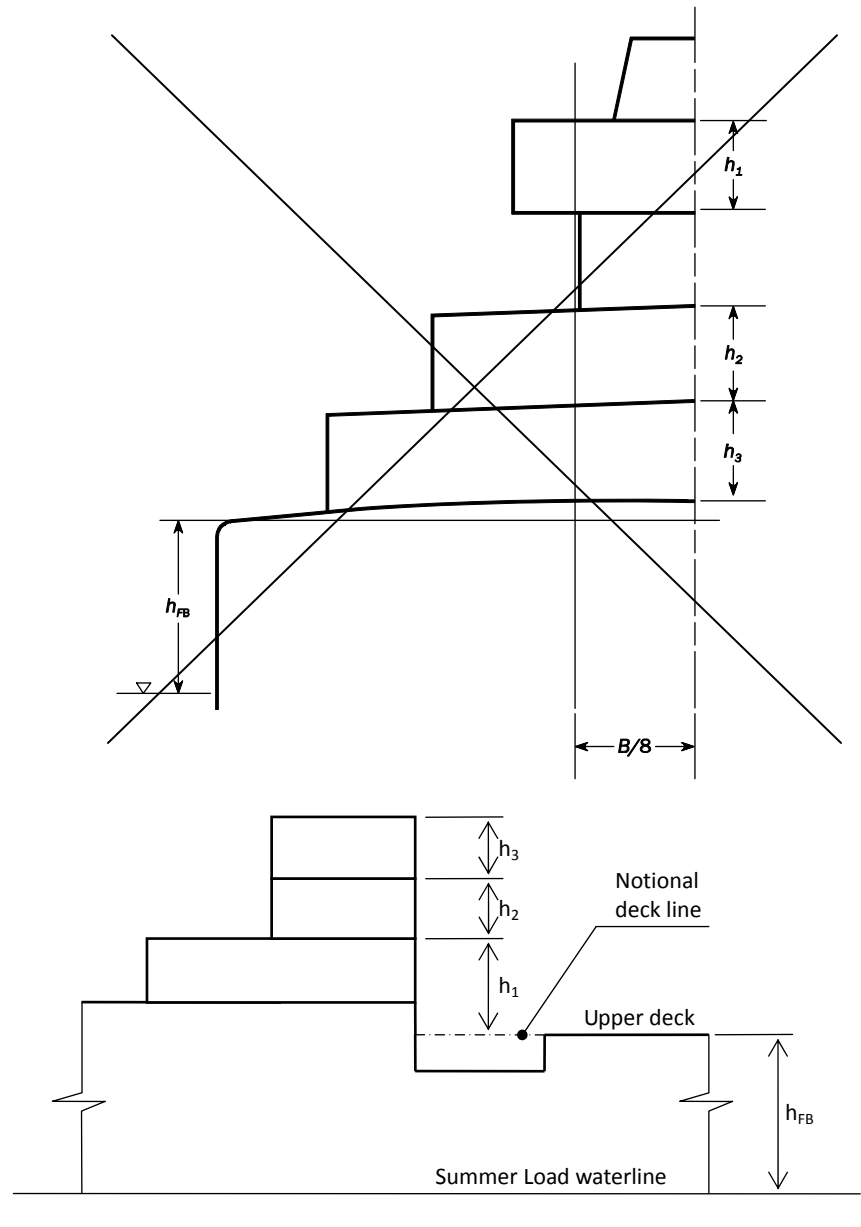
Fig. 1 Effective Heights of Deckhouses Measurement of heights
