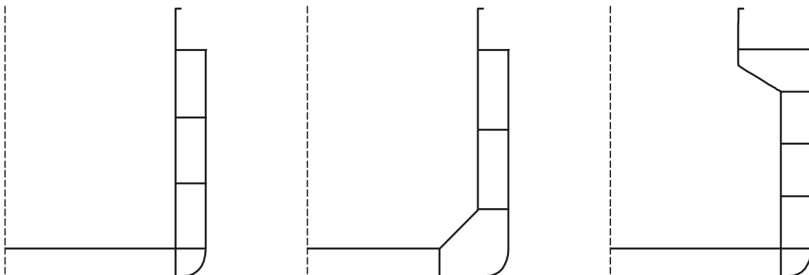
Fig. 2 Examples of Transverse Sections of Cargo Hold without Hopper Tank and/or Topside Tank
