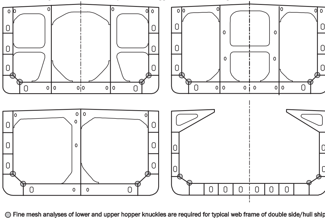
Fig. 1 Mandatory Areas at Hopper Knuckles for Ships with Double Side
