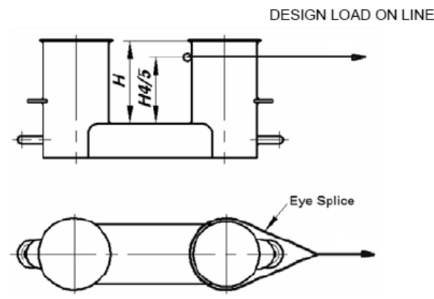
Fig. 5 Attachment point of the towing line
