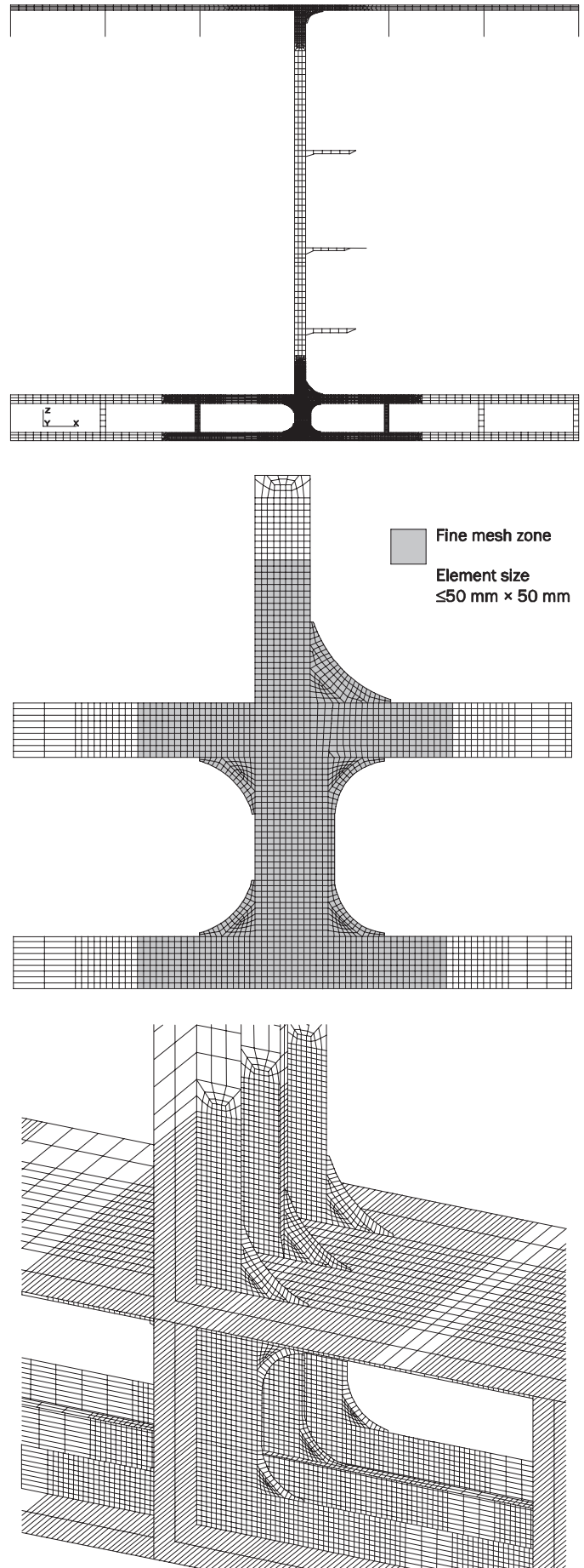
Fig. 17 Example of Local Model for Fine Mesh Analysis of End Connections and Web Stiffeners of Deck and Double Bottom Longitudinals
