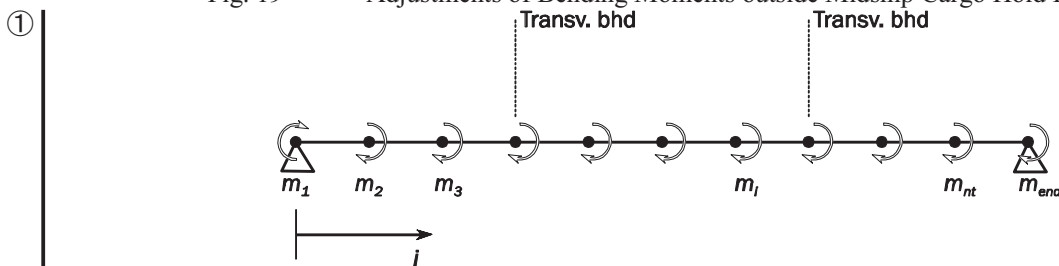
Fig. 19 Adjustments of Bending Moments outside Midship Cargo Hold Region
