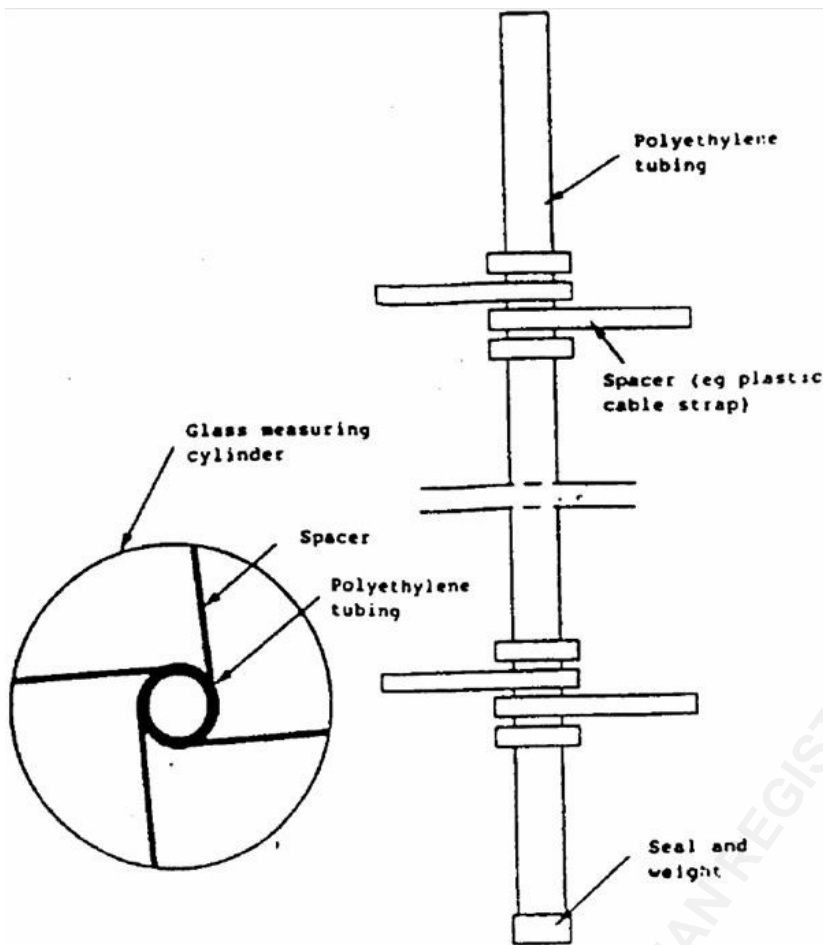
Figure 1 - Typical form of polyethylene tube
