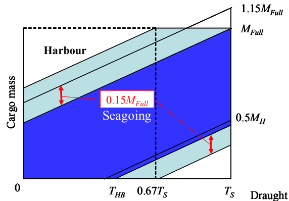
Figure 2.4: Example of mass curve for BC-B or BC-C ships Example of mass curve for BC-B and BC-C ships having {No MP} assigned
