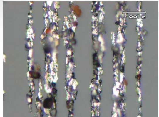
Microscopic analysis of lubricant
