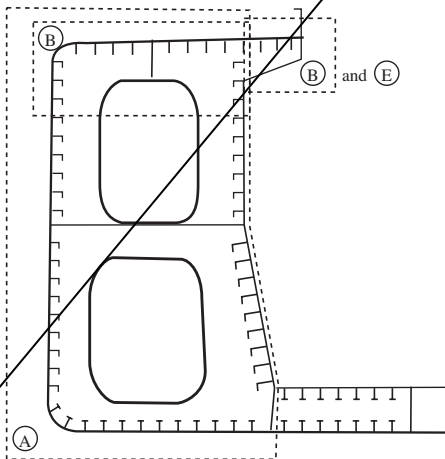
Typical transverse section close-up survey
