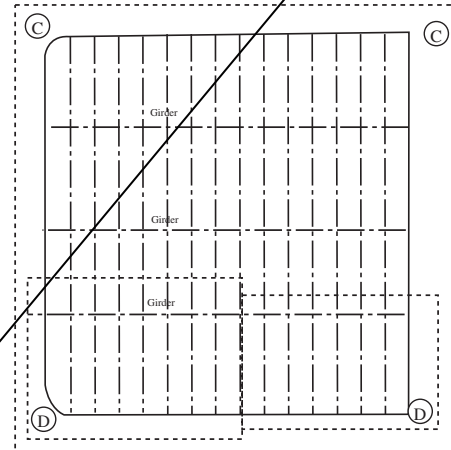
Typical transverse bulkhead
