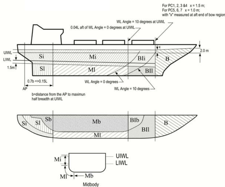
Figure 1 - Hull Area Extents
