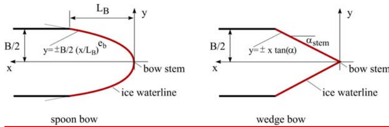
Figure 8 - Illustration of e_b Effect on the Bow Shape for B = 20 and L_B = 16
