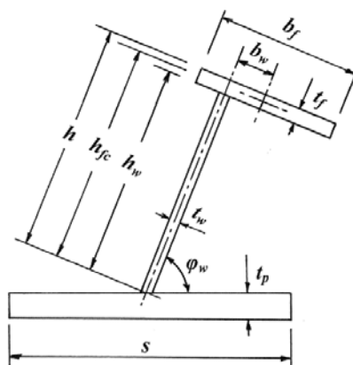
Figure 4 - Stiffener geometry
