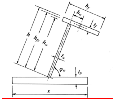
Figure 4 - Stiffener geometry
