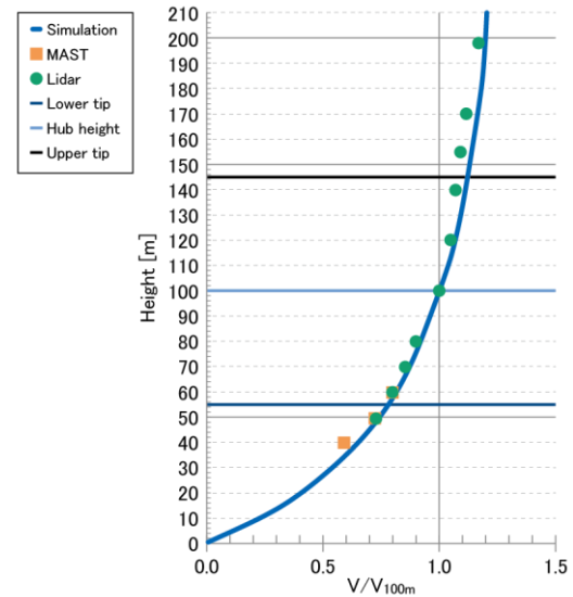
Figure B.3 Measurement mast + vertical lidar (Displacement height not set)
