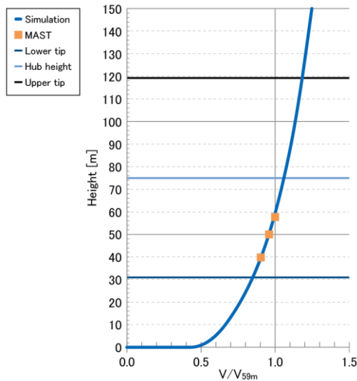
Figure B.2 Measurement mast only (Displacement height not set)
