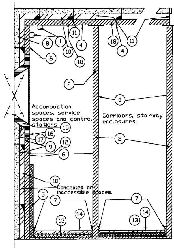
Figure 1: Constructural elements in accomodation spaces
