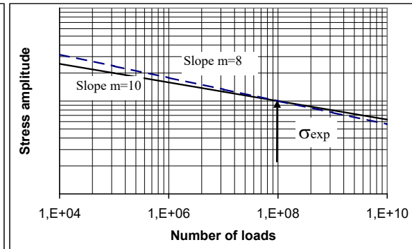
Figure 6: Constant-slope S-N curve
