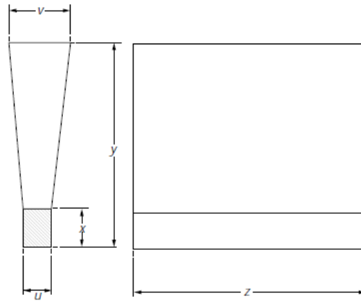
Fig2. Separately cast or side-by-side cast blocks (Y-shaped block)
