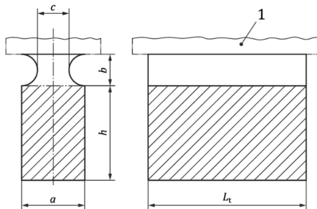
Fig 3. Cast-on test block
