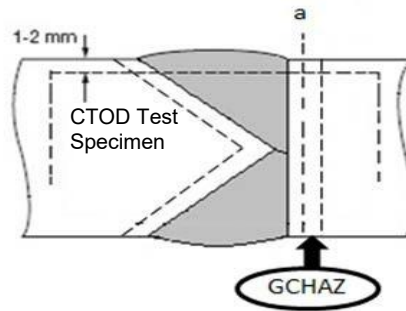
Figure A1 a) – For plate thickness t \leq 50 mm, CTOD test specimen is to be sampled in full thickness
