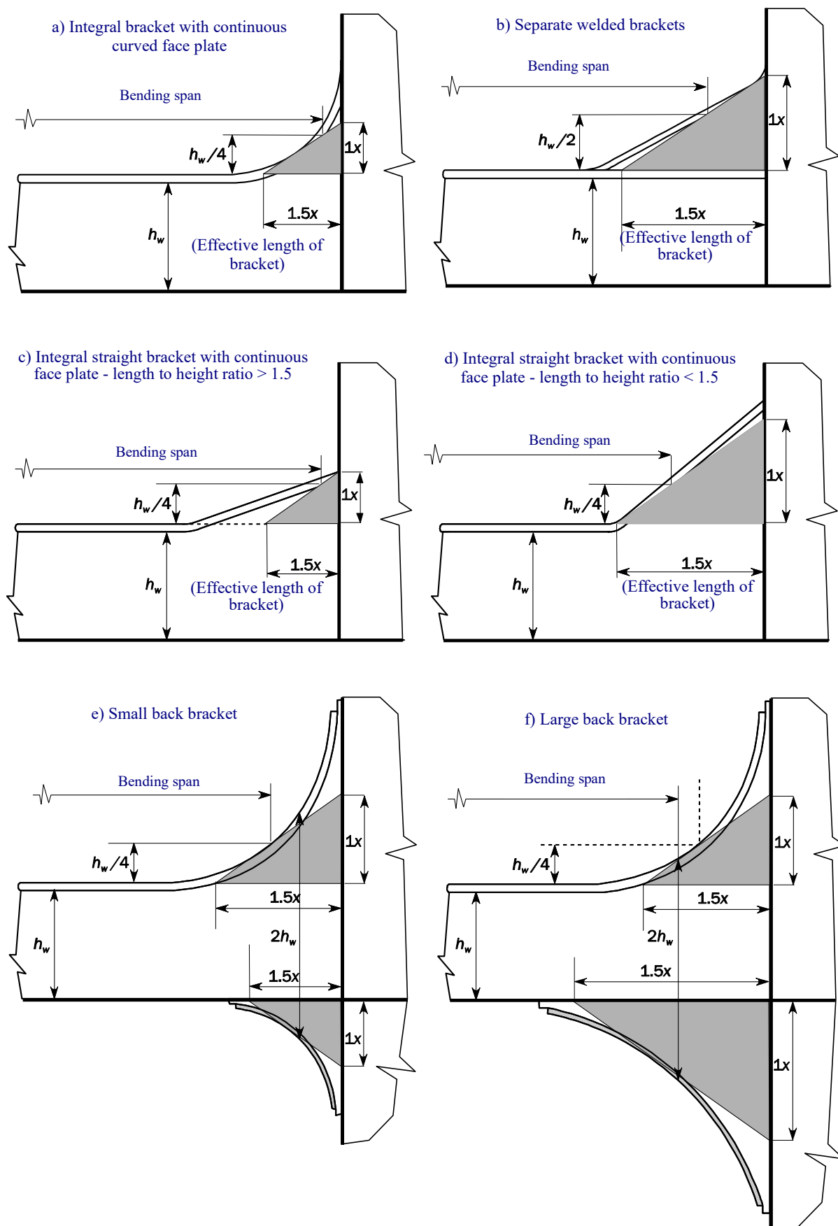
Fig. 3.6.1-5 Effective Bending Span of Primary Supporting Member
