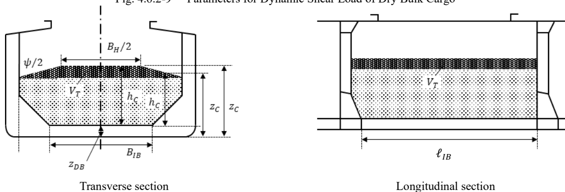
Fig. 4.6.2-9 Parameters for Dynamic Shear Load of Dry Bulk Cargo
