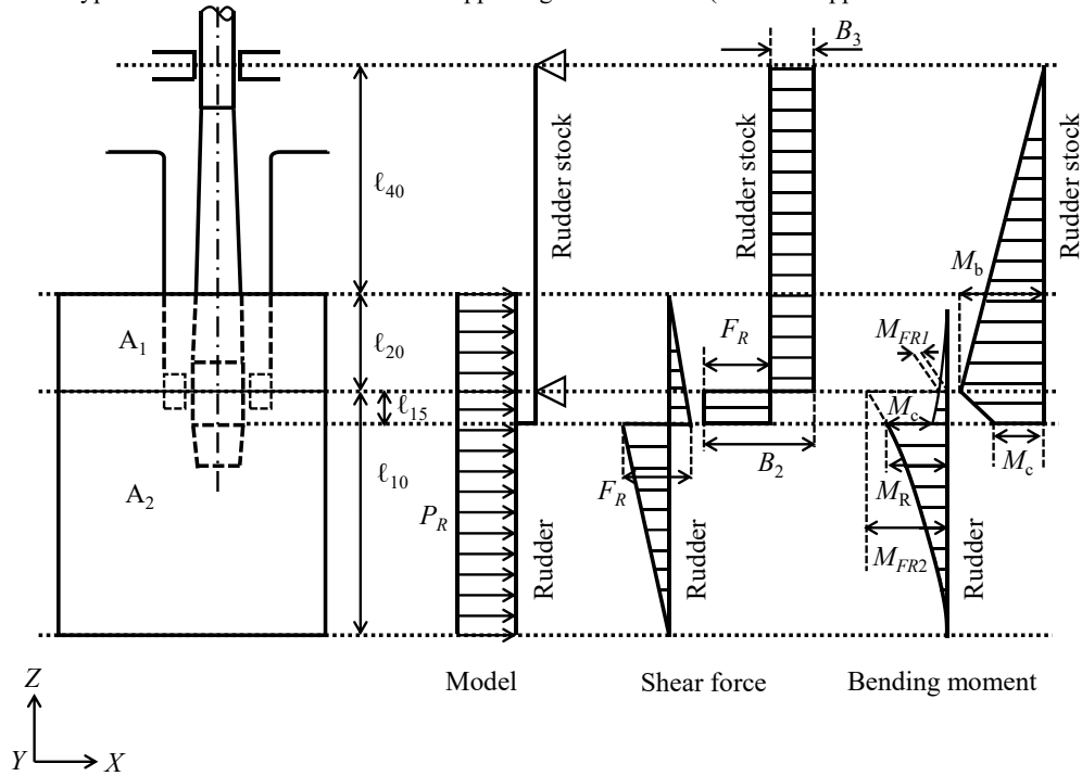
Fig. C13.2.4-6 Type C Rudder with Rudder Trunk Supporting Rudder Stock (Pressure Applied on the Entire Rudder Area)
