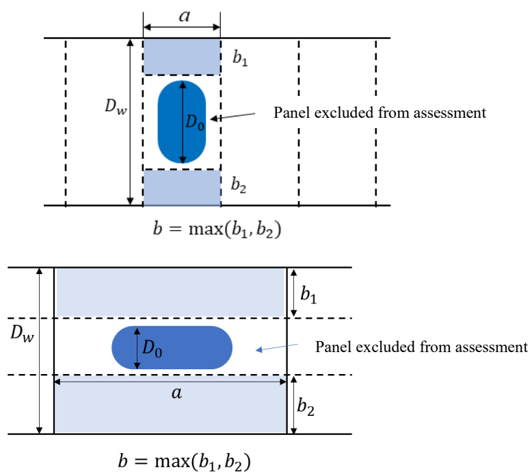
Fig. 7.2.5-2 Parameter Settings for an Opening Reinforced by Stiffeners in the Girder Span Direction
