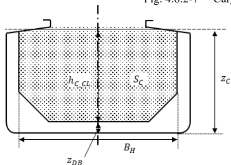
Fig. 4.6.2-7 Cargo Hold Loaded with Dry Bulk Cargo
