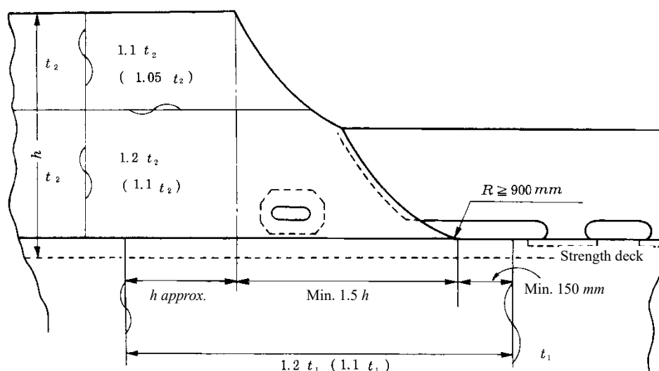
Fig. C11.3.2-1 Construction of Superstructure End (Where Expansion Joint is Installed)
