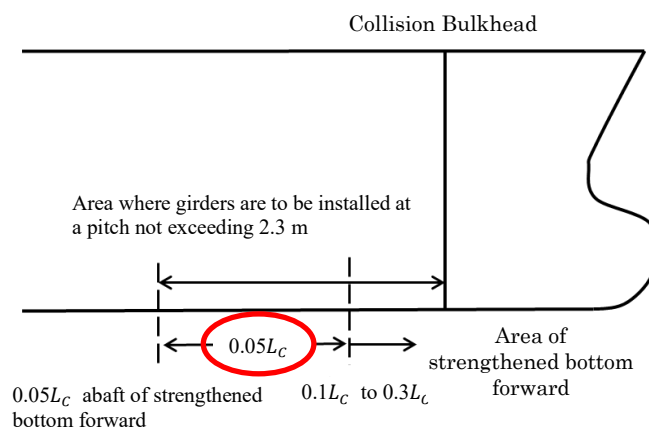
Fig. 10.6.2-1 Region where Girders are to be Installed Closely
