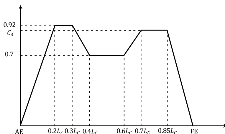
Fig. 4.3.2-4 Coefficient of Distribution along the Ship Length, C_{2n}
