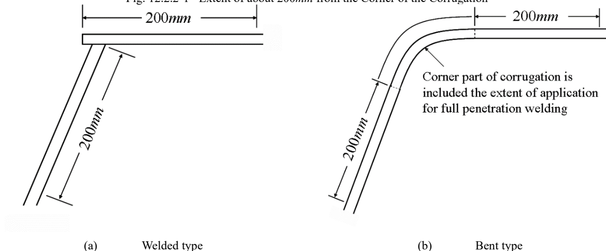
Fig. 12.2.2-1 Extent of about 200mm from the Corner of the Corrugation
