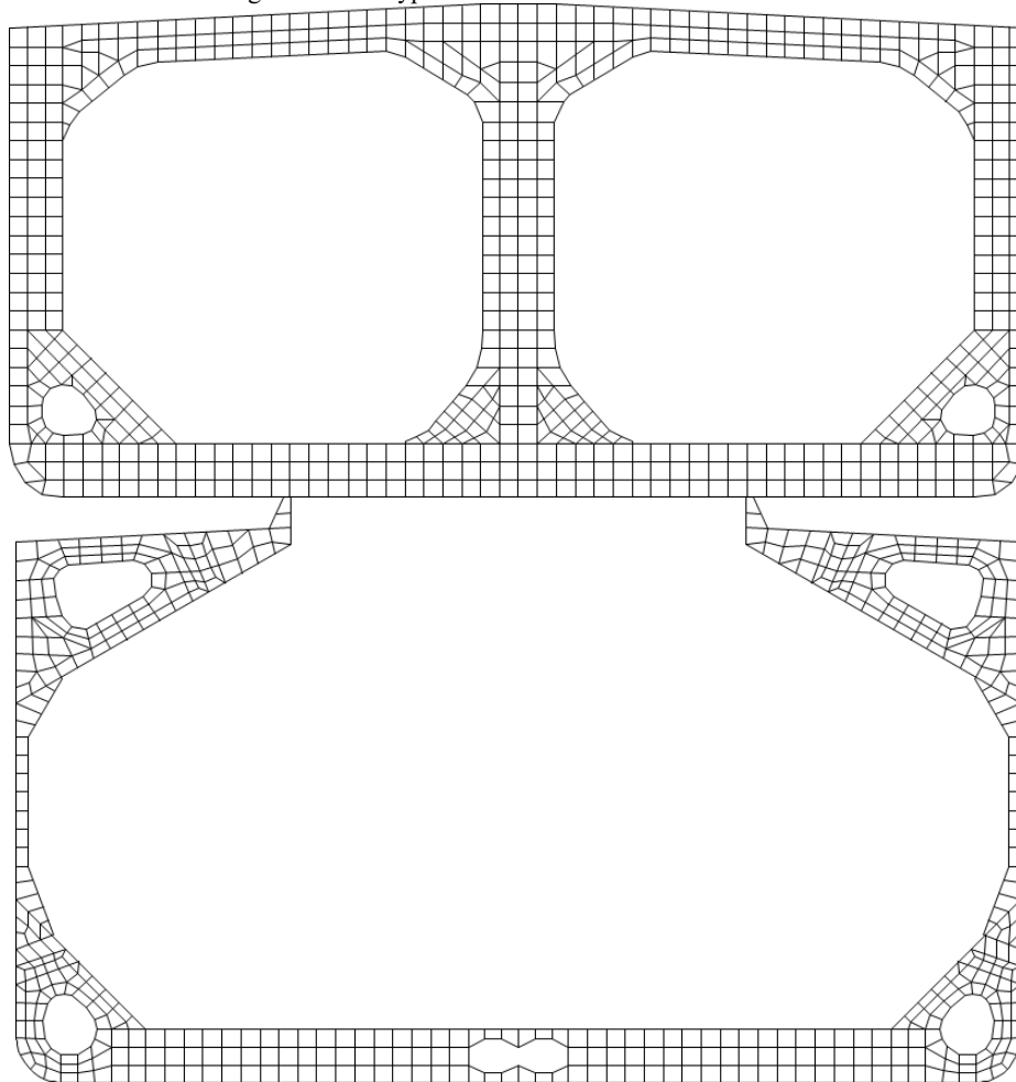
Fig. 8.3.3-1 Typical Mesh Size on Transverse Girder
