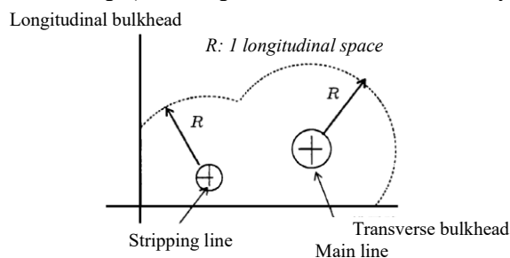
Fig. 3.3.4-2 Thickness Increase Range (With Longitudinal Bulkhead in the Vicinity of the Suction Bellmouth)
