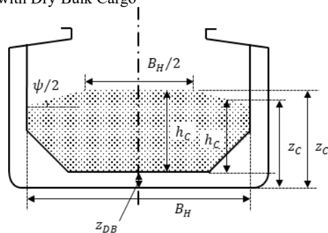
Fig. 4.6.2-7 Cargo Hold Loaded with Dry Bulk Cargo
