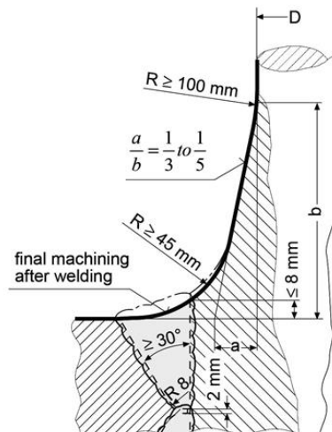
Fig. 13.2.8-1 Welded Joint between Rudder Stock and Coupling Flange
