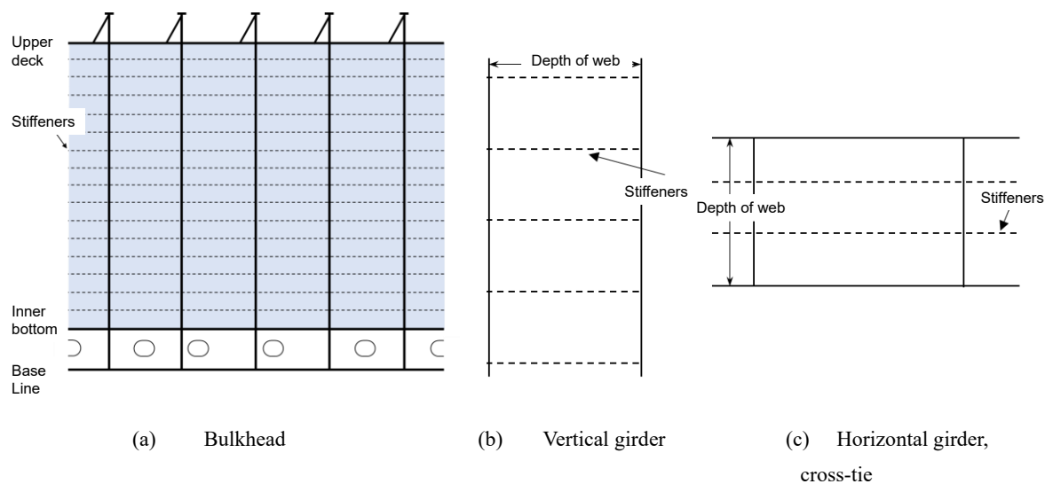
Fig. 10.9.3-2 Stiffened System B
