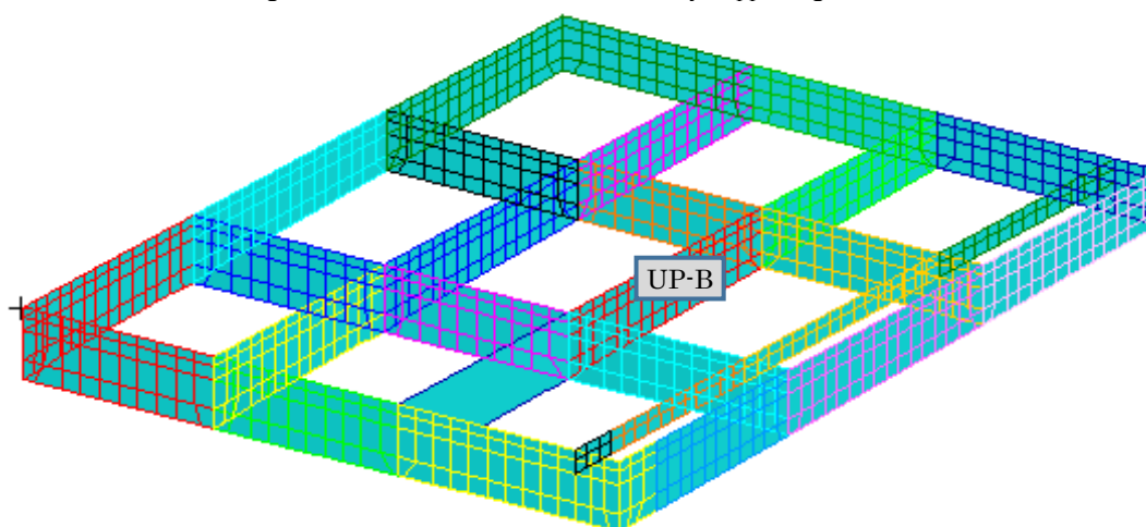
Fig. 14.6.5-4 Hatch Cover Webs of Primary Supporting Members
