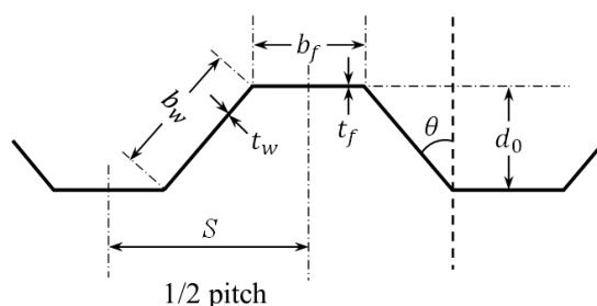
Fig. 10.9.2-1 1/2 Pitch of Corrugated Bulkheads
