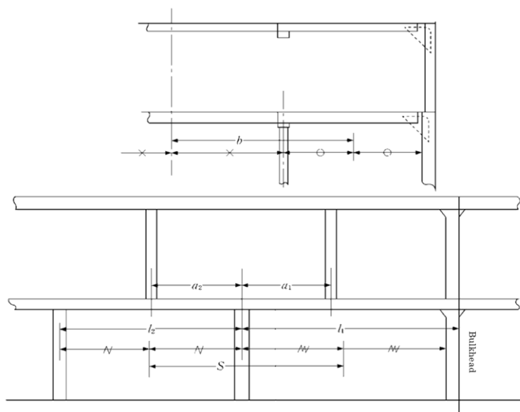
Fig. C7.4.2-1 Measurement of S , b , etc.
