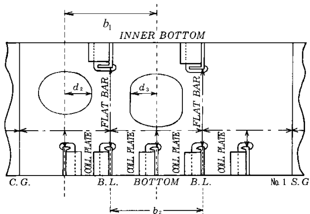
Fig. 10.6.3-1 Floor
