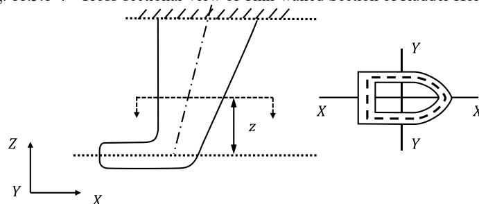
Fig. 11.5.1-4 Cross-sectional View of Thin-walled Section of Rudder Horn
