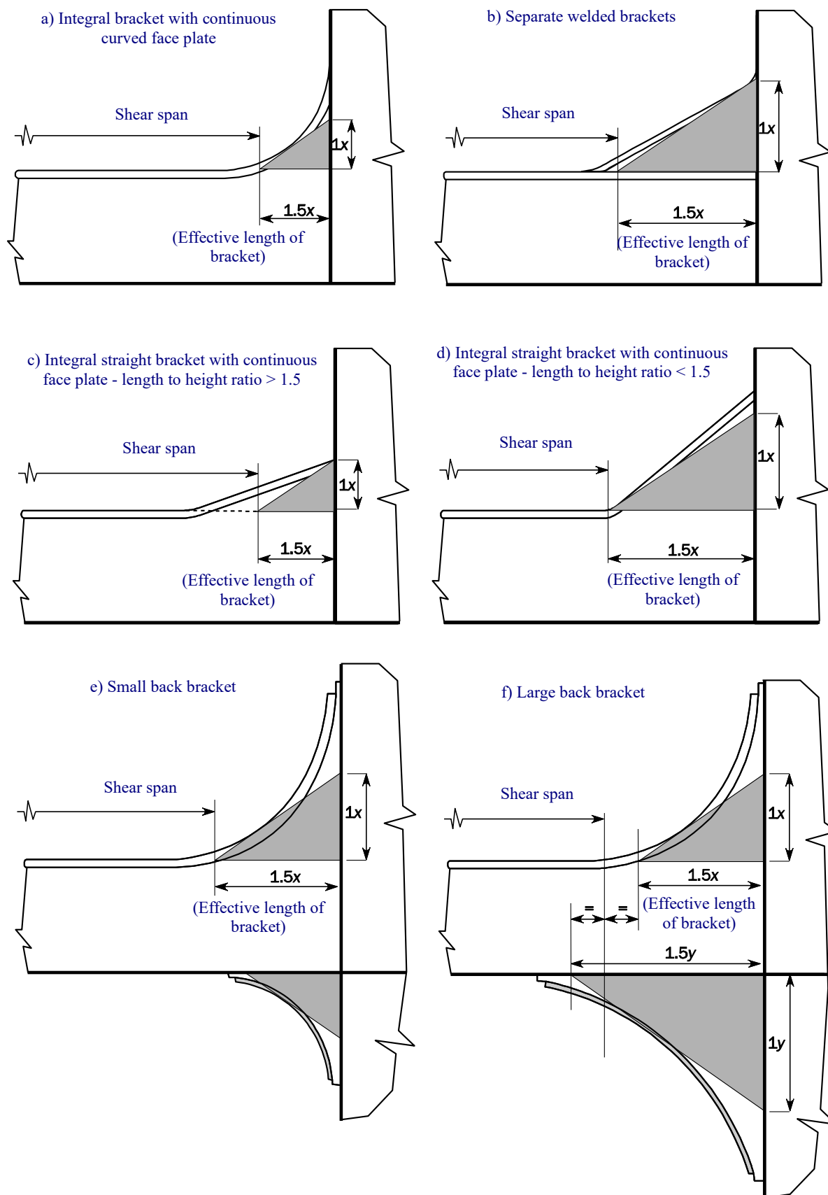
Fig. 3.6.1-6 Effective Shear Span of Primary Supporting Member
