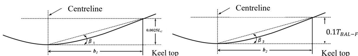
Fig. 4.8.2-1. Measuring Method of b_1 and b_2
