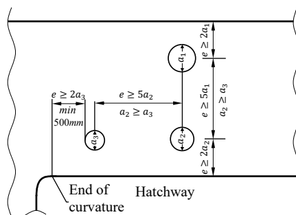
Fig. 5.2.1-6 Intervals between Centers of Holes
