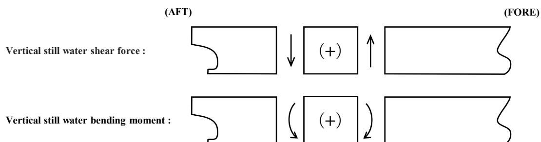
Fig. 3 Descriptive Example 1 of Allowable Values for Vertical Still Water Bending Moment and Vertical Still Water Shear Force (Ships with One to Four Rows of Longitudinal Bulkheads)
