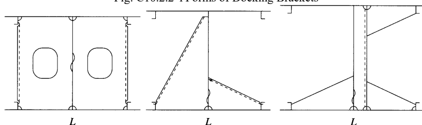
Fig. C10.2.2-1 Forms of Docking Brackets
