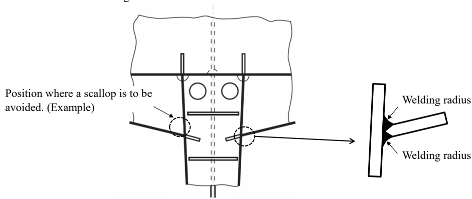
Fig. 11.5.1-5 Connection of Rudder Horn and Hull
