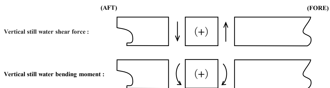
Fig. 2 Descriptive Example 1 of Allowable Values for Vertical Still Water Bending Moment and Vertical Still Water Shear Force (Ships without Longitudinal Bulkheads)
