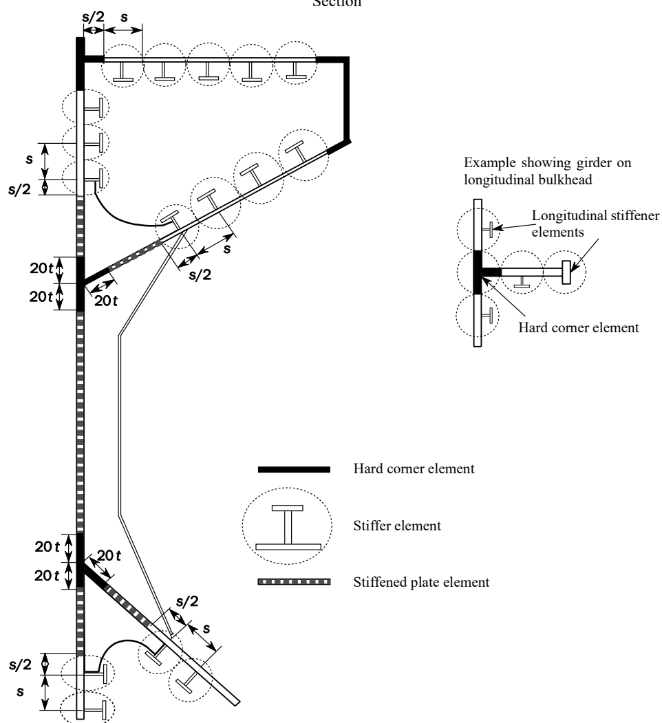
Fig. An3 Examples of the Configuration of Stiffened Plate Elements, Stiffener Elements and Hard Corner Elements on a Hull Section
