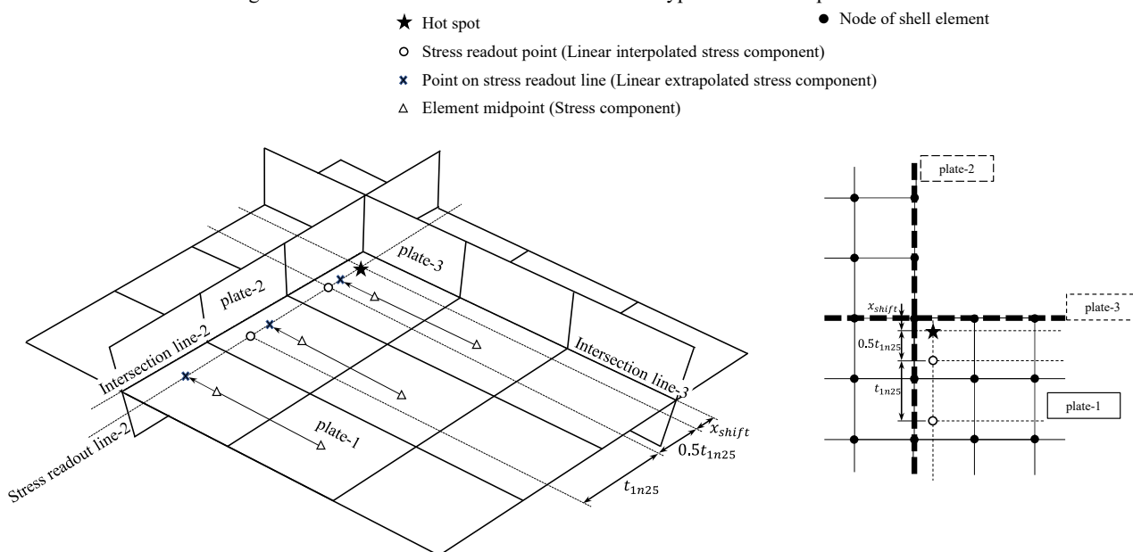
Fig. 9.4.5-3 Location and Readout Method for Type “a1-1” Hot Spot Stress
