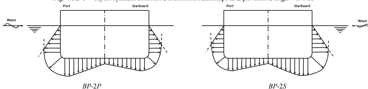
Fig. 4.6.2-6 Hydrodynamic Pressure Distribution Amidships in Equivalent Design Wave BP
