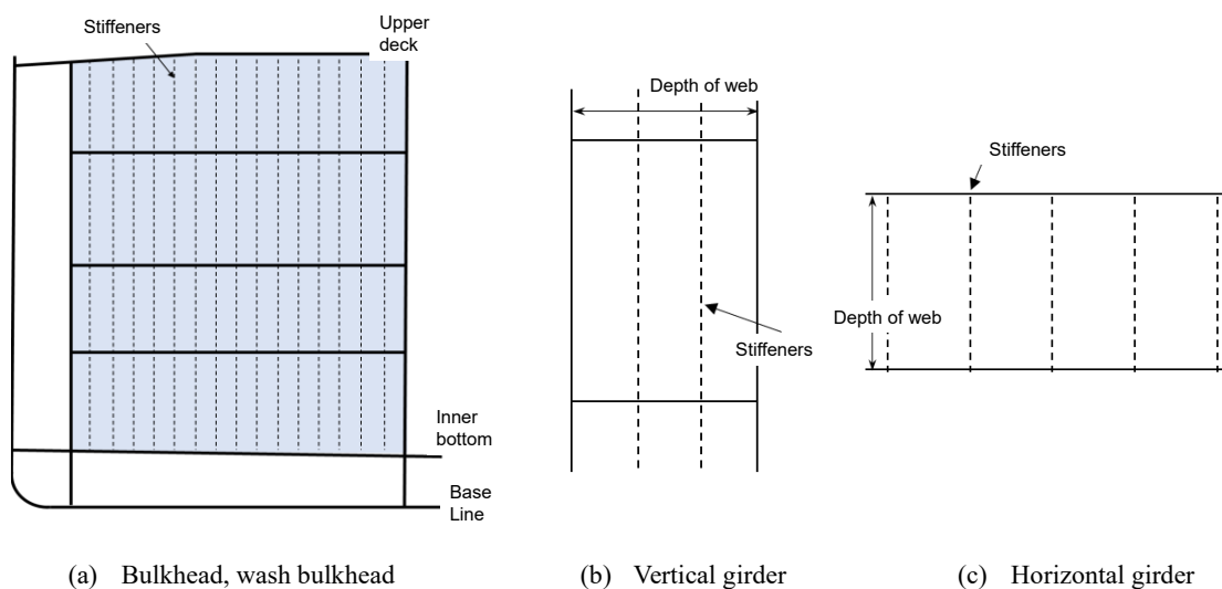
Fig. 10.9.3-2 Stiffened System B
