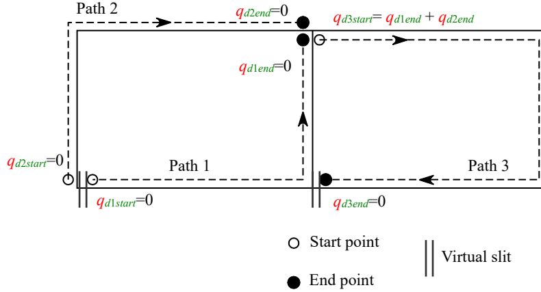
Fig. An2 Calculation of Determinate Shear Flow at Bifurcation
