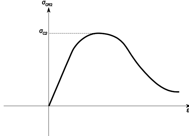
Fig. An9 Load-end Shortening Curve \sigma_{CR2} - \epsilon for Flexural-torsional Buckling
