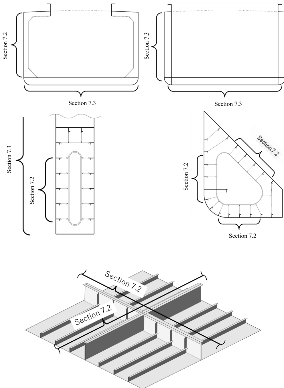
Fig. 7.1.2-1 Examples of Application of 7.2 (Simple Girders) and 7.3 (Double Hulls)
