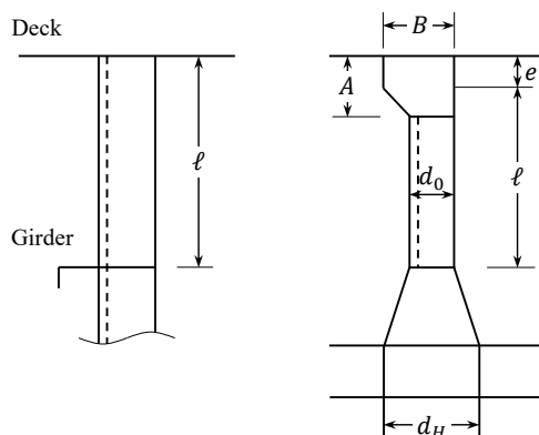
Fig. 7.2.7-2 Measurement of \ell
