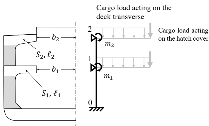
Fig. 7.2.2-1 Web Frames in a Double-Deck Ship with the First Layers and the Second Layers being Single Side
