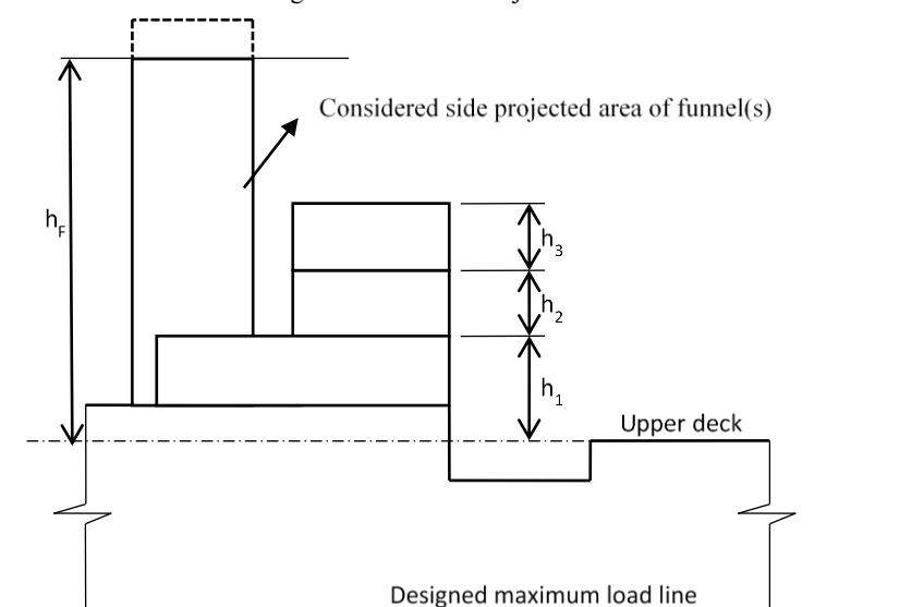
Fig. 14.5.1-2 Side Projected Area of Funnel
