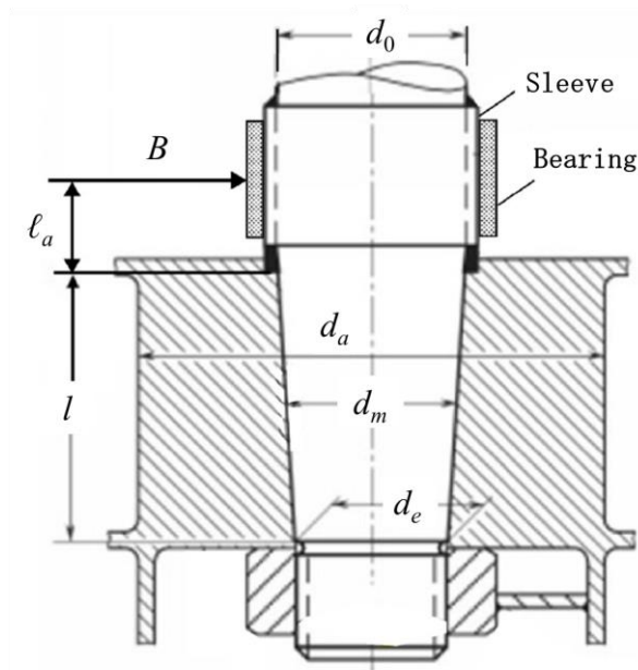
Fig. 13.2.9-1 Pintle Cone Coupling Indicating \ell_a
