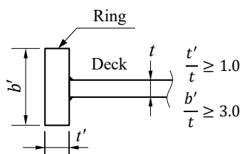
Fig. 5.2.1-5 Reinforcement by Means of Ring
