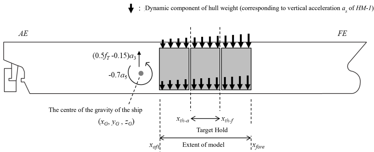
Fig. 8.5.1-1 An Example of Dynamic Component of Hull Weight due to Ship Motions
