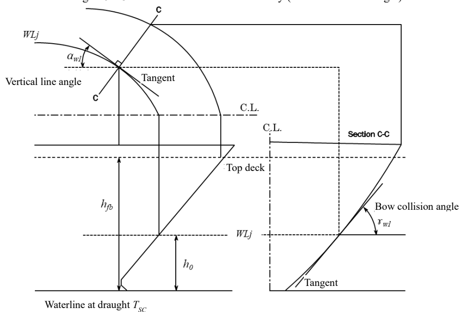
Fig. 4.8.2-3 Definitions of Bow Geometry (Bow Inclination Angle)
