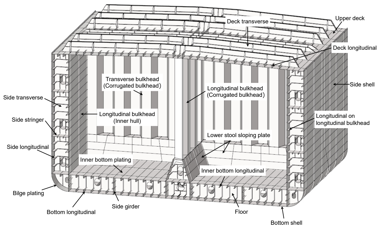
Fig. 1.4.5-9 Chemical Tanker
