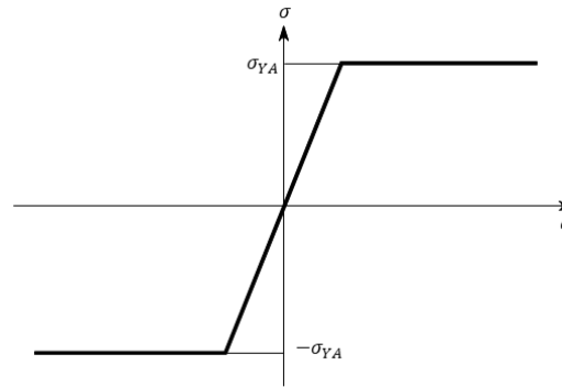
Fig. An7 Load-end Curve \sigma - \epsilon for Elasto-plastic Collapse
