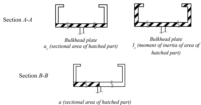
Fig. 5.2.1-4 Where Elliptic Hole and Circular Hole are in Same Cross section
