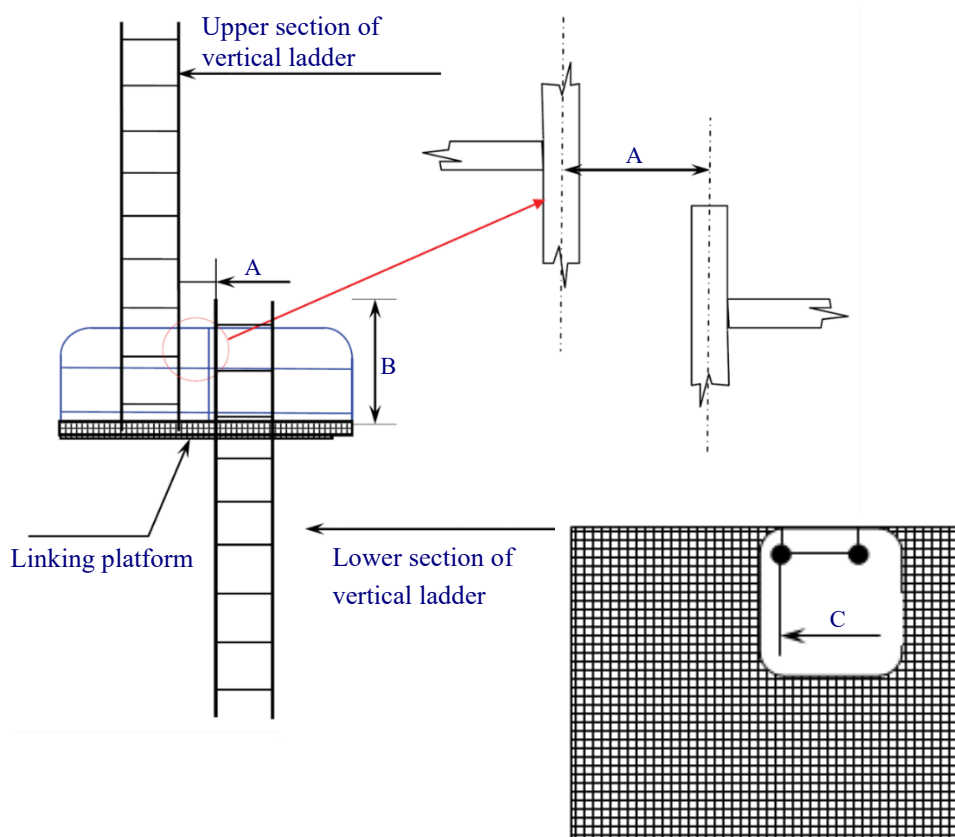
Fig. 14.16.3-2 Vertical Ladder - Ladder Passing through Linking Platform
