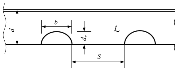
Fig. 5.2.1-2 S , b and d_s of Scallop
