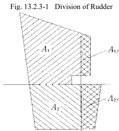
Fig. 13.2.3-1 Division of Rudder
