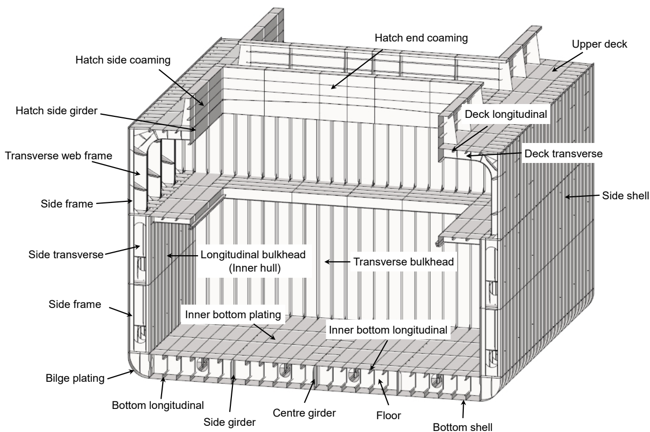
Fig. 1.4.5-5 General Cargo Ship
