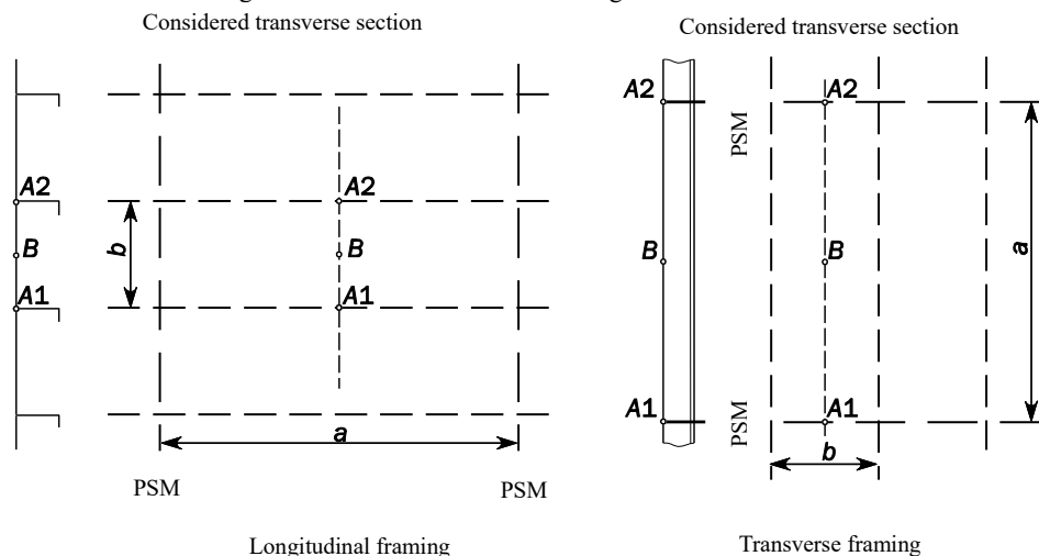
Fig. 3.7.1-7 LCP for Plate Buckling – Hull Girder Stress
