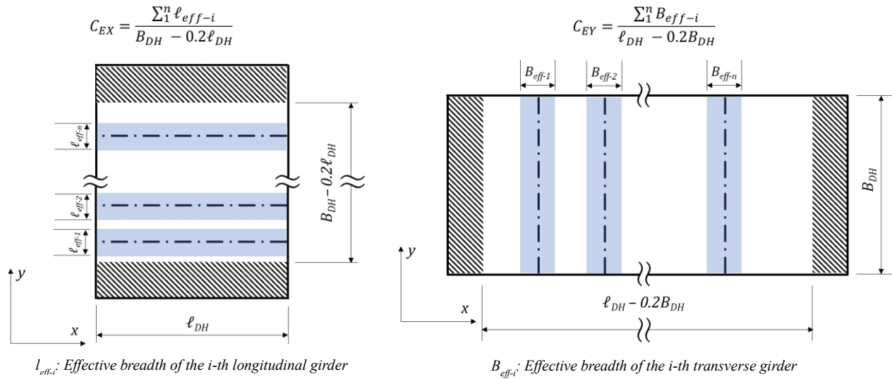
Fig. 7.3.3-1 Effective Breadth Ratio
