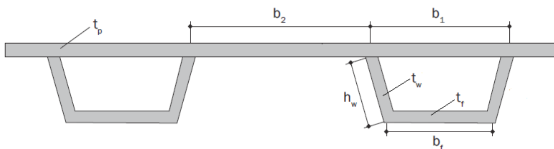
Fig. An3 Dimensions of a U-type Stiffener Cross Section
