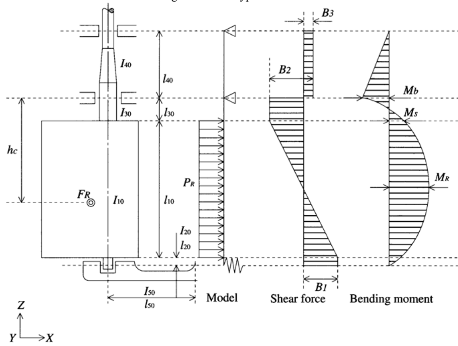
Fig. C13.2.4-2 Type B Rudder
