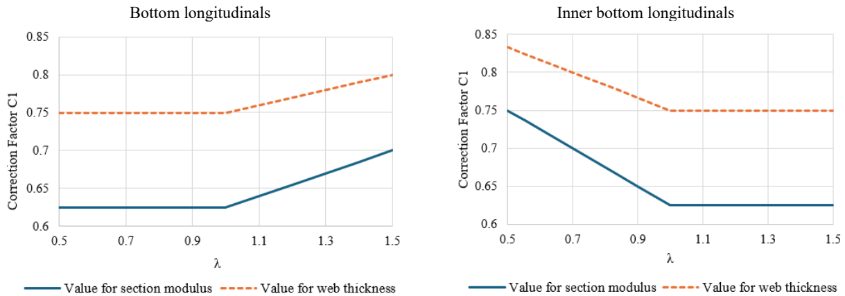
Fig. 6.4.2-2 Correction Factor C_1 for Struts
