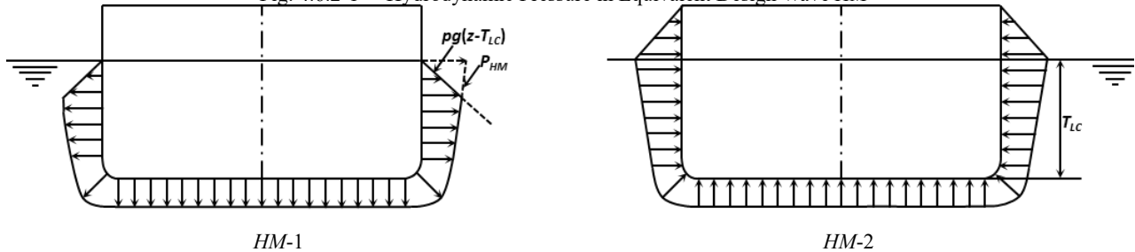
Fig. 4.6.2-1 Hydrodynamic Pressure in Equivalent Design Wave HM
