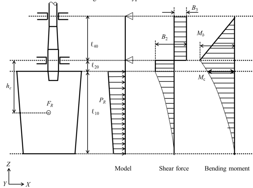
Fig. C13.2.4-3 Type C Rudder
