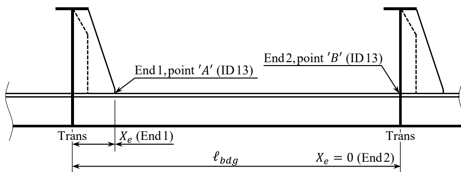
Fig. 9.3.4-1 Definition of Effective Span and \chi_e for Hot Spot
