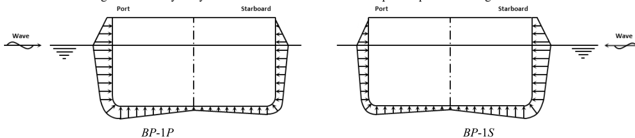
Fig. 4.7.2-5 Hydrodynamic Pressure Distribution Amidships in Equivalent Design Wave BP
