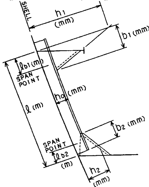
Fig. 10.7.1-1 Corrected Span Length of Stiffener
