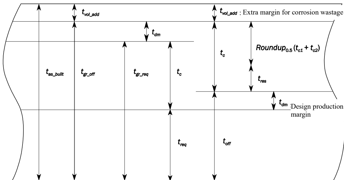
Fig. 3.3.1-1 Net Scantling Approach Scheme
