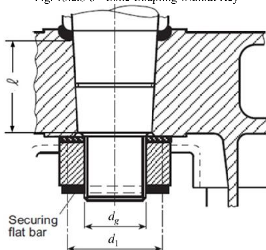
Fig. 13.2.8-5 Cone Coupling without Key
