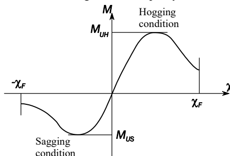
Fig. 5.4.4-1 Bending Moment Capacity vs. Curvature \chi
