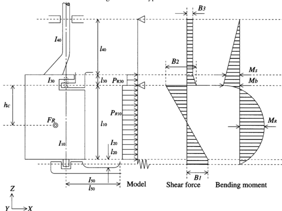
Fig. C13.2.4-1 Type A Rudder
