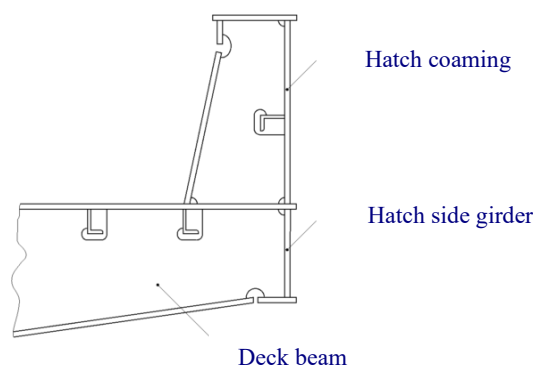
Fig. 14.6.9-2 Example for the Extension of Coaming Plates
