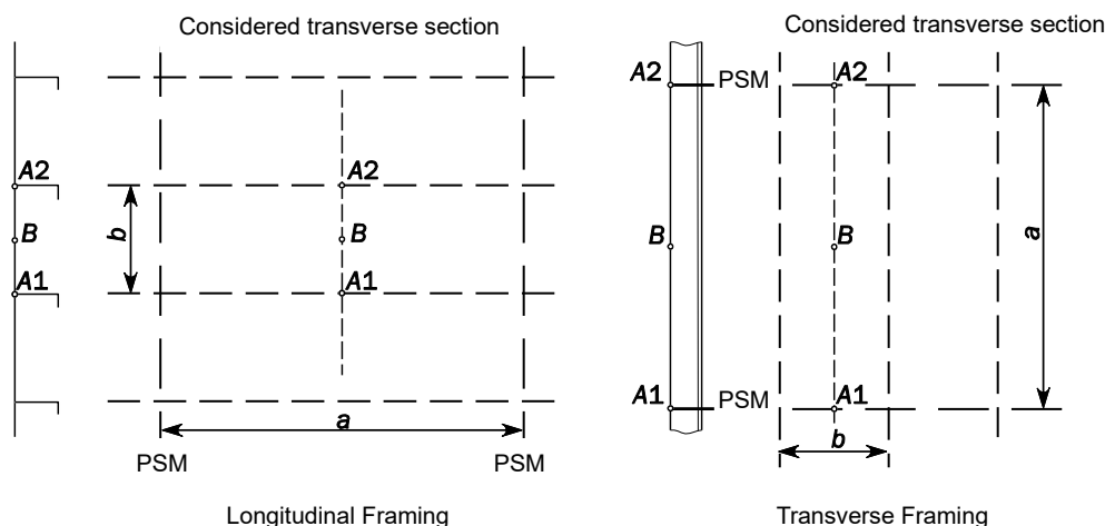
Fig. An5 LCP for Plate Buckling Assessment
