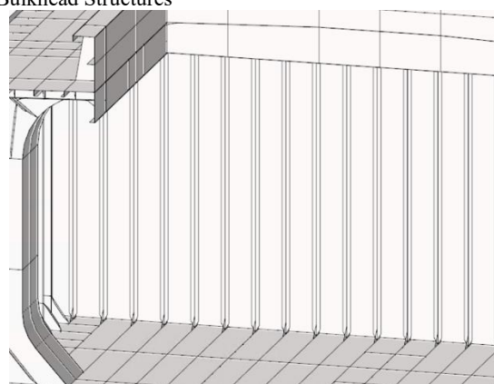
(b) Bulkhead structure supported solely by stiffeners
