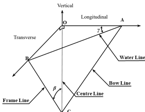
Fig. 4.8.2-2 Inclination Angle of Outer Shell
