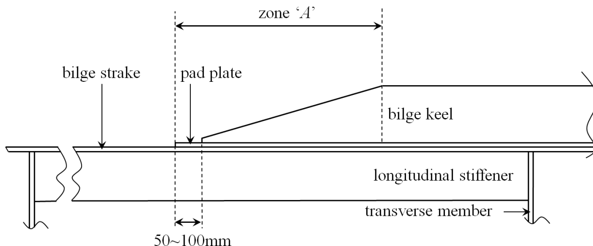
Fig. C10.2.3-2 Example of Supporting Structure of Bilge Keel End by Longitudinal Stiffener
