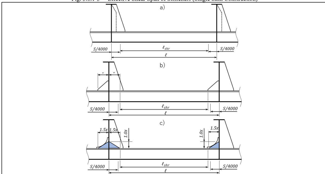
Fig. 3.6.1-3 Effective Shear Span of Stiffeners (Single Skin Construction)
