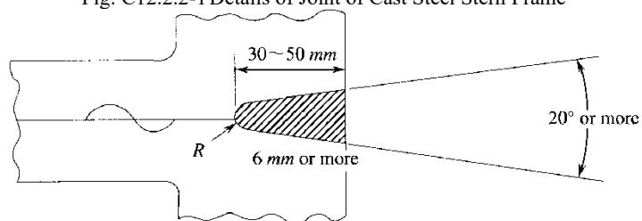
Fig. C12.2.2-1 Details of Joint of Cast Steel Stern Frame
