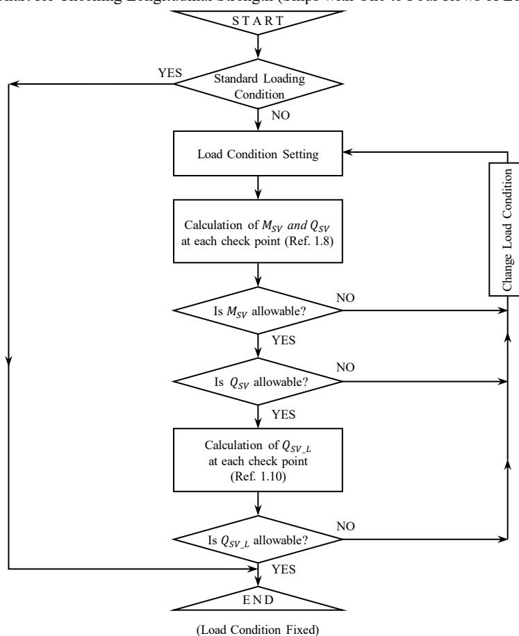
Fig. 6 Flow Chart for Checking Longitudinal Strength (Ships with One to Four Rows of Longitudinal Bulkheads)
