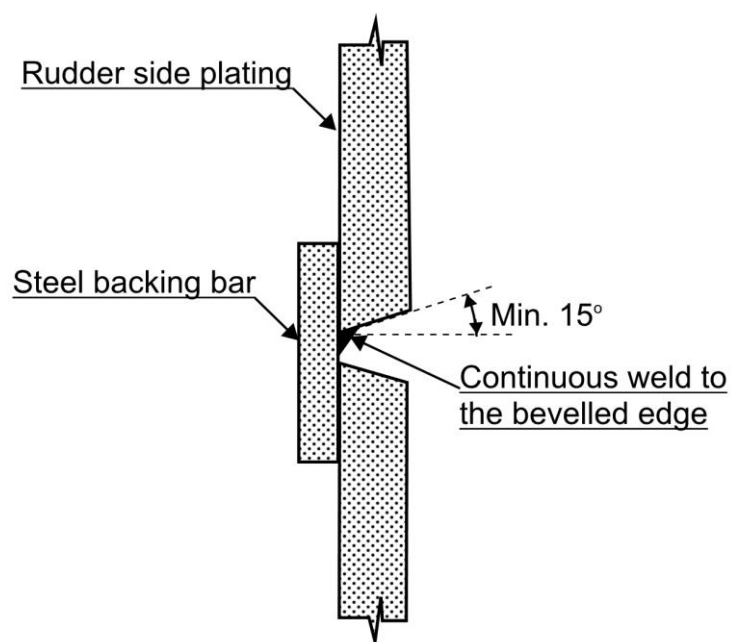
Fig. 13.2.1-3 Use of Steel Backing Bar in way of Full Penetration Welding of Rudder Side Plating
