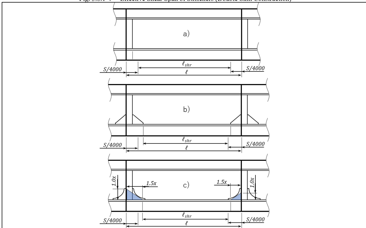
Fig. 3.6.1-4 Effective Shear Span of Stiffeners (Double Skin Construction)
