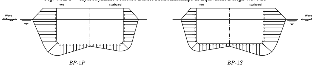
Fig. 4.6.2-5 Hydrodynamic Pressure Distribution Amidships in Equivalent Design Wave BP
