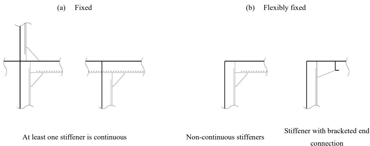
Fig. 6.4.2-1 Examples of Connections
