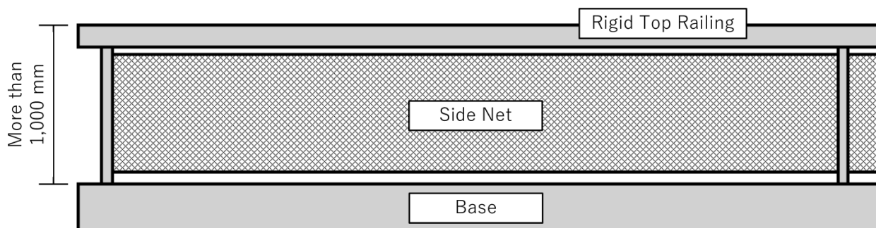
Fig. 14.14.1.1-1 Example of Side Net between Rigid Top Railing and Base of a Means of Embarkation and Disembarkation
