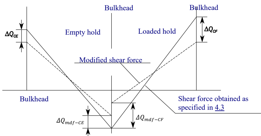
Fig. 5.2.2-1 Shear Force modification, \Delta Q_{mf}
