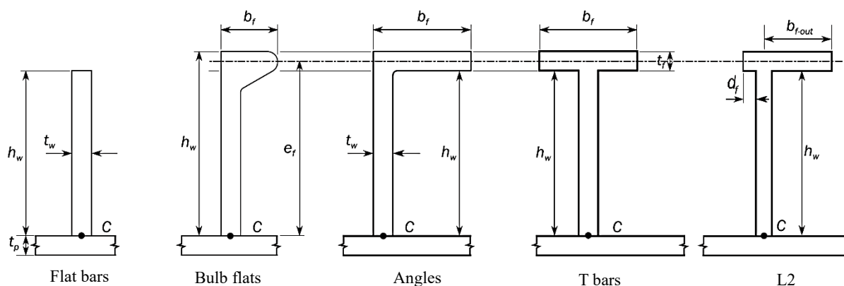
Fig. An2 Dimensions of Typical Stiffener Cross Sections
