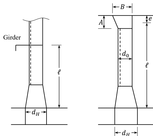
Fig. 7.2.7-3 Measurement of \ell with d_H/d_0 < 2.5
