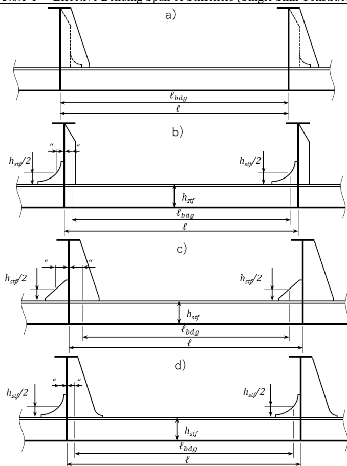
Fig. 3.6.1-1 Effective Bending Span of Stiffeners (Single Skin Construction)
