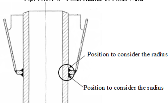
Fig. 11.5.1-6 Fillet Radius of Fillet Weld
