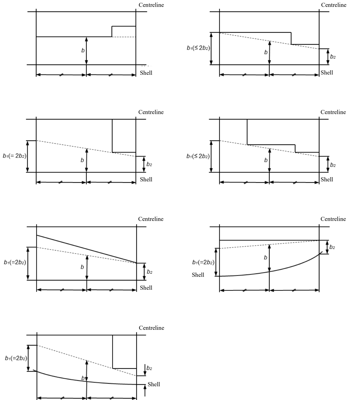
Fig. 2.3.2-3 Examples of Assumed Vertical Plane (In Case of Single Damage Zone)
