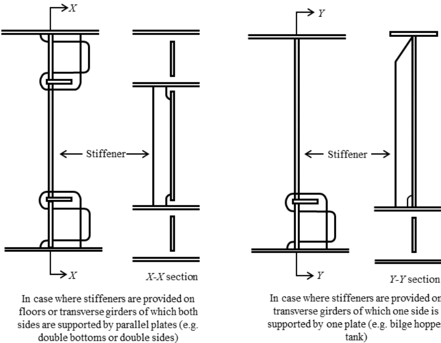
Fig. 10.8.1-1 Examples of Stiffeners Fitted on Floor and Girder
