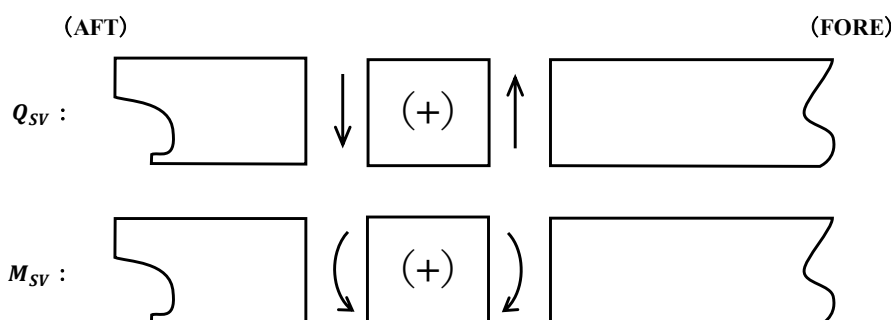
Fig. 7 Sign Conventions for Q_{SV} and M_{SV}
