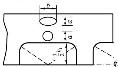
Fig. 5.2.1-4 Where Elliptic Hole and Circular Hole are in Same Cross section
