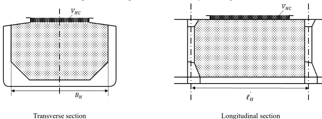
Fig. 4.6.2-8 Cargo Hold Loaded with Dry Bulk Cargo
