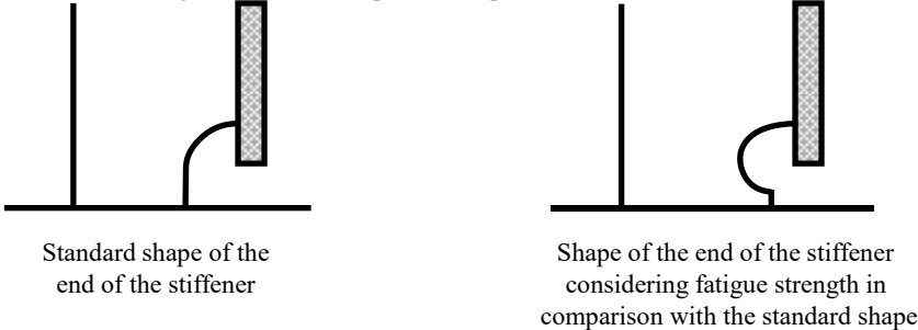
Fig. 10.8.1-2 Examples of Shapes of the Ends of Stiffeners
