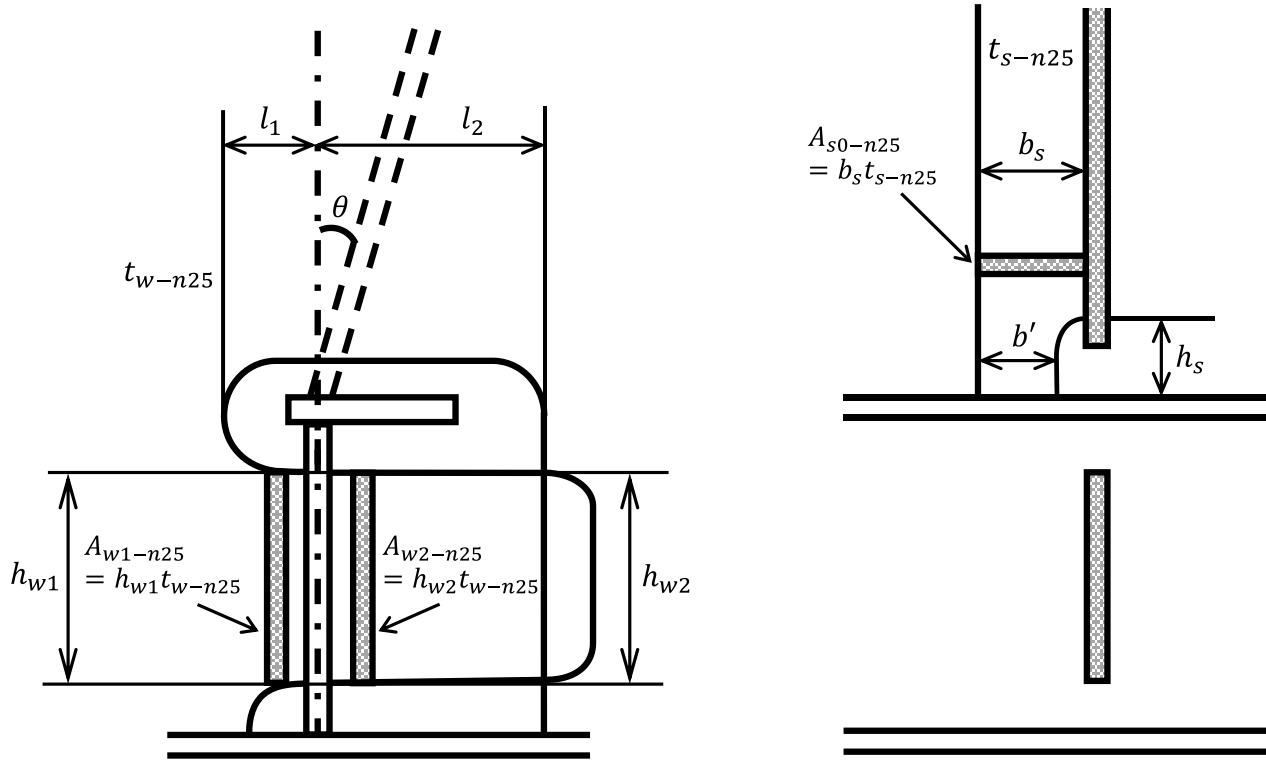
Fig. 10.8.1-3 Definitions of Geometry Parameters Near Slot for Longitudinals
