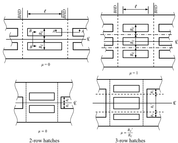
Fig. 5.2.1-3 \ell , b and \mu
