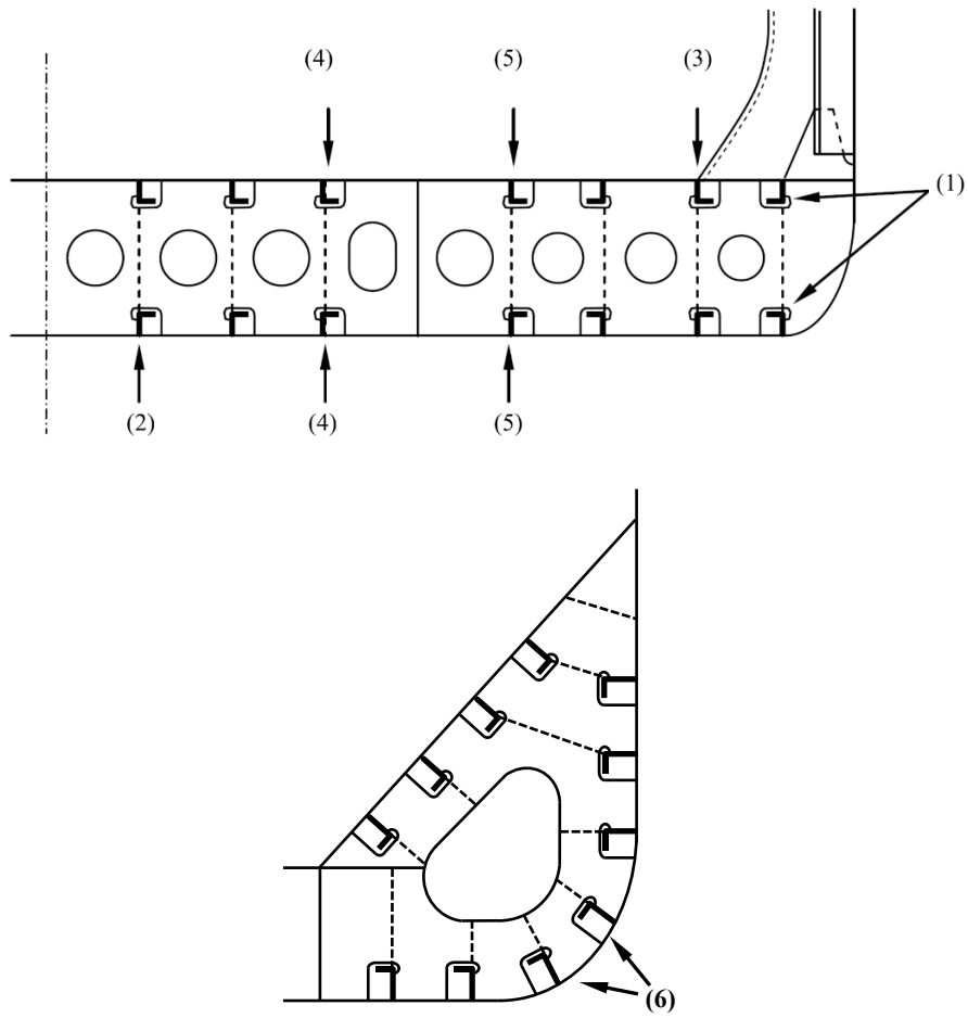
Fig. C3.4.5-1 Typical Locations for Providing Collar Plates
