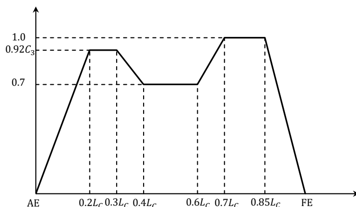
Fig. 4.3.2-3 Coefficient of Distribution along the Ship Length, C_{2p}
