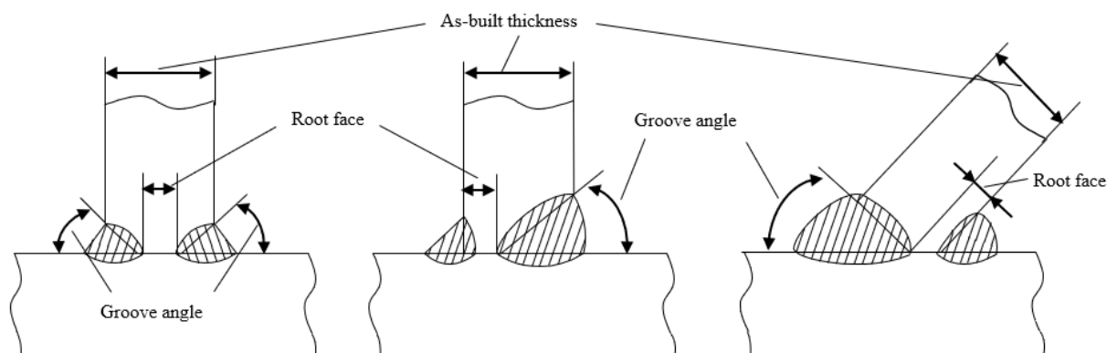
Fig. 12.2.1-3 Examples of partial penetration welds
