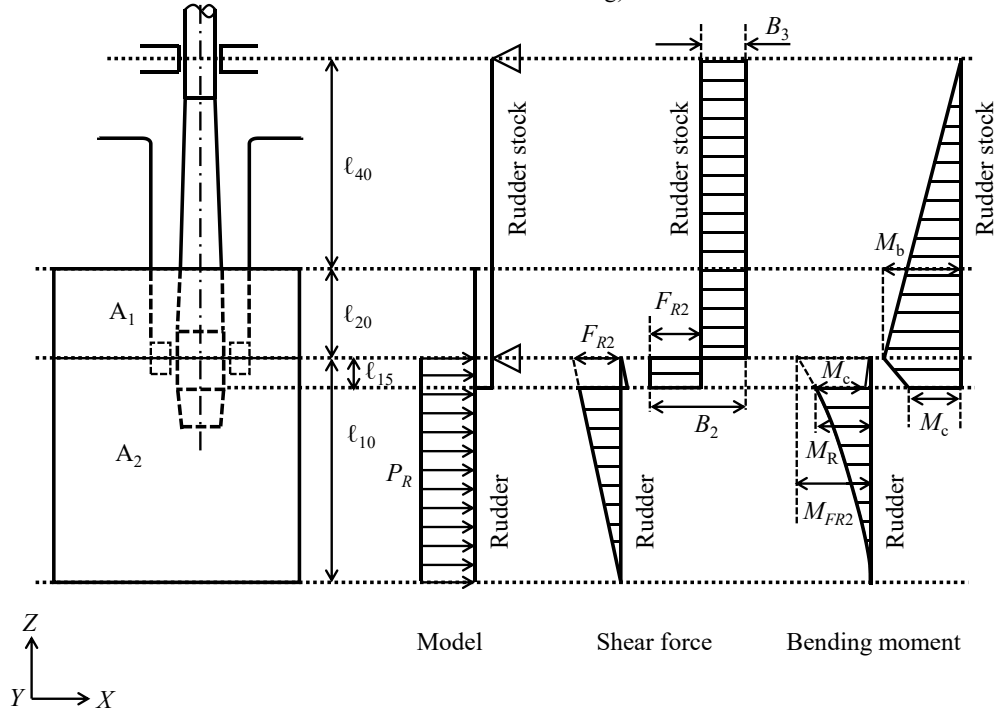
Fig. C13.2.4-7 Type C Rudder with Rudder Trunk Supporting Rudder Stock (Pressure Applied only on Rudder Area below the Middle of Neck Bearing)
