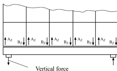
Fig. 4.10.4-1 Vertical Force acting on Hatch Cover
