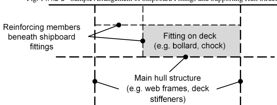
Fig. 14.4.2-2 Sample Arrangement of Shipboard Fittings and Supporting Hull Structures
