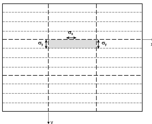
Fig. 14.6.5-1 Determination of the Normal Stress of Hatch Cover Plating \sigma = \max(\sigma_x, \sigma_y)
