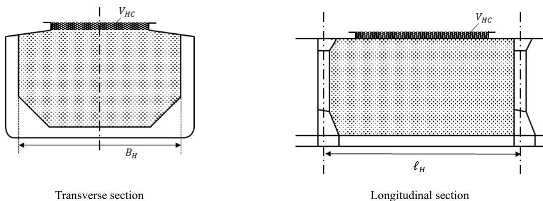
Fig. 4.4.2-2 Cargo Hold Loaded with Dry Bulk Cargo
