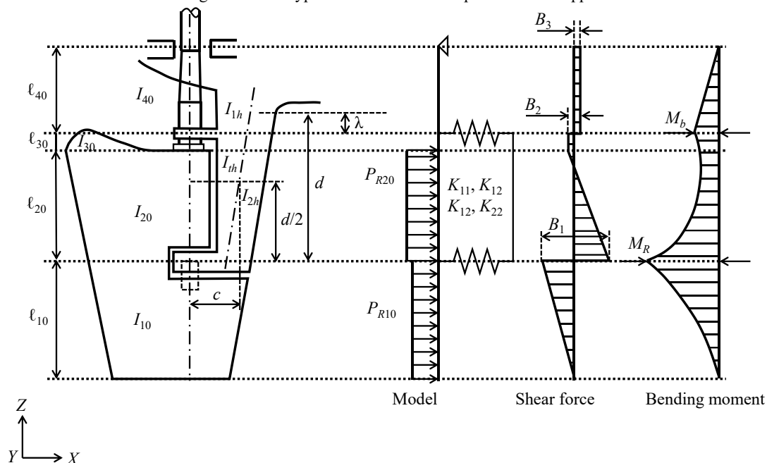
Fig. C13.2.4-8 Type D Rudder with Two-point Elastic Support
