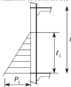
Fig. An6 Definition of Pressure for Vertical Stiffeners
