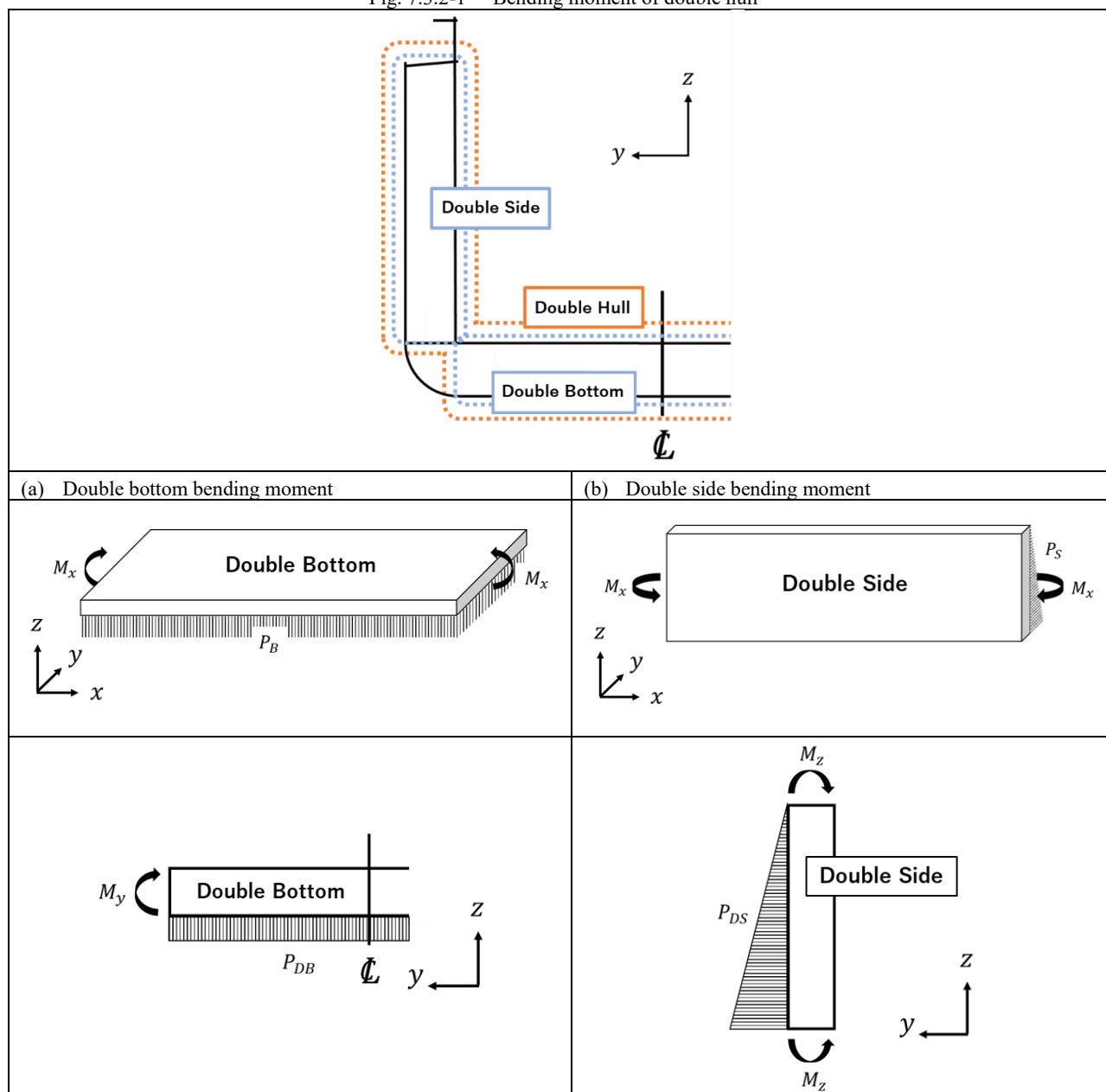
Fig. 7.3.2-1 Bending moment of double hull
