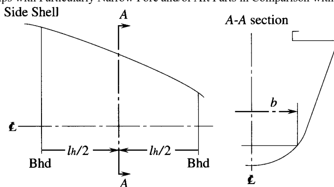
Fig. C6.1.1-3 Ships with Particularly Narrow Fore and/or Aft Parts in Comparison with Breadth Amidships
