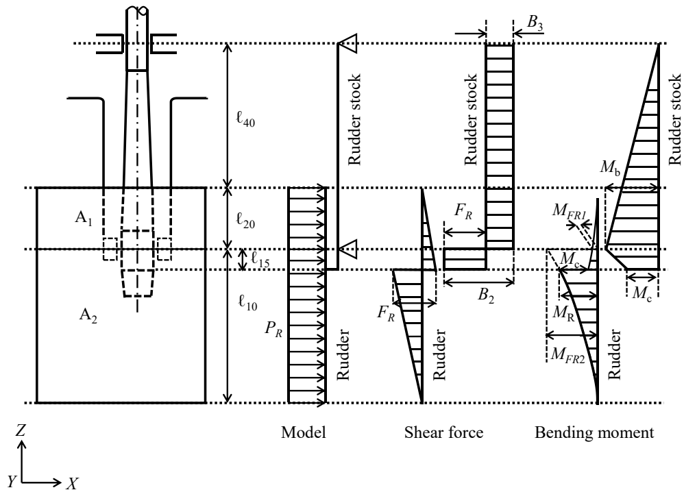
Fig. C3.4.1-6 Type C Rudder with Rudder Trunk Supporting Rudder Stock (Pressure Applied on the Entire Rudder Area)
