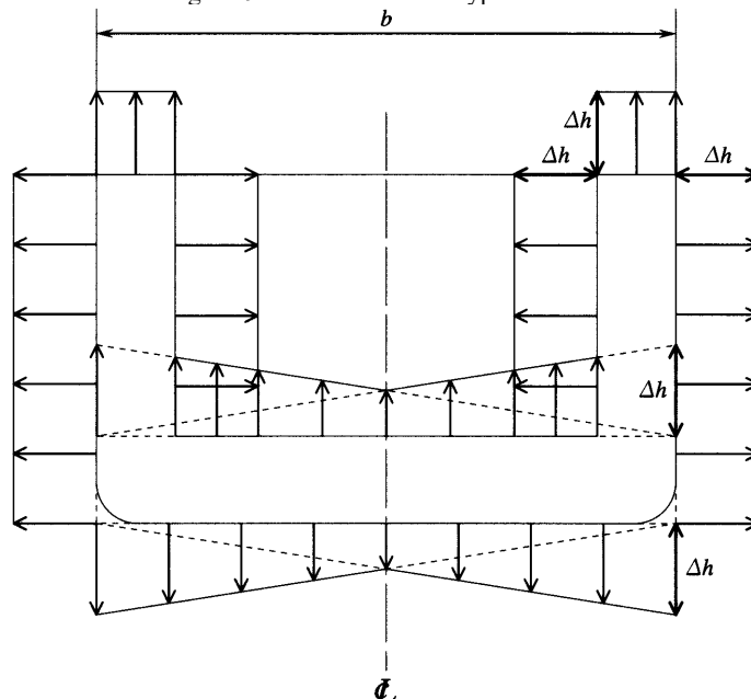
Fig. C29.4.1-2 Case of U-type of Tanks
