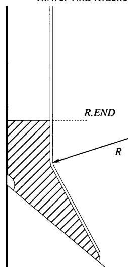
Fig. C31.1.6-1 Lower End Brackets of Hold Frames
