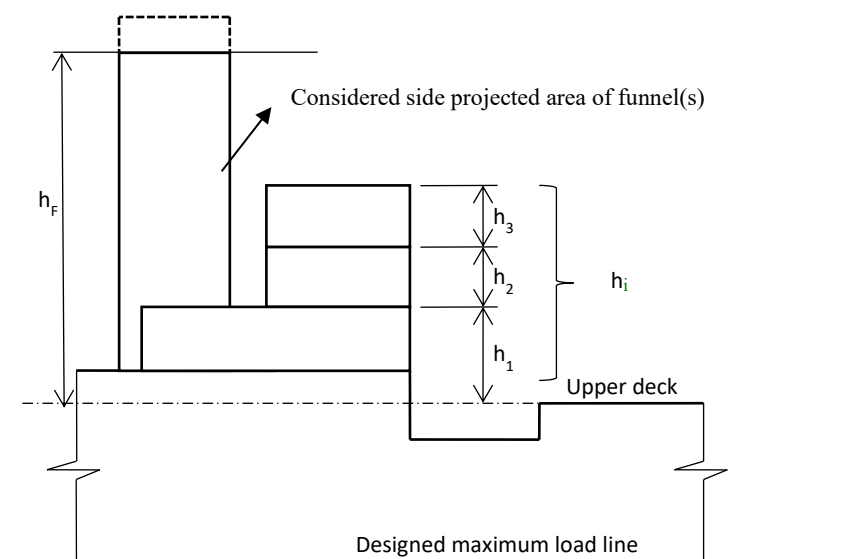
Fig. C27.1 Effective Height
