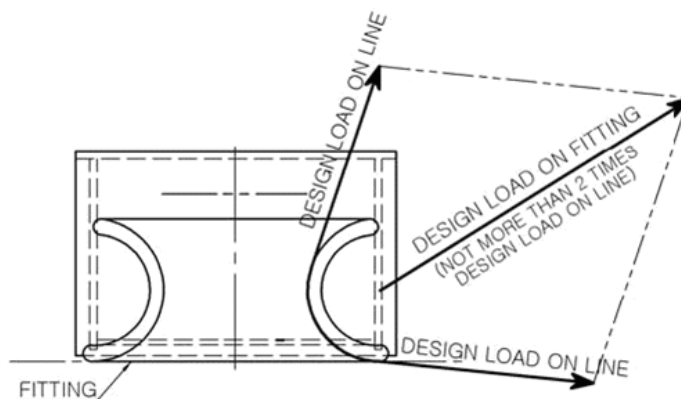
Fig. C27.7 Design Load
