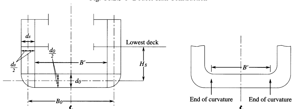
Fig. C6.2.3-1 Double Hull Construction
