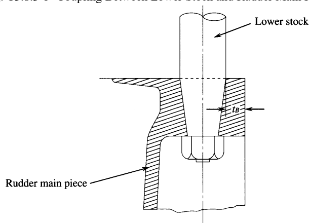
Fig. C3.8.3-1 Coupling Between Lower Stock and Rudder Main Piece
