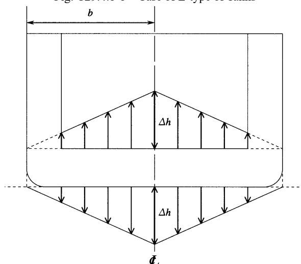
Fig. C29.4.1-1 Case of L-type of Tanks
