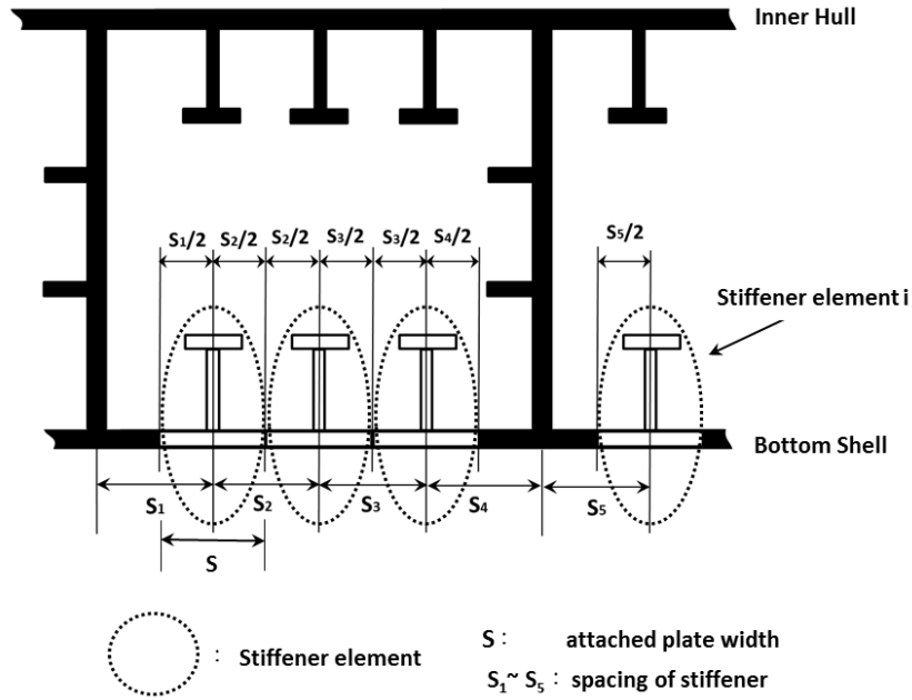
Fig. 2 Method of Dividing Stiffener Element
