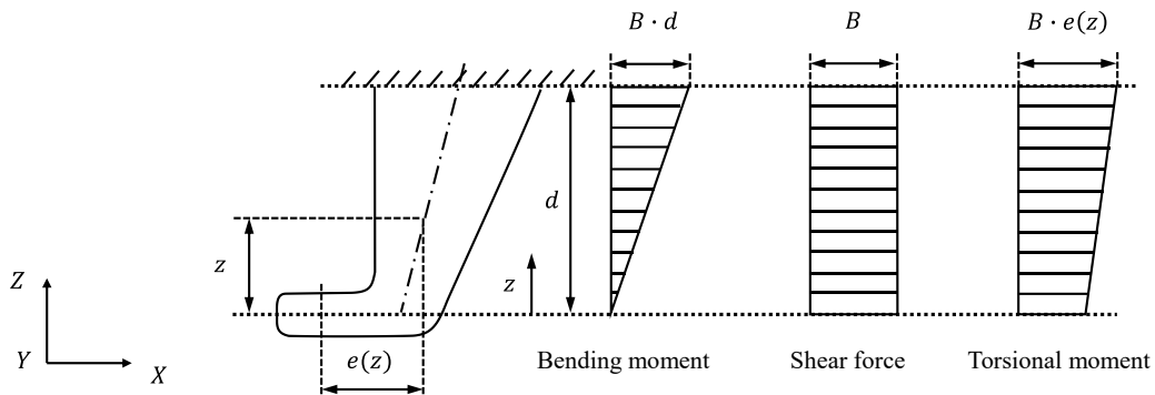
Fig. C2.2.5-1 Geometry of Rudder Horn (Single-point Elastic Support)
