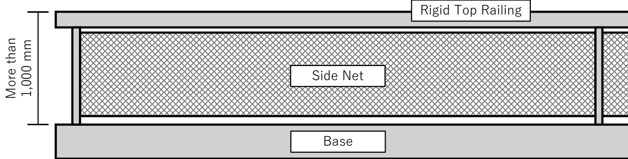
Fig. C23.8.1-1 Example of Side Net between Rigid Top Railing and Base of a Means of Embarkation and Disembarkation
