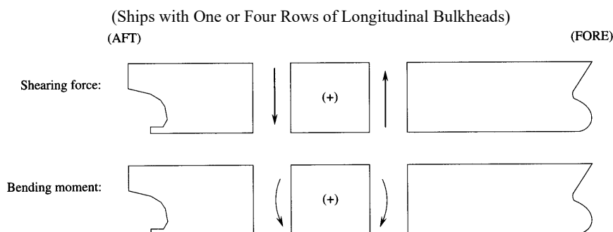
Fig. 3 Descriptive Example 2 of Allowable Values for Vertical Still Water Bending Moment and Vertical Still Water Shear Force
