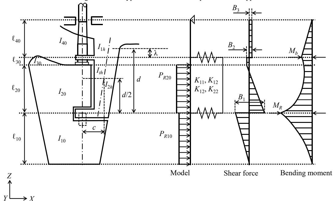
Fig. C3.4.1-8 Type D Rudder with Two-point Elastic Support
