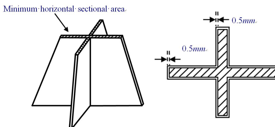
Fig. C29.7.4-1 Example of Supporting Structure (Excluding Top Plate) and the Relevant Minimum Horizontal Sectional Area
