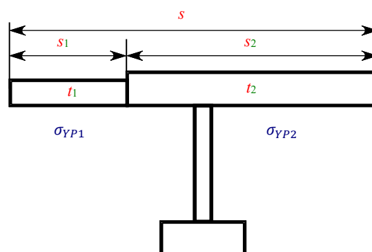
Fig. 5 Element with Different Thickness and Yield Strength
