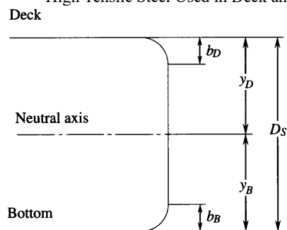
Fig. 2.1 High Tensile Steel Used in Deck and Bottom
