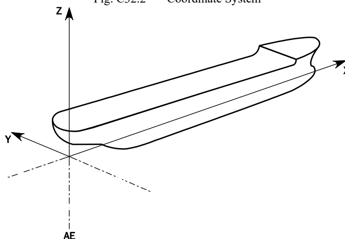
Fig. C32.2 Coordinate System
