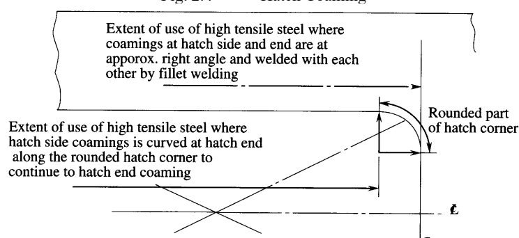
Fig. 2.4 Hatch Coaming
