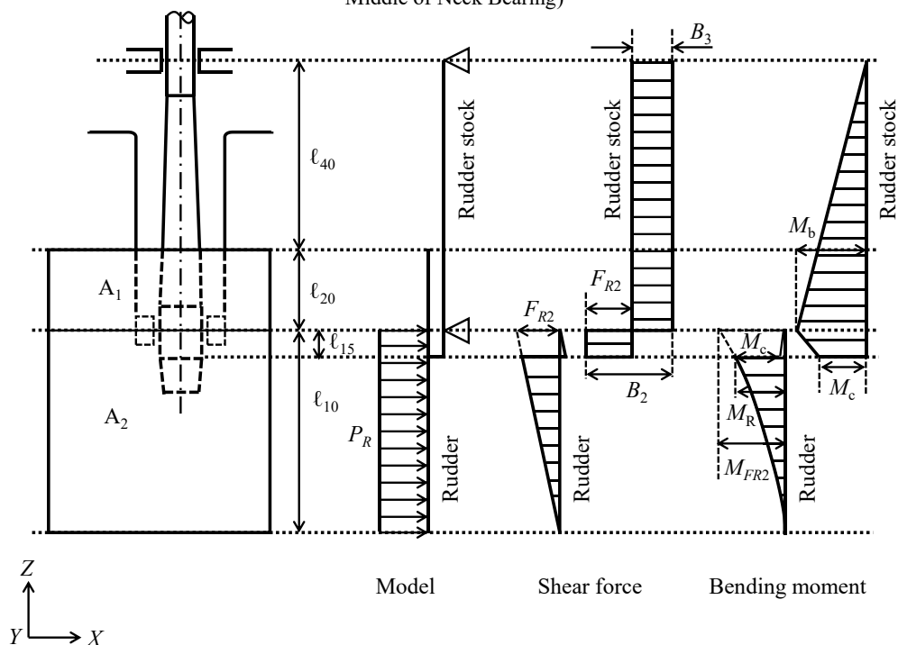
Fig. C3.4.1-7 Type C Rudder with Rudder Trunk Supporting Rudder Stock (Pressure Applied only on Rudder Area below the Middle of Neck Bearing)
