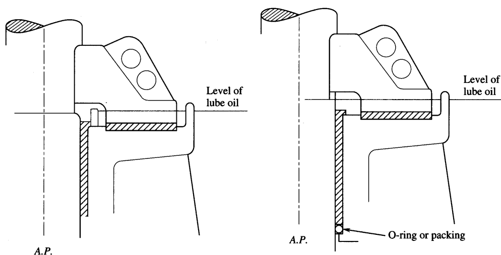
Fig. C3.11.1-1 Rudder Carrier
