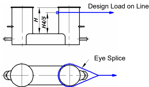
Fig. C27.6 Acting point of the towing force
