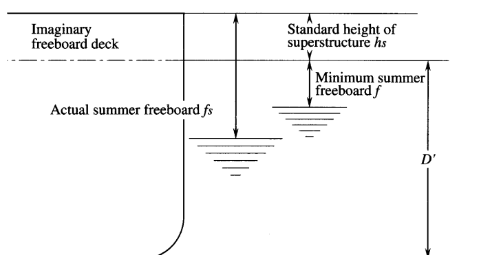
Fig. C1.1.3-2 Ship Having Unusual Large Freeboard
