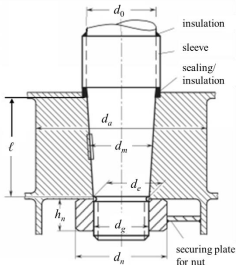
Fig. C3.8 Cone Coupling with Key
