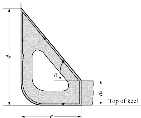
Fig. C31.1 Measurement of l , e , d_0 , d_1 and \beta
