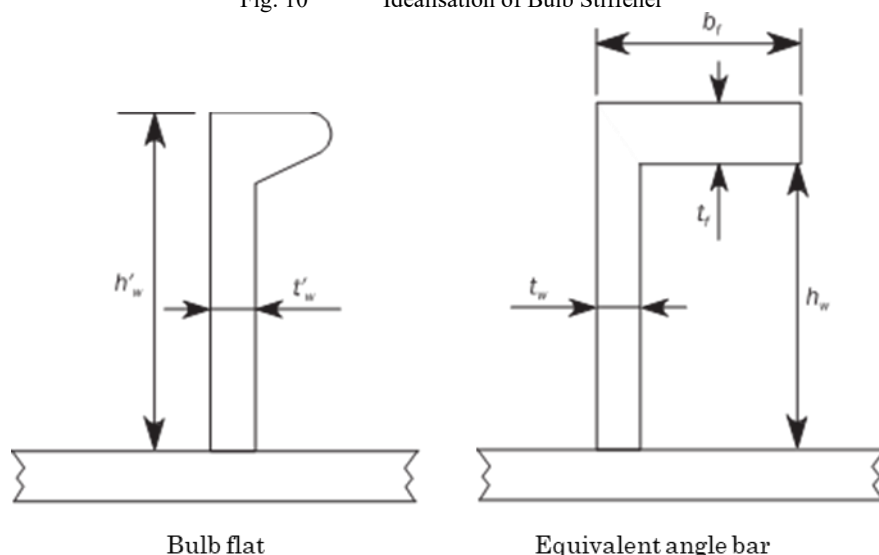
Fig. 10 Idealisation of Bulb Stiffener
