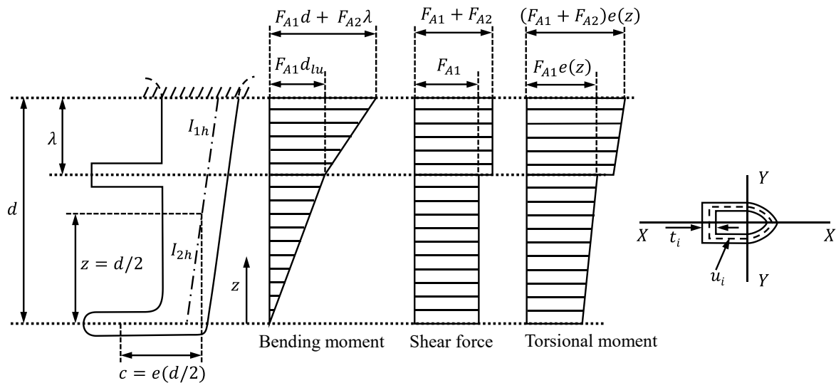
Fig. C2.2.5-2 Geometry of Rudder Horn (Two-point Elastic Support)
