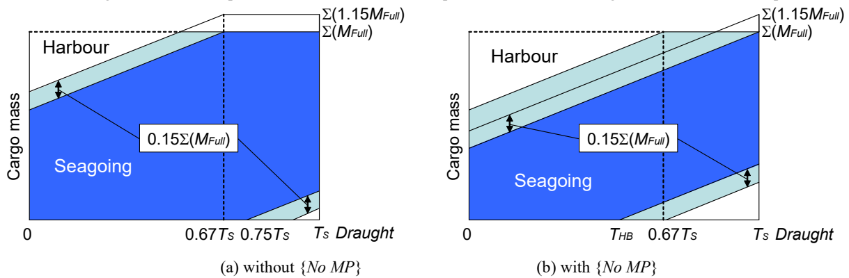
Fig. 6 Example of Mass Curve for BC-A Ships without Block Loading and BC-B or BC-C Ships
