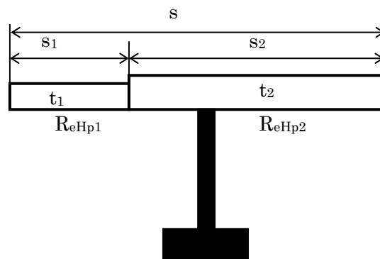
Fig. 10 Element with Different Thickness and Yield Strength
