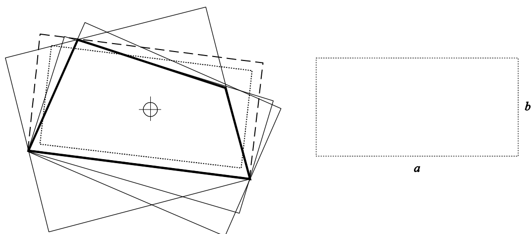
Fig. 5 Approximation of Non Rectangular Elementary Plate Panels
