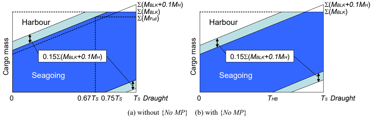
Fig. 5 Example of Mass Curve for BC-A Ships with “Block Loading”
