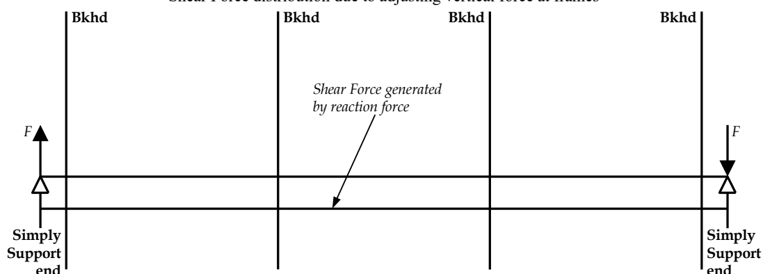
Shear Force distribution due to adjusting vertical force at frames
