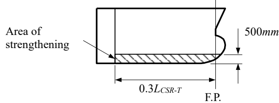
Fig. 8.6.4 Extent of strengthening against bottom slamming
