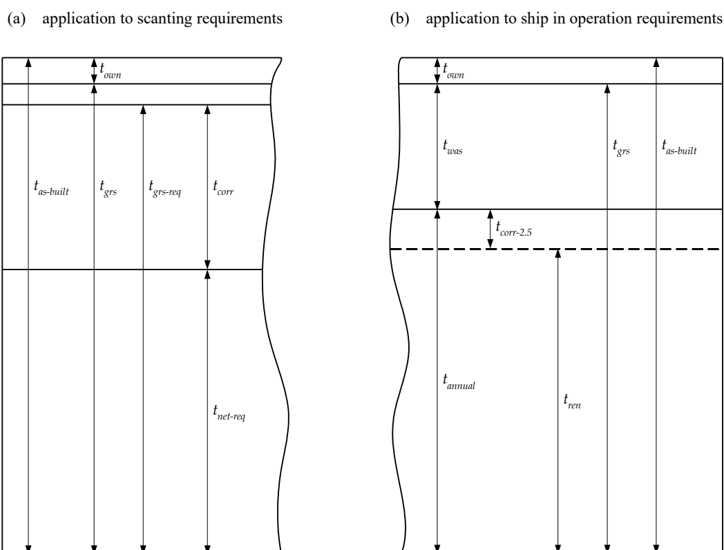
Fig. 2.4.1 Net Thickness Approach for Local Wastage
