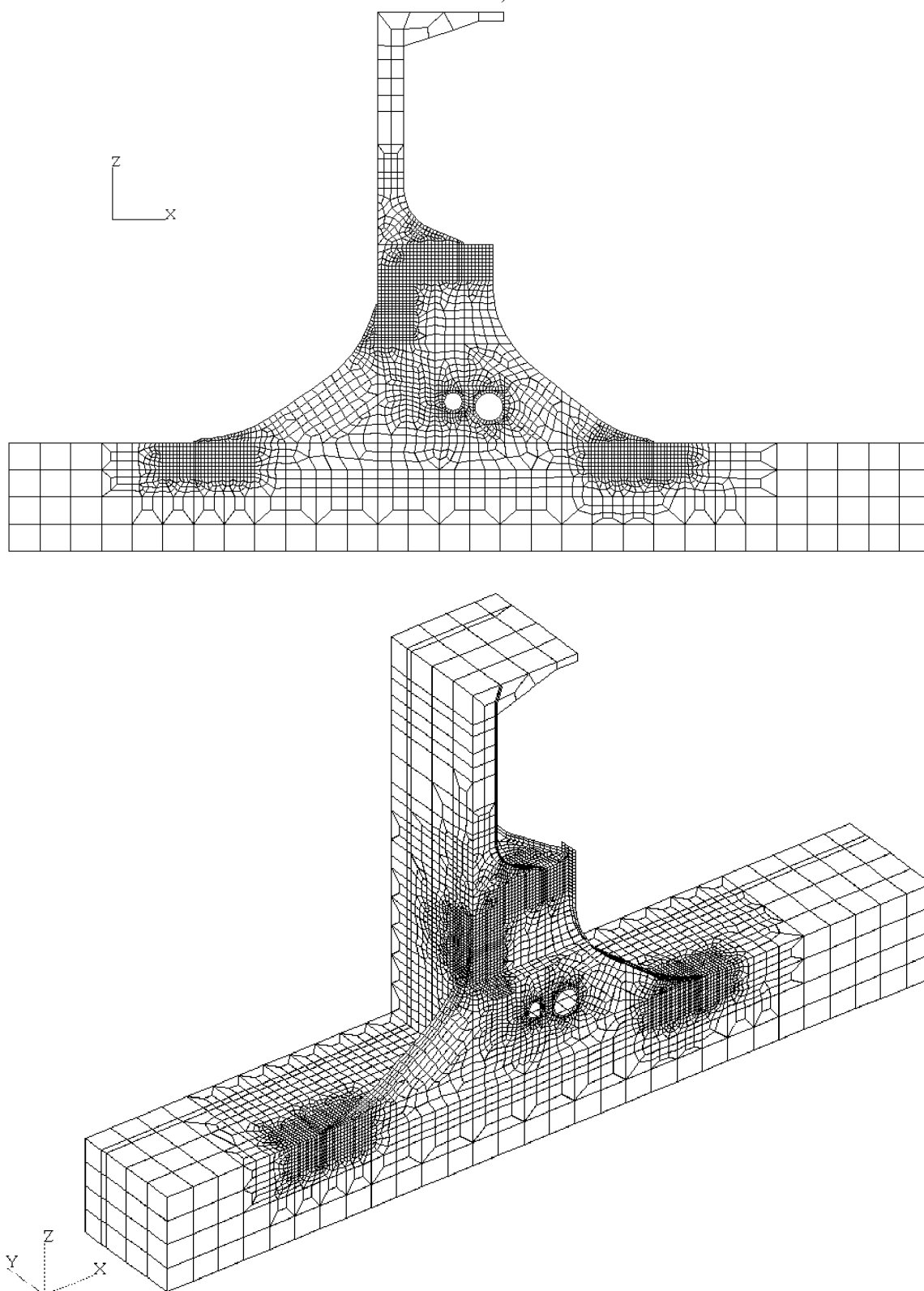
Fig. B.3.12 Sub-Model for the Analysis of Buttress Connections to Bulkhead and Double Bottom Structure (figure shows port half of model)
