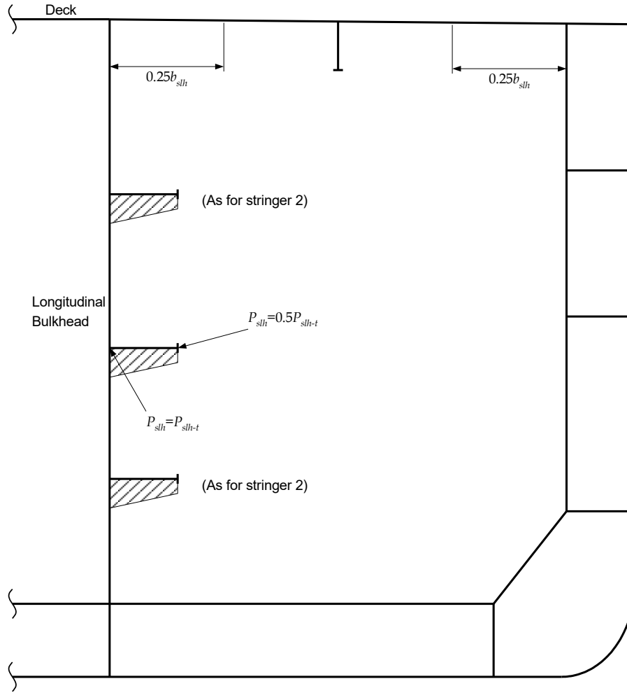
Fig. 7.4.4 Pressure Distribution on Stringers and Longitudinal Girders
