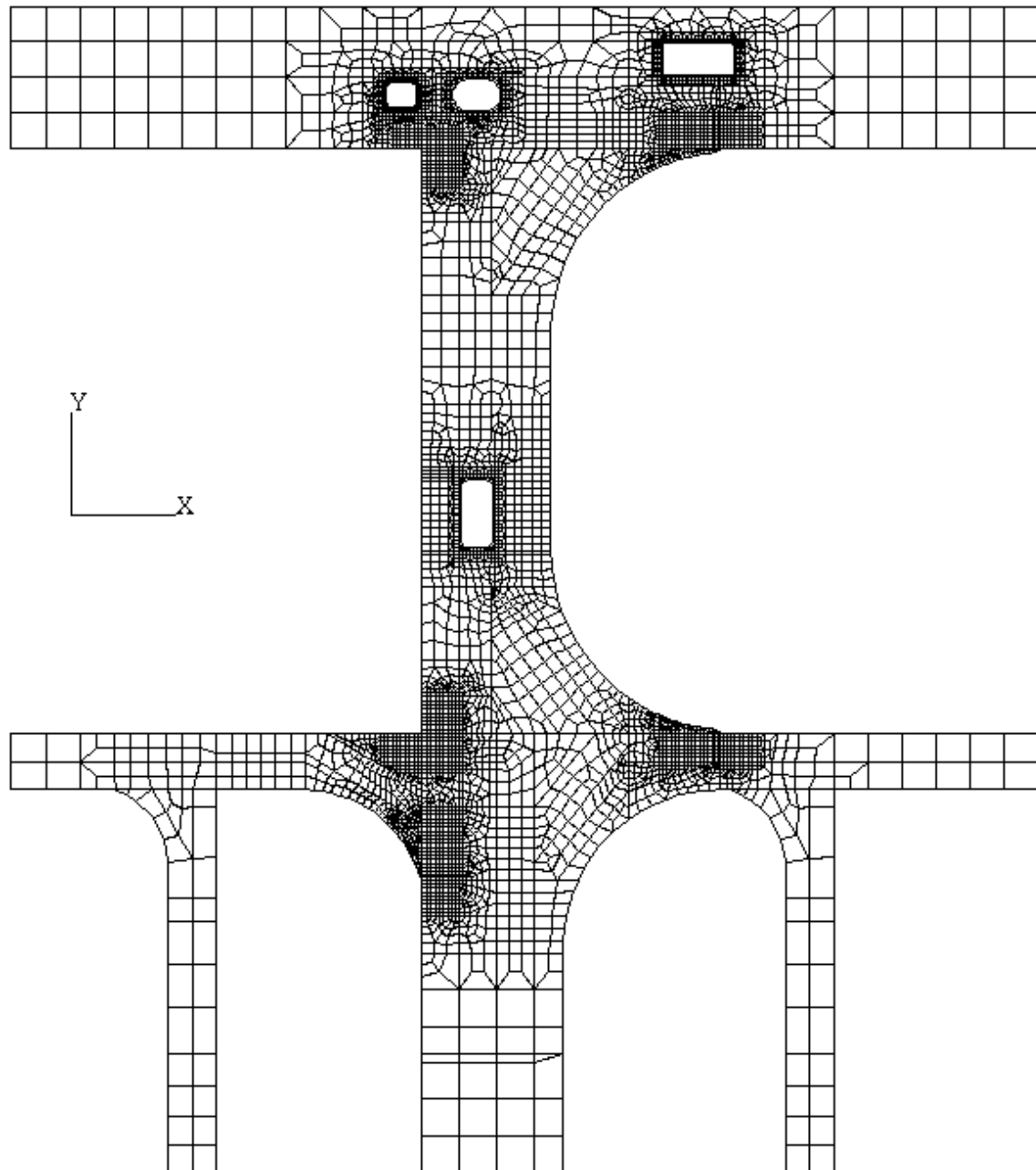
Fig. B.3.11 Finite Element Mesh on Transverse Bulkhead Horizontal Stringer (figure shows port side of model)
