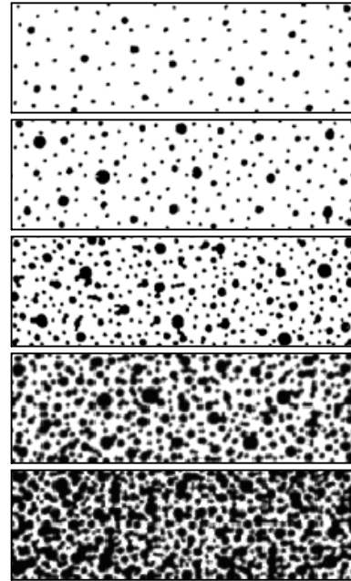
Fig. 12.1.1 Pitting Intensity Diagrams
