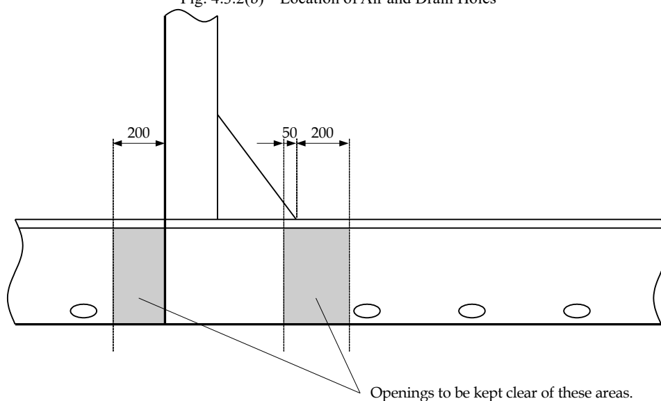
Fig. 4.3.2(b) Location of Air and Drain Holes
