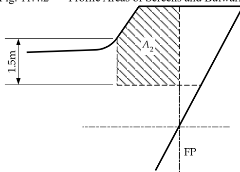
Fig. 11.4.2 Profile Areas of Screens and Bulwarks
