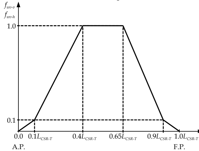
Fig. 7.3.2 Vertical and Horizontal Wave Bending Moment Distribution for Fatigue Strength
