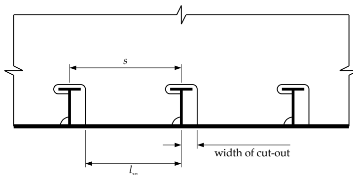
Fig. 6.5.9 Lost Material in Web Cut-outs for Stiffeners
