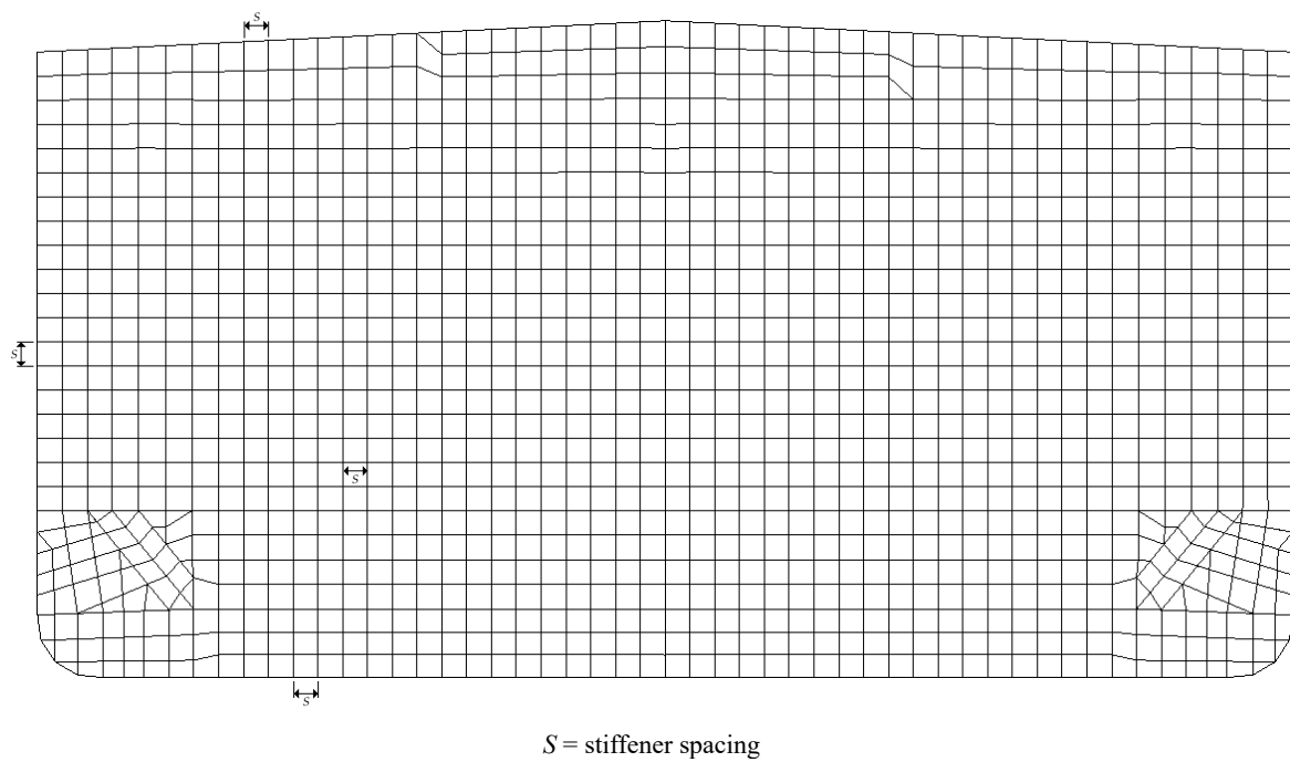
Fig. B.2.3 Typical Finite Element Mesh on Transverse Bulkhead
