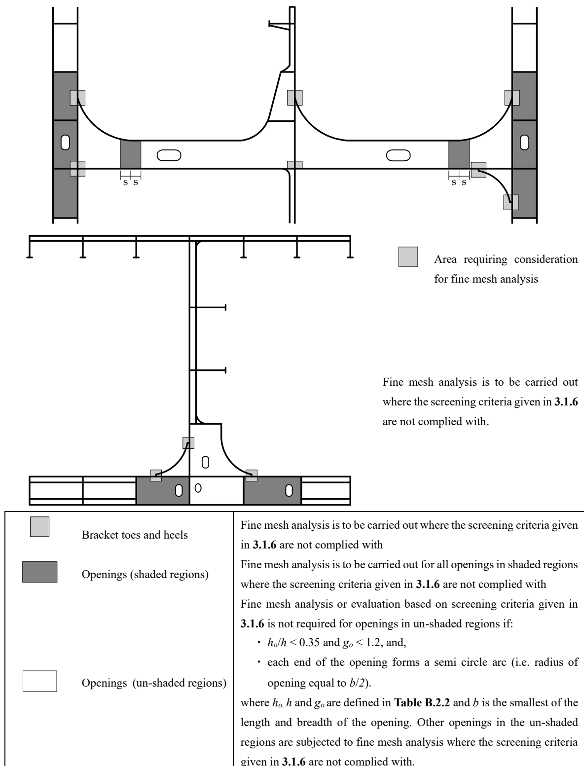
Fig. B.3.2 Areas Requiring Consideration for Fine Mesh Analysis on Horizontal Stringer and Transverse Bulkhead to Double Bottom Connections
