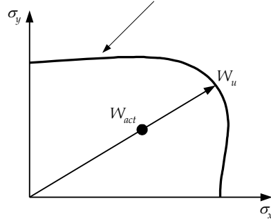
Fig. D.4.1 Definition of Utilisation Factor Example Showing a Bi-Axial Loading Pattern Buckling strength interaction curve
