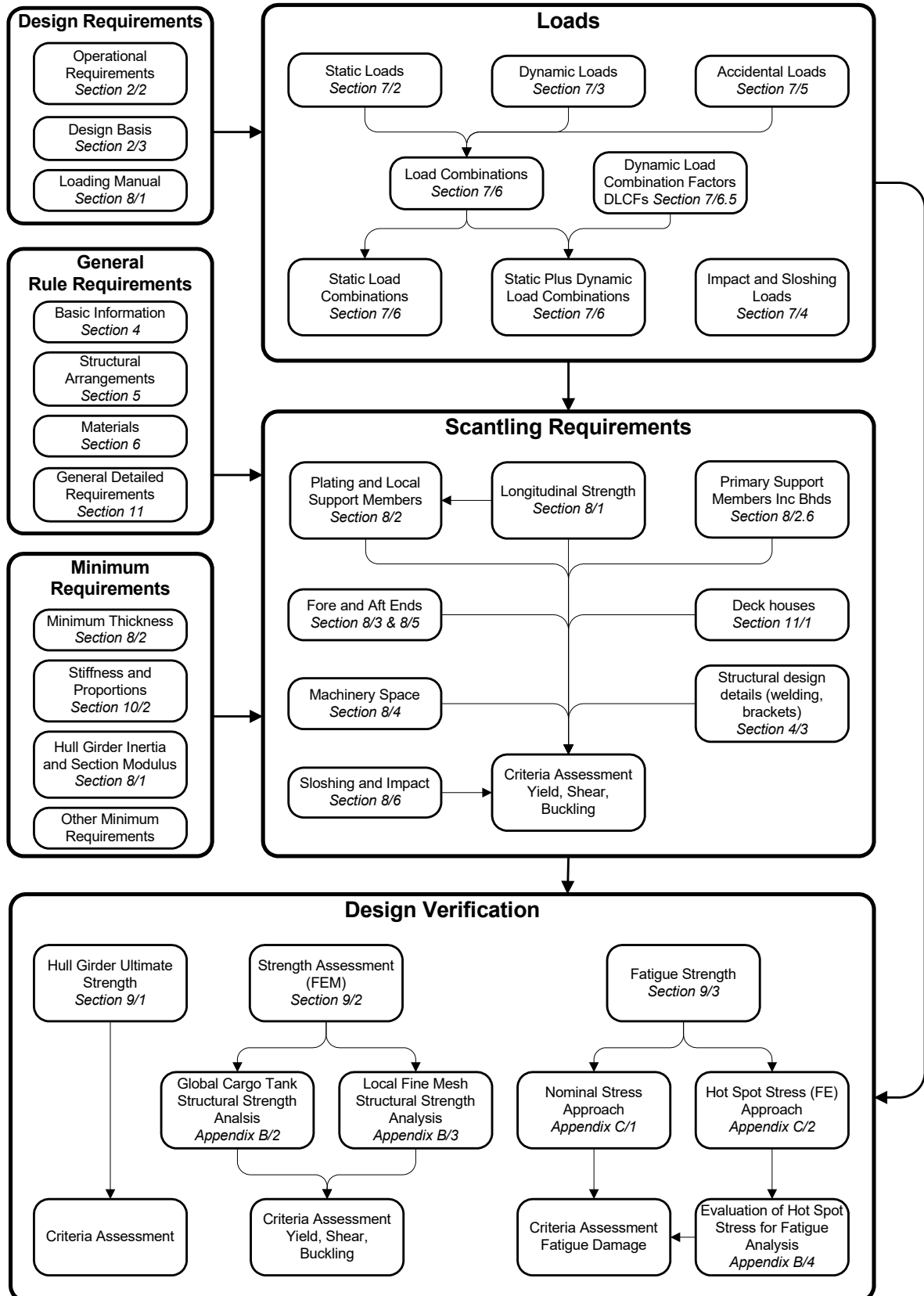
Fig. 2.5.1 Overview of Structural Design Process
