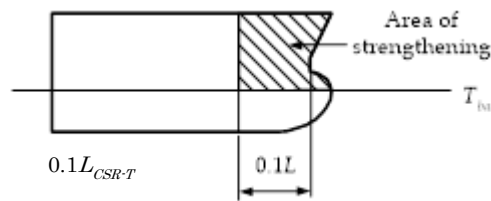
Fig. 8.6.6 Extent of Strengthening Against Bow Impact
