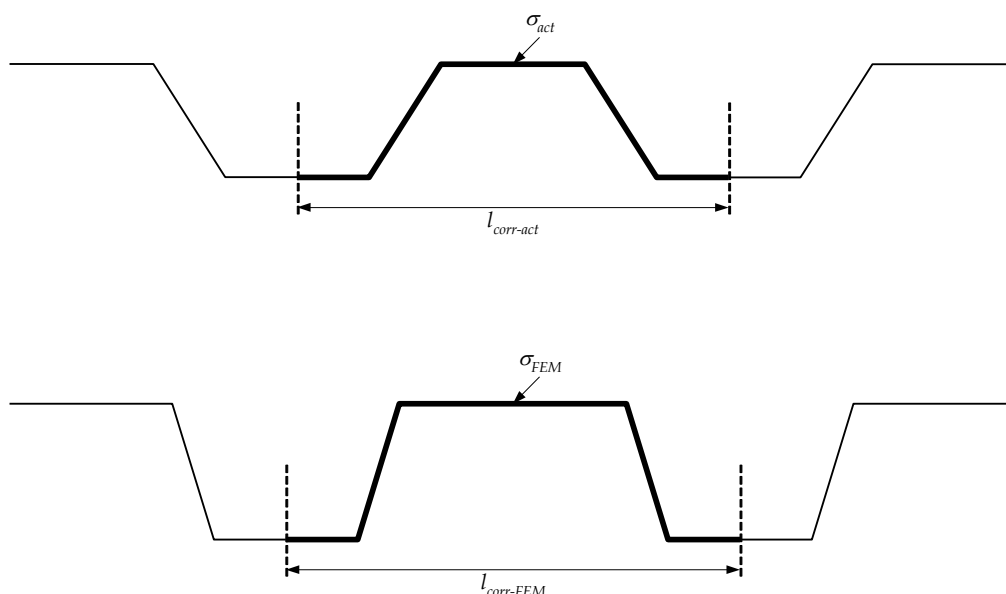
Fig. B.2.15 Axial Bending Stress in Flange Corrugation
