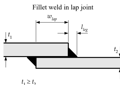
Fig. 6.5.6 Lapped Joints
