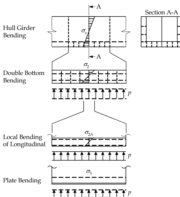
Fig. C.1.3 Definition of Local Stress Components
