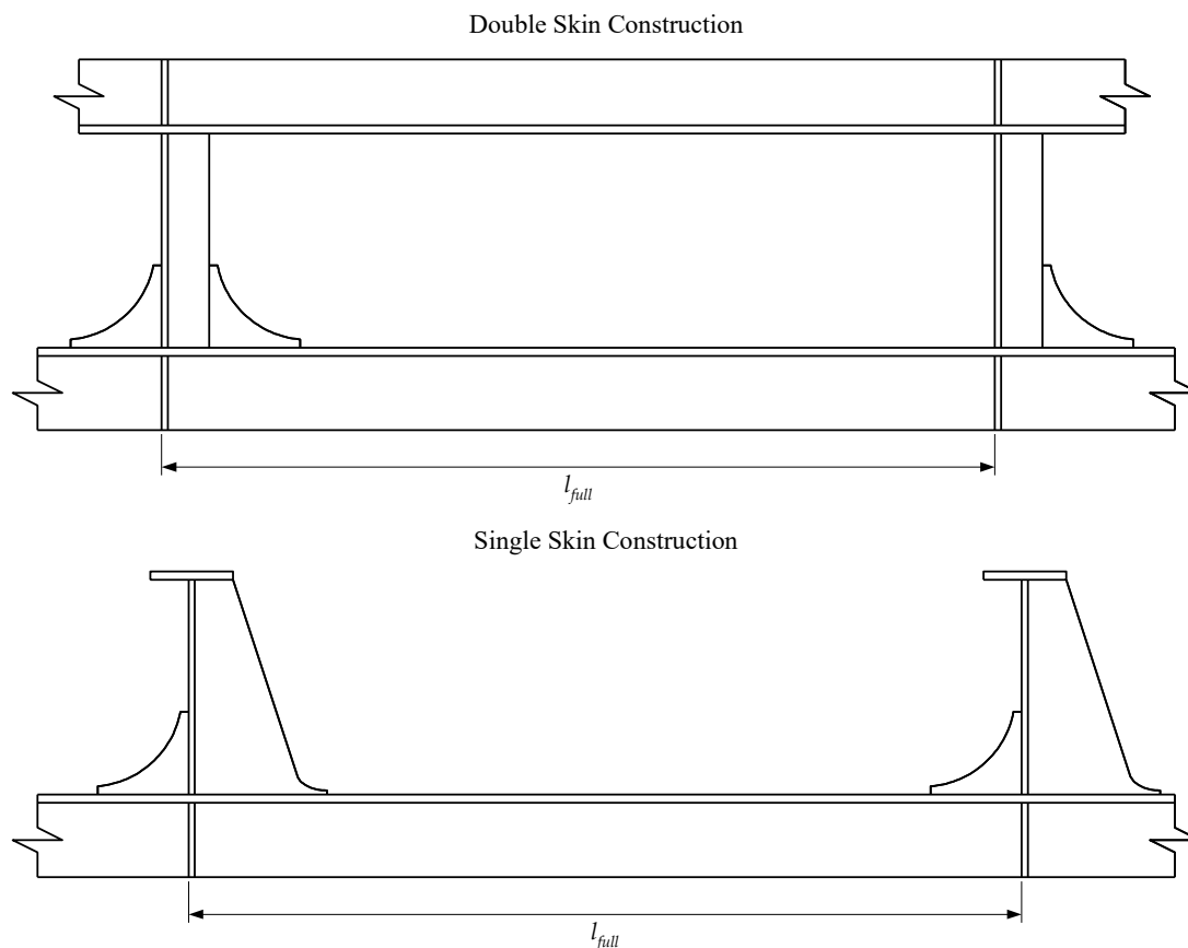
Fig. 3.5.4 Definition of Overall Span of Stiffeners, l_{full}
