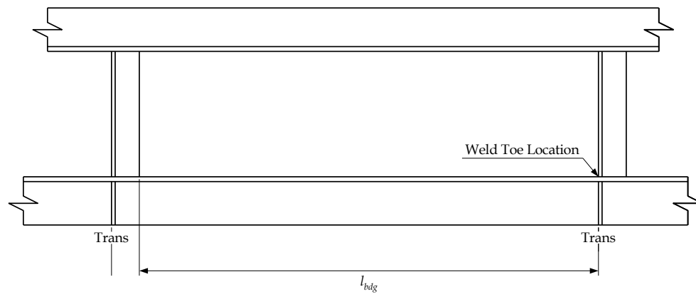
Supported by double skin / transverse bulkheads (1)
