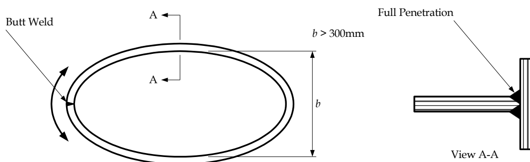
Fig. 6.5.5 Examples of Suitable Edge Reinforcements
