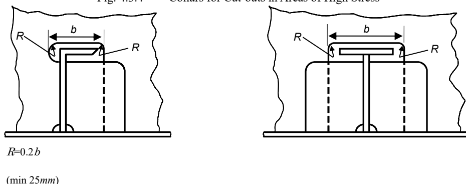
Fig. 4.3.4 Collars for Cut-outs in Areas of High Stress
