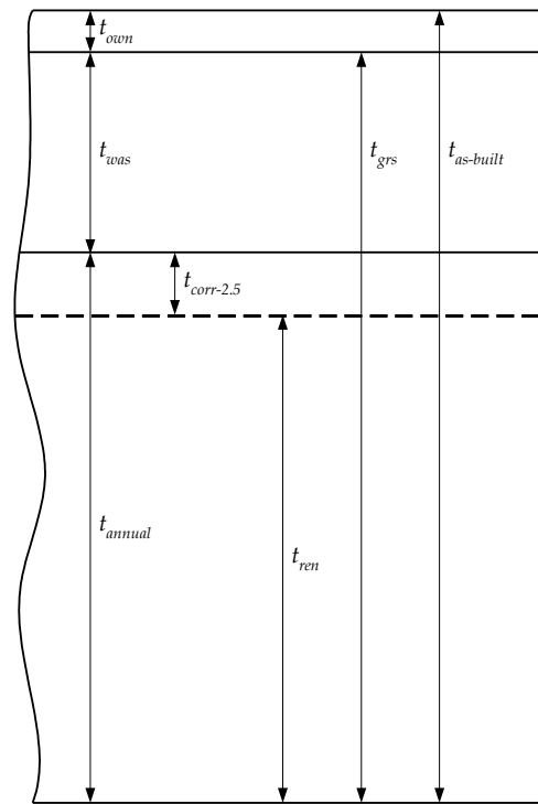
Fig. 2.4.1 Net Thickness Approach for Local Wastage
