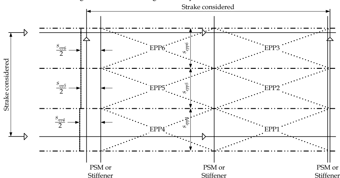
Fig. 3.5.2 Determining Elementary Plate Panels for a Strake
