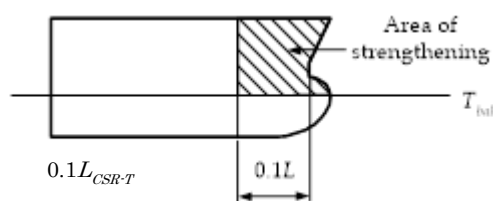
Fig. 8.6.6 Extent of Strengthening Against Bow Impact
