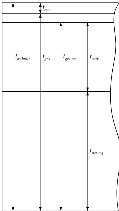
Fig. 2.4.1 Net Thickness Approach for Local Wastage
