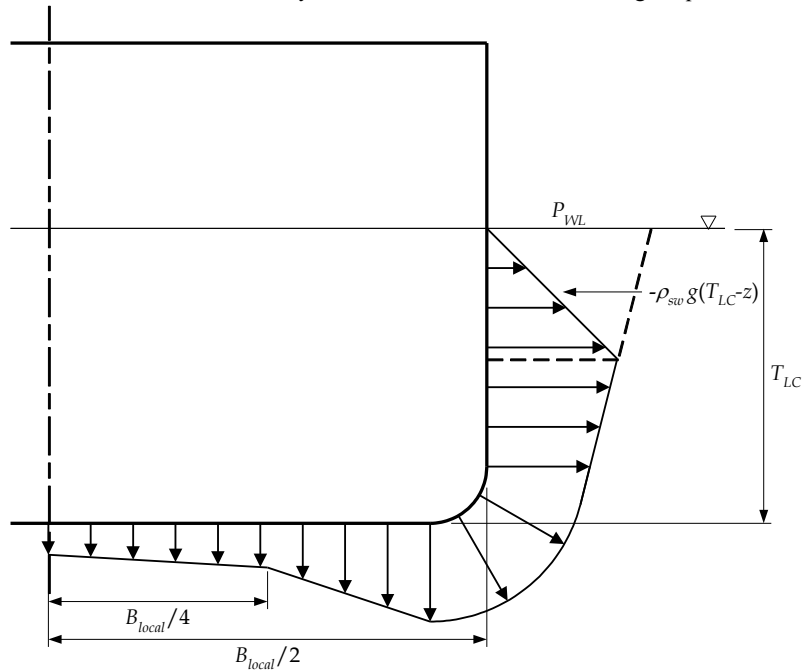
Fig. 7.3.6 Transverse Distribution of Minimum Dynamic Wave Pressure for Scantling Requirements and Strength Assessment
