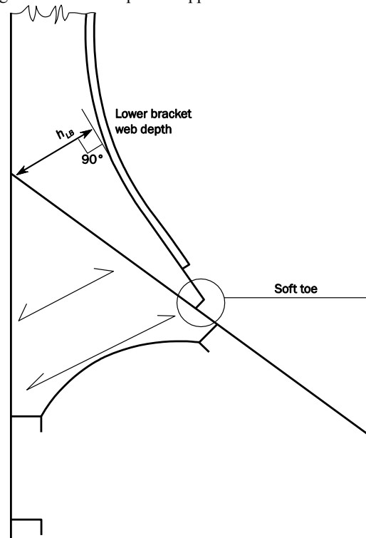
Fig. 5 Example of Support Structure for Lower End
