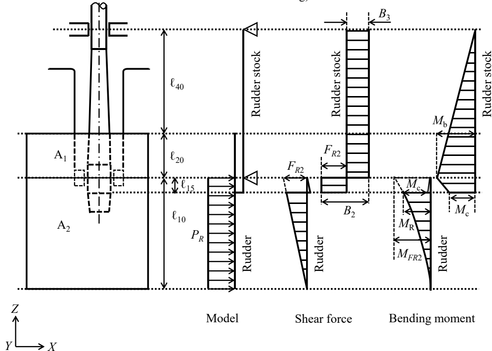
Fig. CS3.4.1-5 Type C Rudder with Rudder Trunk Supporting Rudder Stock (Pressure Applied only on Rudder Area below the Middle of Neck Bearing)
