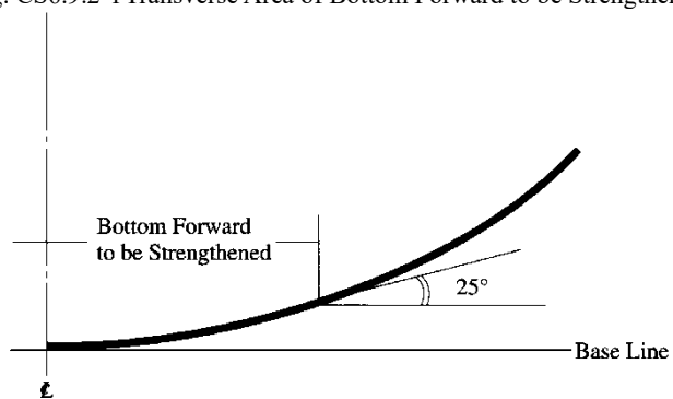
Fig. CS6.9.2-1 Transverse Area of Bottom Forward to be Strengthened
