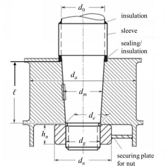
Fig. CS3.8 Cone Coupling with Key
