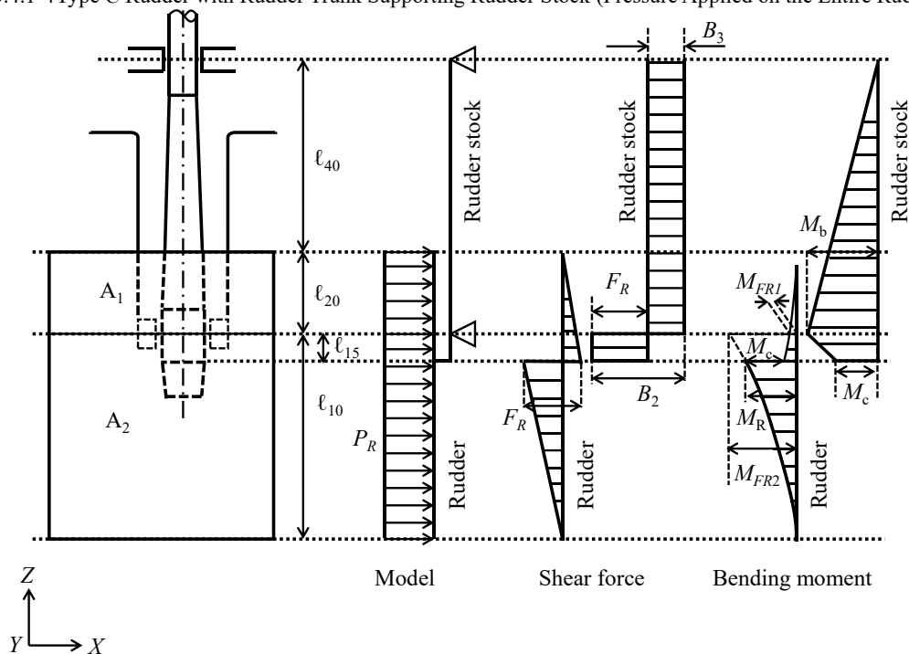
Fig. CS3.4.1-4 Type C Rudder with Rudder Trunk Supporting Rudder Stock (Pressure Applied on the Entire Rudder Area)
