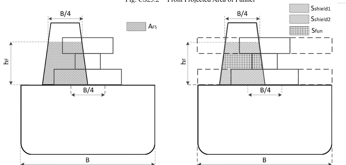
Fig. CS23.2 Front Projected Area of Funnel
