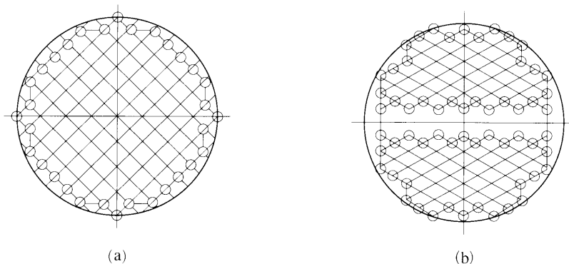
Fig. D10.2 Polygon used for Tube Plate Calculation
