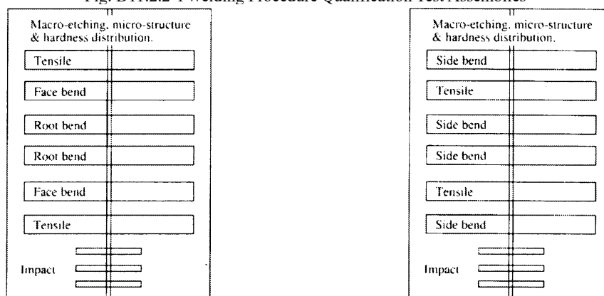
Fig. D11.2.2-1 Welding Procedure Qualification Test Assemblies
