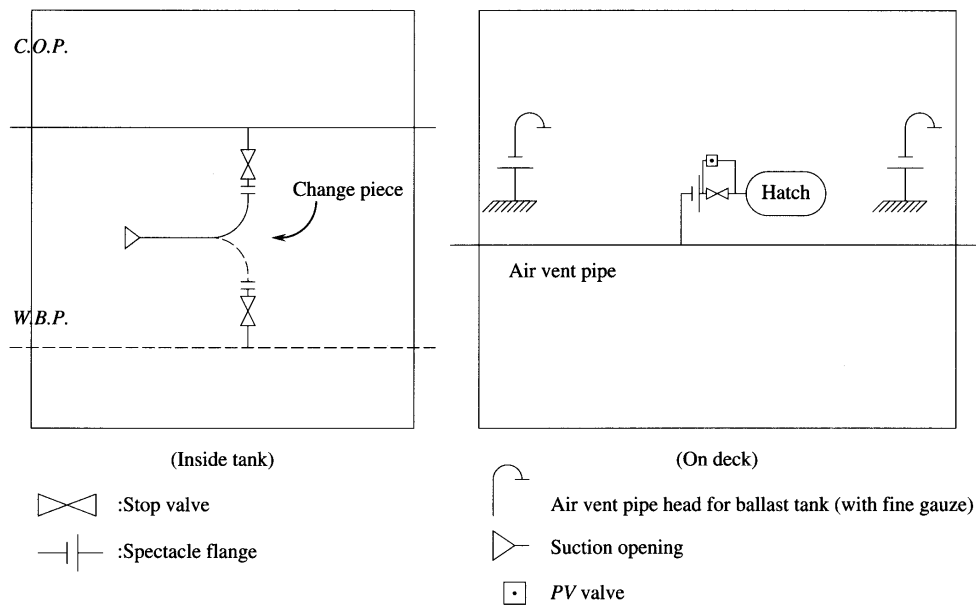
Fig. D14.2.3-2 Example of Piping Arrangements for Tanks Alternatively Used as Cargo Oil Tanks and Fuel Oil Tanks
