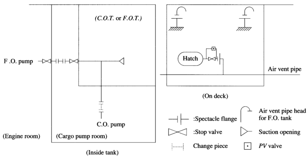
Fig. D14.2.3-2 Example of Piping Arrangements for Tanks Alternatively Used as Cargo Oil Tanks and Fuel Oil Tanks
