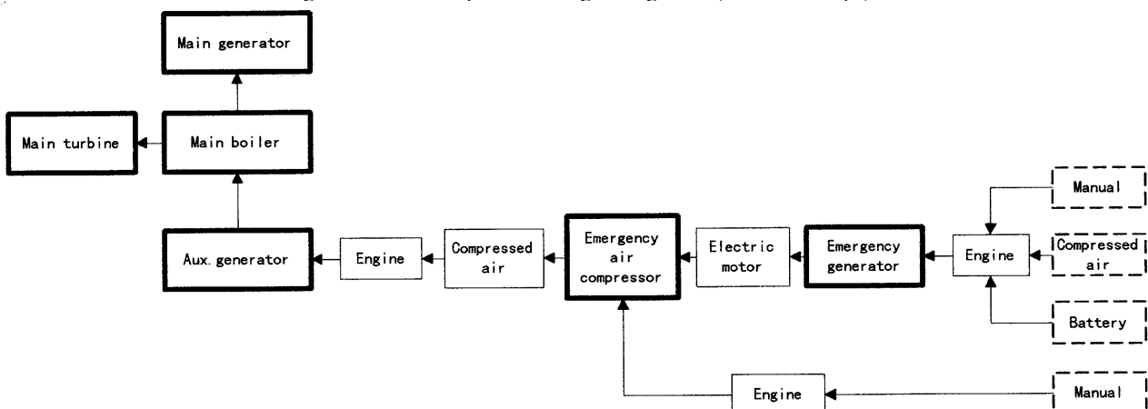
Fig. D1.3.1-3 Example of Starting Arrangement (for Steam Ships)
