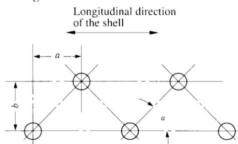
Fig. D9.2 Saw Tooth Pattern of Holes
