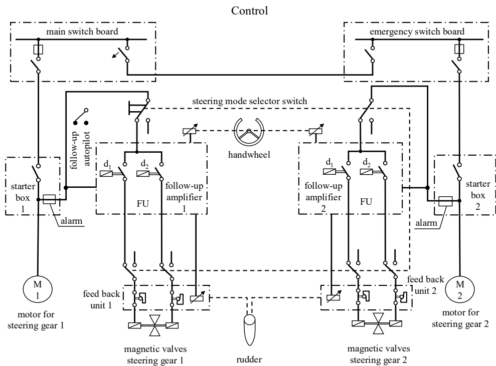
Fig. D15.3.1-2 Example Layout of Control Systems with Double Follow-up Control and Autopilot or Other Additional
