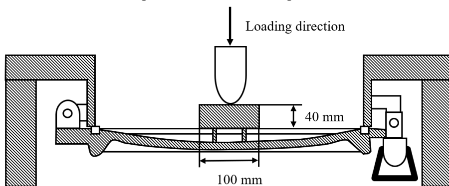
Fig. L7.1 Mechanical Strength Test
