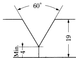
(a) Edge Preparation for Multi-run Technique
