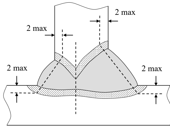
Fig. M4.9 Hardness Test (Unit: mm )
