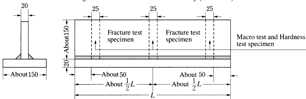
Fig. M6.3 Fillet Weld Test Assembly (Unit: mm)
