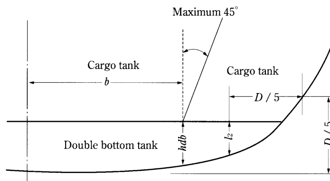
Fig. 3.3.2-10(5) Calculation of P_{As} of a Double Bottom Tank for which the Curvature of the Turn of Bilge Stake is Not Specified-when the Wing Tank is Cargo Tank
