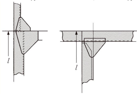
Fig. 4.8.1 Types of End Connection (Connection Type A)
