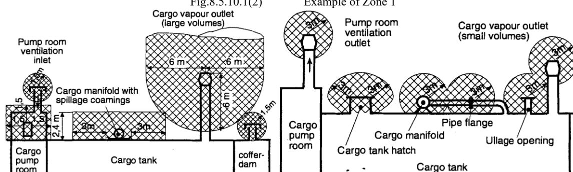
Fig.8.5.10.1(2) Example of Zone 1
