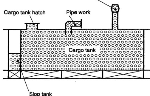
Fig.8.5.10.1(1) Example of Zone 0 Venting system
