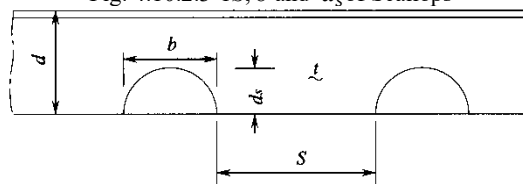
Fig. 4.10.2.3-1 S , b and d ς of Scallops
