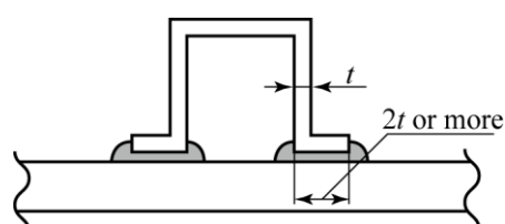
(c) Hat Shaped Structure Bonding
