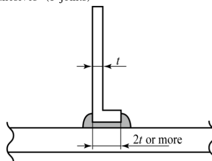
Fig. 5.5 Joints Using Structural Adhesives ( T -joints)
