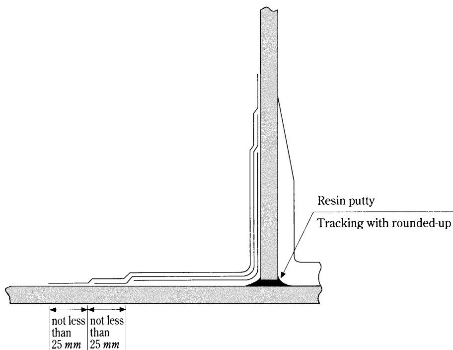
Fig. 5.3(b) In Case Chopped Mats are Used
