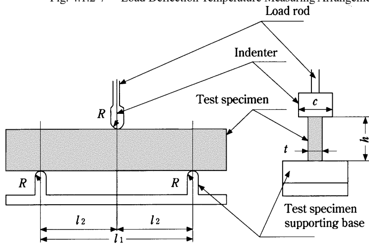
Fig. 4.1.2-7 Load Deflection Temperature Measuring Arrangement
