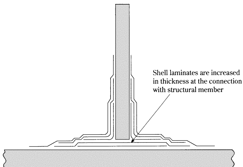
Fig. 5.4(a) In Case Consideration is to be Paid to Load or Vibration
