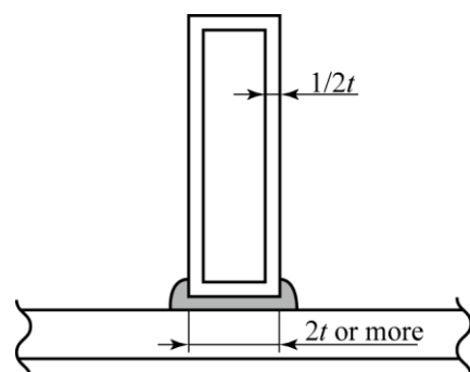
(b) Plywood Sandwich Bonding
