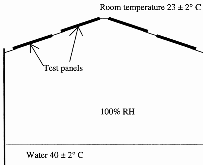
Figure 2 Condensation chamber
