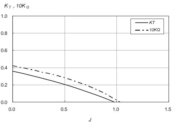
Figure 8: Propeller characteristics
