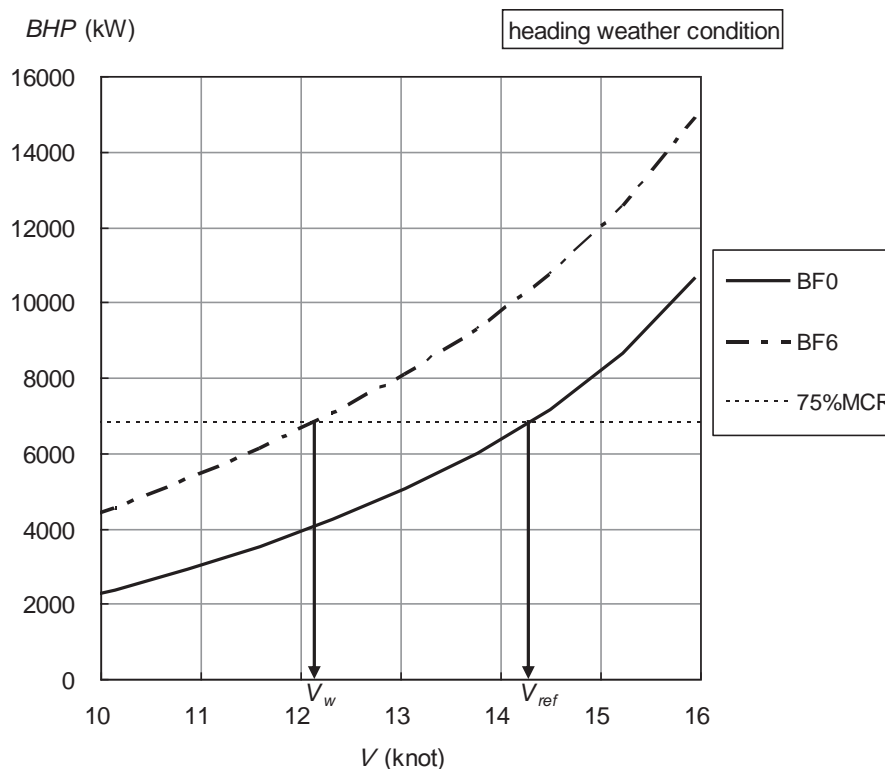
Figure 9: Power curves
