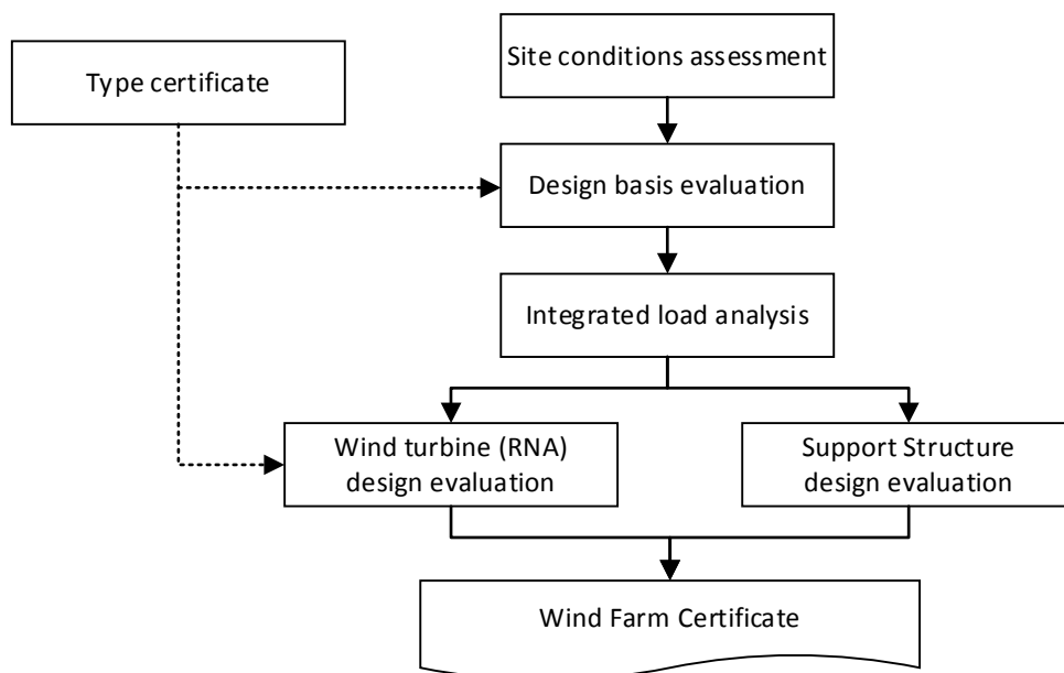
Fig. 1: Evaluation module for wind farm certification
