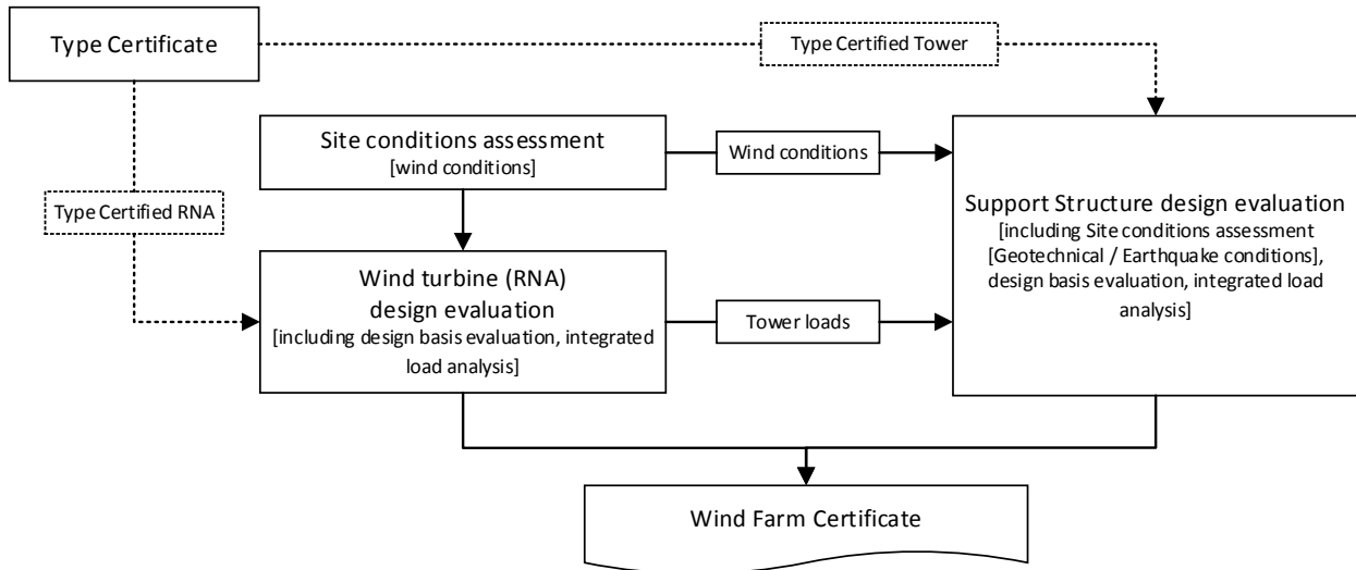
Fig. 2: Evaluation module for wind farm certification [in the case of onshore wind power plants]
