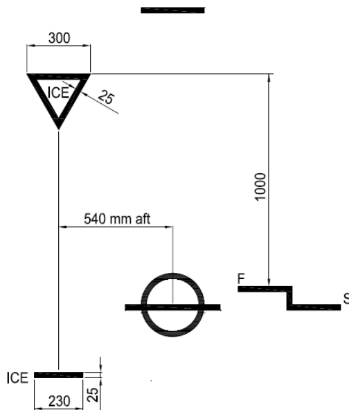
Fig. I8.1 Ice Class Draught Marking
