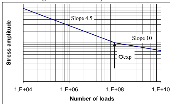
Fig. 18.11 Two-slope S-N Curve
