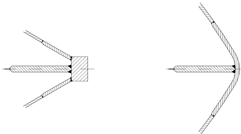
Fig. I8.3 Examples of Suitable Stems
