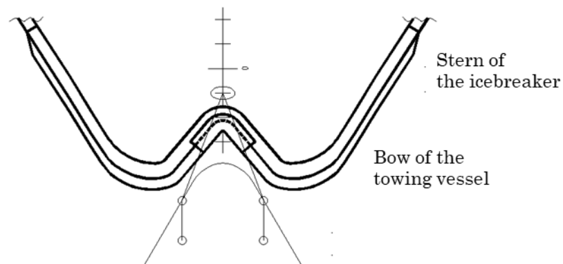
Fig. 18.3.8-1 The Typical Towing Arrangement
