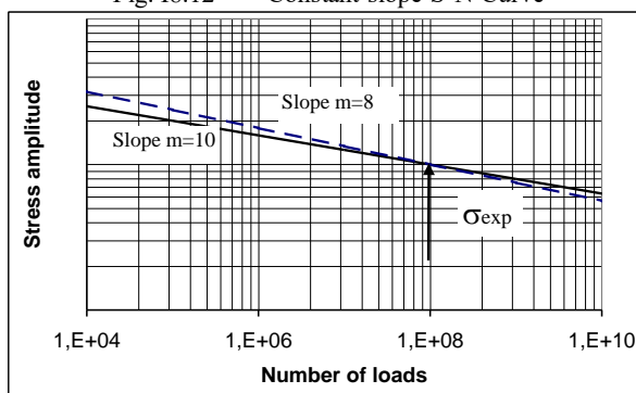
Fig. 18.12 Constant-slope S-N Curve
