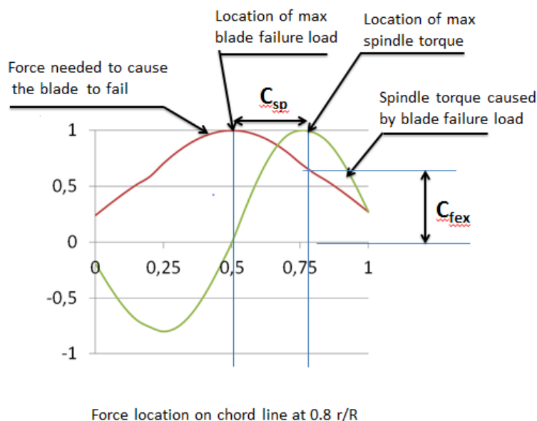
Fig. 18.10 Schematic figure showing a blade failure load and the related spindle torque when the force acts at a different location on the chord line at radius 0.8R
